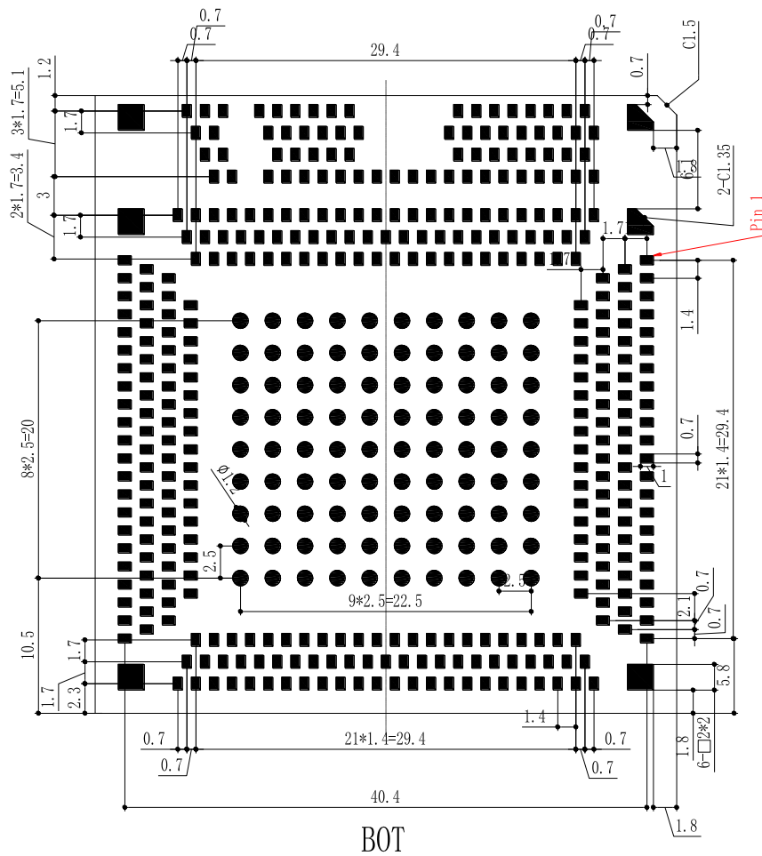
Figure 49: Module Bottom Dimensions (Bottom View, Unit: mm)
