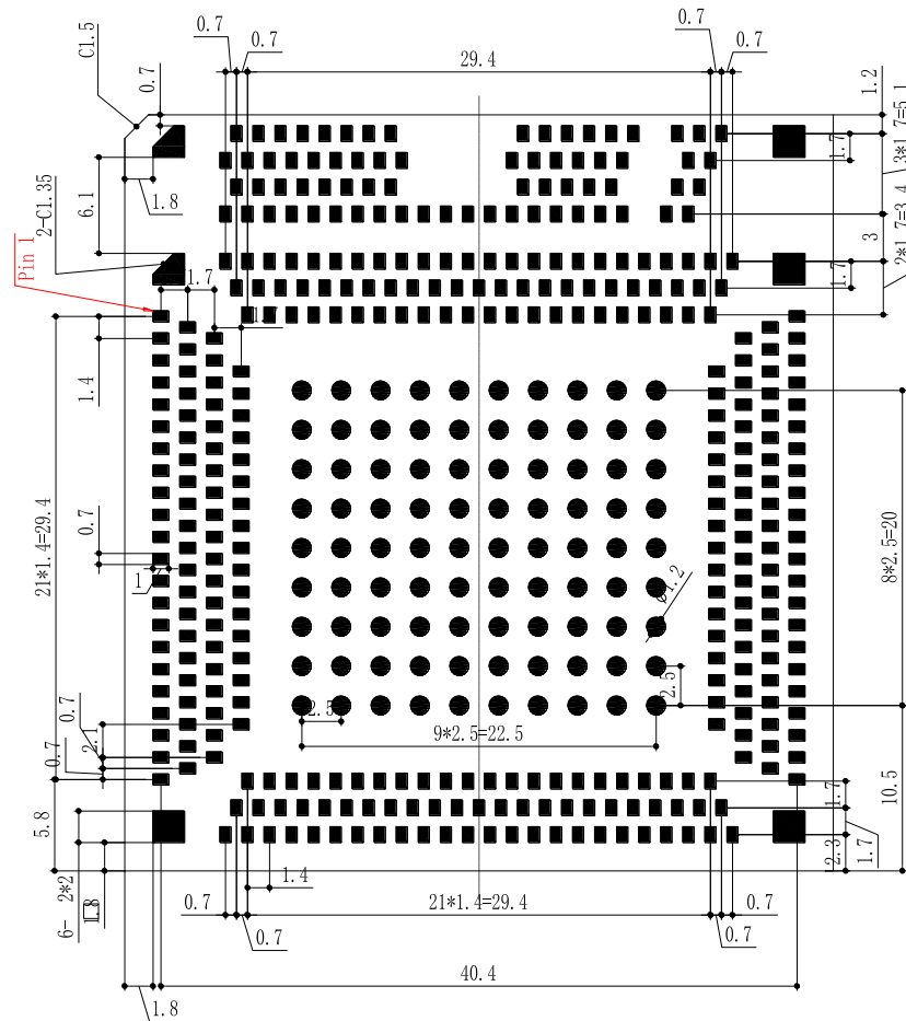
Figure 50: Recommended Footprint
