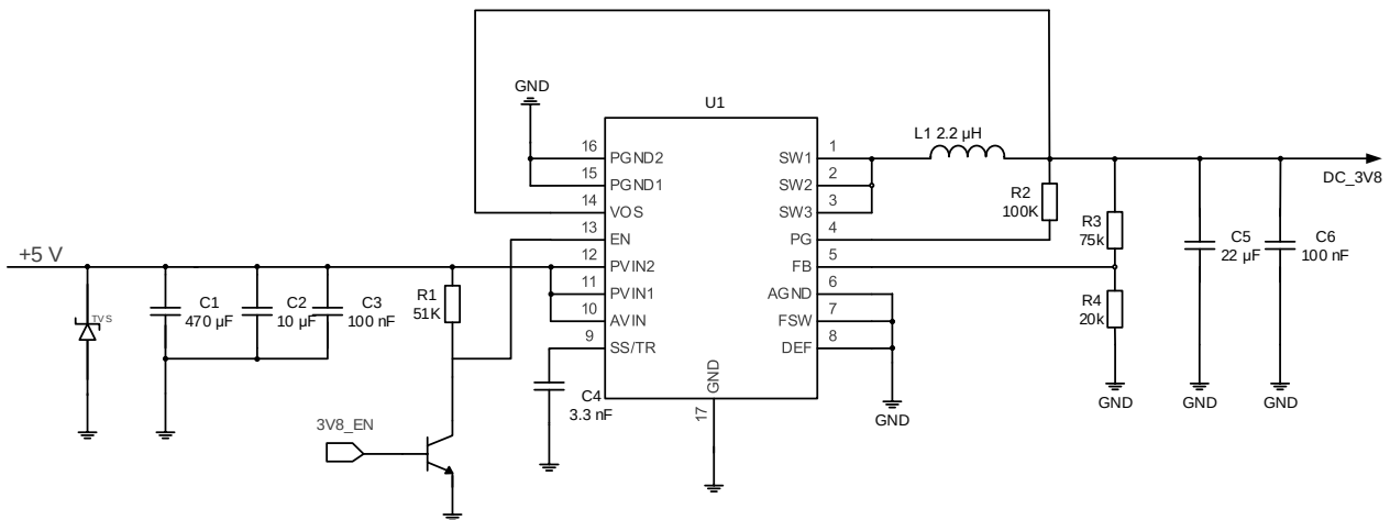
Figure 8: Reference Design of Power Supply
