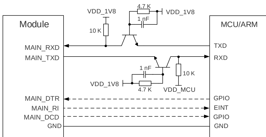
Figure 29: Reference Circuit with Transistor Circuit
