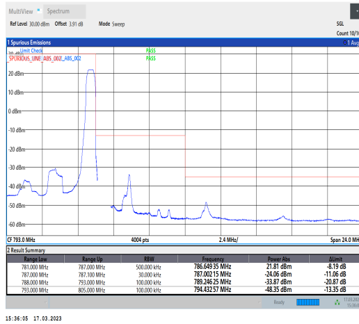
1-N13-PC3-15-5-H-2-DFT-PI2BPSK-Edge_1RB_Right-1@24-Ant1-1--PASS-see graph
