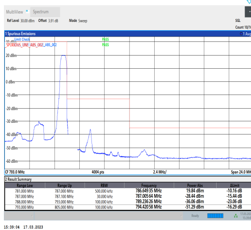
1-N13-PC3-15-5-H-5-CP-QPSK-Edge_1RB_Right-1@24-Ant1-1--PASS-see graph
