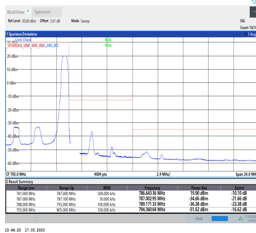
1-N13-PC3-15-10-H-5-CP-QPSK-Edge_1RB_Right-1 @51-Ant1-1--PASS-see graph
