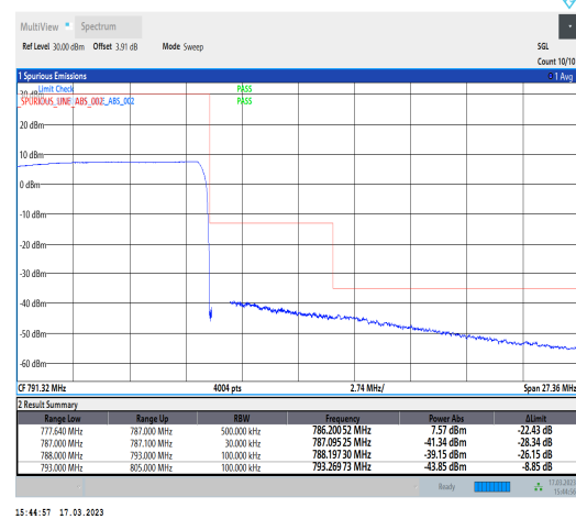
1-N13-PC3-15-10-H-6-CP-QPSK-Outer_Full-52@ 0-Ant1-1--PASS-see graph
