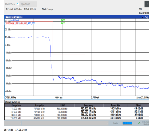
1-N13-PC3-15-10-H-3-DFT-PI2BPSK-Outer_Full-5 0@0-Ant1-1--PASS-see graph
