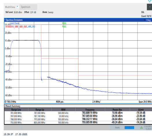
1-N13-PC3-15-5-H-6-CP-QPSK-Outer_Full-25@0-Ant1-1--PASS-see graph
