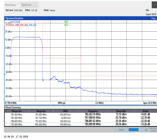
1-N13-PC3-15-5-H-3-DFT-PI2BPSK-Outer_Full-25@0-Ant1-1--PASS-see graph
