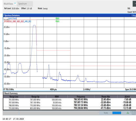
1-N13-PC3-15-10-H-2-DFT-PI2BPSK-Edge_1RB_Righ t-1@51-Ant1-1--PASS-see graph
