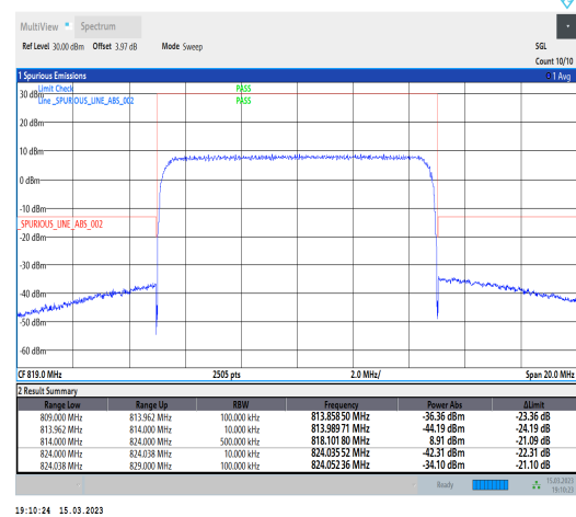
1-N26-814-824-PC3-15-10-L-6-CP-QPSK-Outer_F ull-52@0-Ant1-1--PASS-see graph
