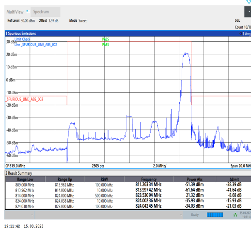
1-N26-814-824-PC3-15-10-H-5-CP-QPSK-Edge_1RB Right-1@51-Ant1-1--PASS-see graph
