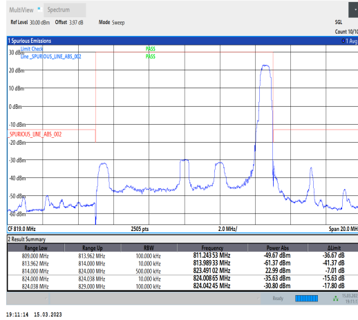
1-N26-814-824-PC3-15-10-H-2-DFT-PI2BPSK-Edge_1 RB_Right-1@51-Ant1-1--PASS-see graph
