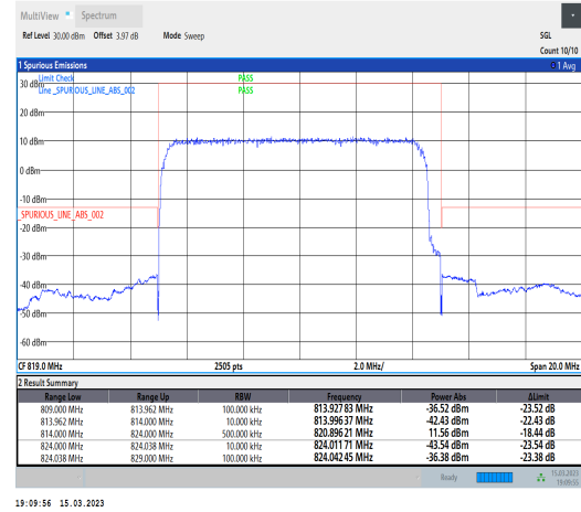
1-N26-814-824-PC3-15-10-L-3-DFT-PI2BPSK-Out er_Full-50@0-Ant1-1--PASS-see graph
