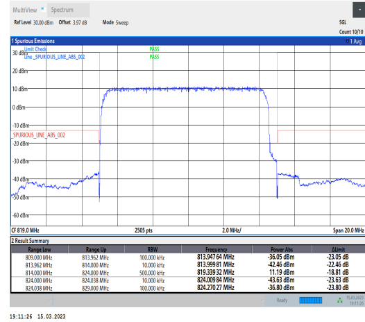
1-N26-814-824-PC3-15-10-H-3-DFT-PI2BPSK-Out er_Full-50@0-Ant1-1--PASS-see graph
