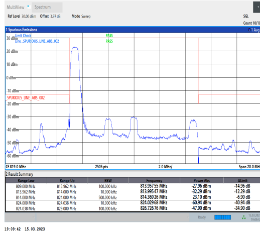
1-N26-814-824-PC3-15-10-L-1-DFT-PI2BPSK-Edge_1 RB_Left-1@0-Ant1-1--PASS-see graph
