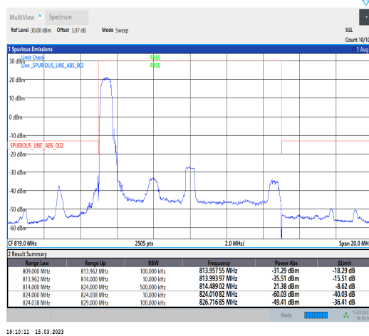
1-N26-814-824-PC3-15-10-L-4-CP-QPSK-Edge_1RB_ Left-1@0-Ant1-1--PASS-see graph
