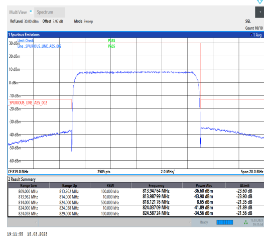
1-N26-814-824-PC3-15-10-H-6-CP-QPSK-Outer_ Full-52@0-Ant1-1--PASS-see graph
