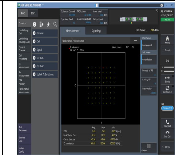
1-N13--15-10-M-8-CP-64QAM-Outer_Full-52@0-Ant1 t1-see graph-PASS
