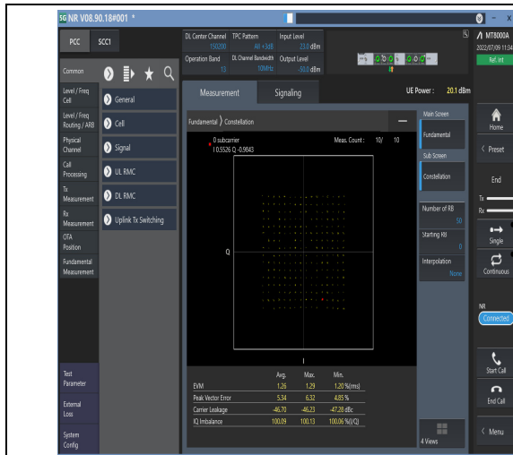
1-N13--15-10-M-5-DFT-256QAM-Outer_Full-50@0-A nt1-see graph-PASS
