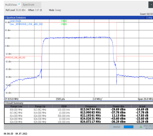
1-N26-814-824--15-10-M-3-DFT-PI2BPSK-Outer_ Full-50@0-Ant1-PASS-see graph
