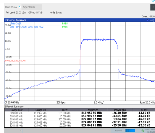
1-N26-814-824--15-5-H-6-CP-QPSK-Outer_Full-2 5@0-Ant1-PASS-see graph
