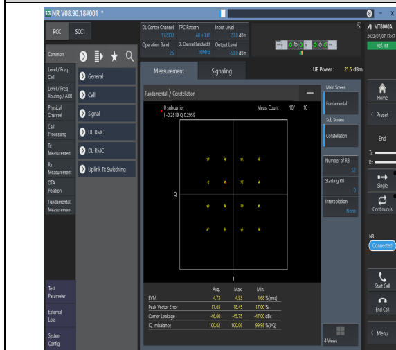
1-N26-814-824--15-10-M-7-CP-16QAM-Outer_Full-52@0-Ant1-see graph-PASS
