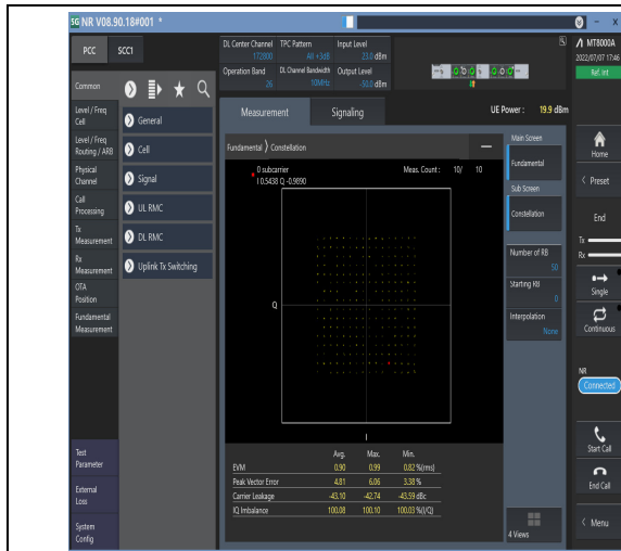
1-N26-814-824--15-10-M-5-DFT-256QAM-Outer_Full-50@0-Ant1-see graph-PASS
