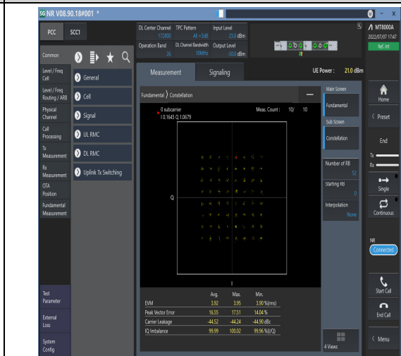
1-N26-814-824--15-10-M-8-CP-64QAM-Outer_Full-52@0-Ant1-see graph-PASS
