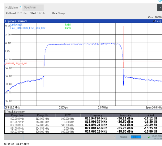
1-N26-814-824--15-10-M-6-CP-QPSK-Outer_Full- 52@0-Ant1-PASS-see graph
