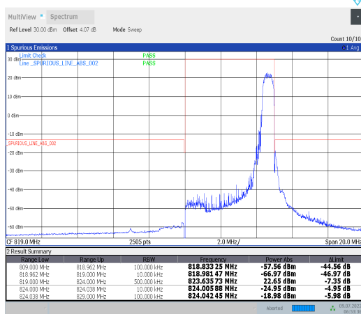
1-N26-814-824--15-5-H-5-CP-QPSK-Edge_1RB_Right- 1@24-Ant1-PASS-see graph
