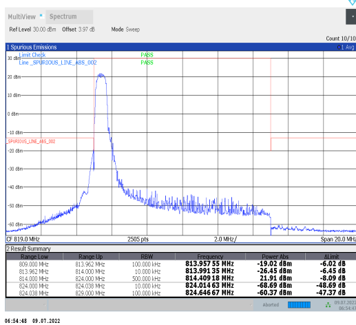
1-N26-814-824--15-10-M-4-CP-QPSK-Edge_1RB_Left- 1@0-Ant1-PASS-see graph
