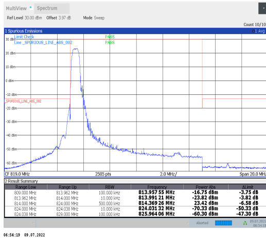
1-N26-814-824--15-10-M-1-DFT-PI2BPSK-Edge_1RB_ Left-1@0-Ant1-PASS-see graph
