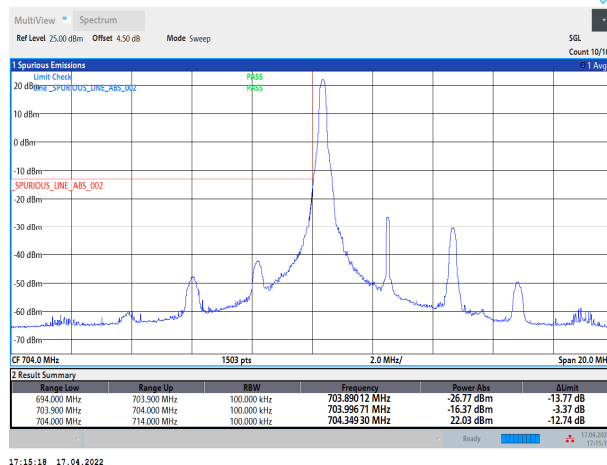
Band17-5MHz-QPSK-23755-25RB#0
