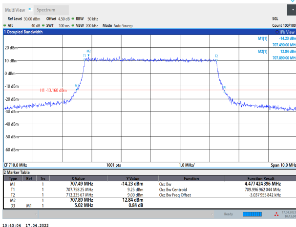
Band17-5MHz-QPSK-23790-25RB#0
