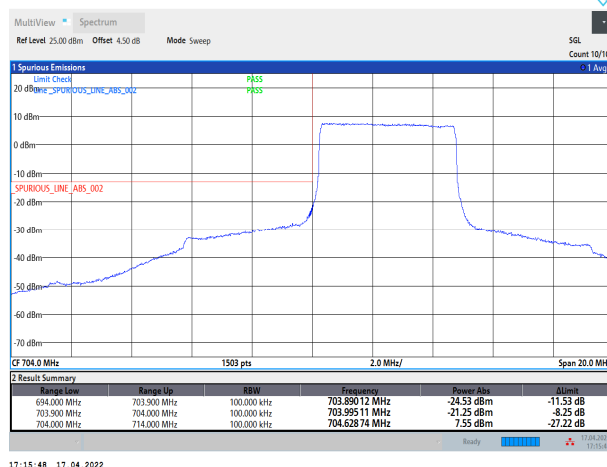
Band17-5MHz-QPSK-23755-25RB#0
