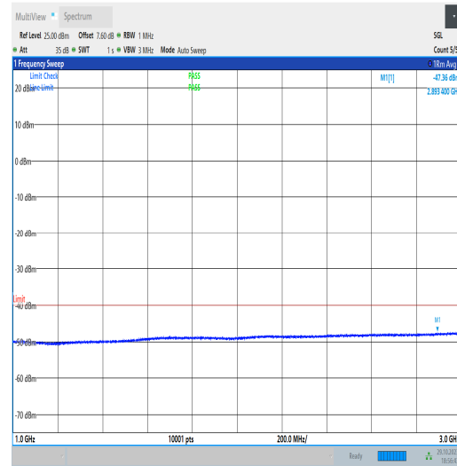
NTNV_N48_PC3_30_30_M_TID1_NS_01_1000_3000_#1
