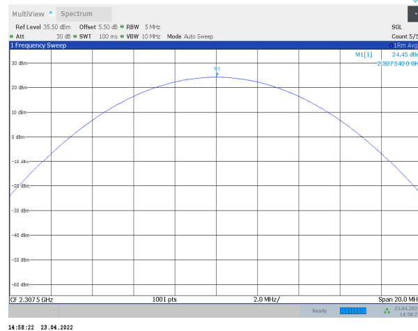
Band30-5MHz-QPSK-27685-1RB#12
