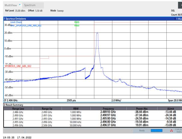
Band41-5MHz-QPSK-39675-25RB#0
