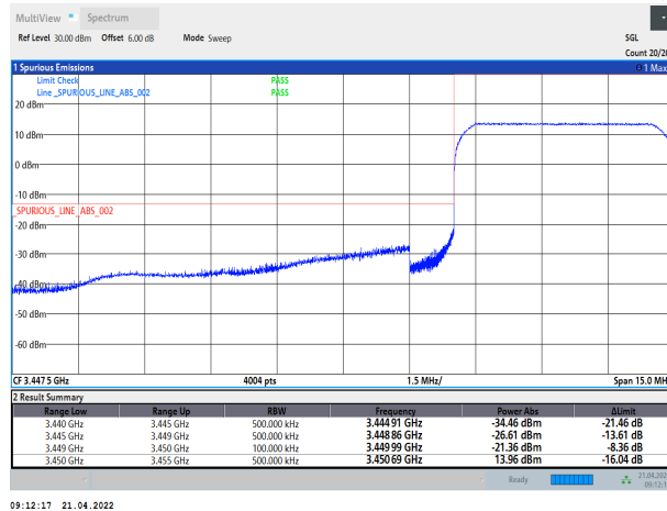
Band42-5MHz-QPSK-42115-25RB#0
