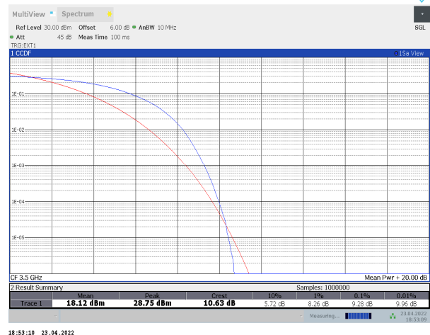
Band42-20MHz-QPSK-42590-100RB#0
