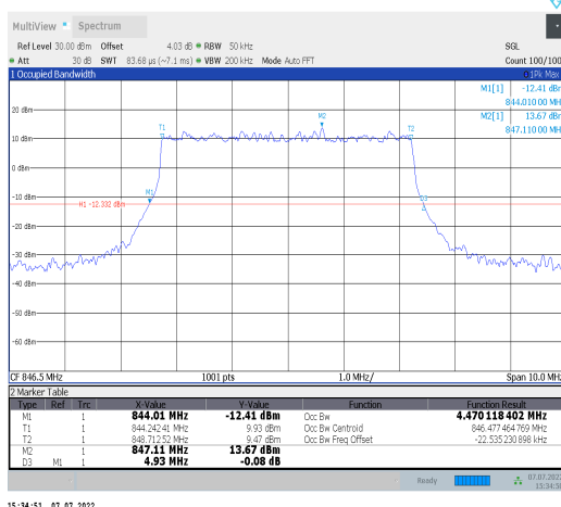
1-N26-824-849--15-5-H-1-DFT-QPSK-Outer_Full-25 @0-Ant0-4.47-4.930-<math>\leq</math>5-PASS
