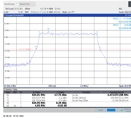
1-N26-824-849--15-5-M-9-CP-256QAM-Outer_Full-2 5@0-Ant0-4.473-4.950-<math>\leq</math>5-PASS
