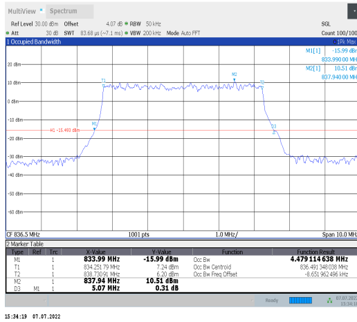
1-N26-824-849--15-5-M-8-CP-64QAM-Outer_Full-25 @0-Ant0-4.479-5.070-<math>\leq</math>5-PASS
