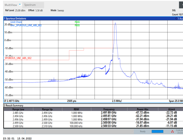
Band7-5MHz-QPSK-20775-25RB#0
