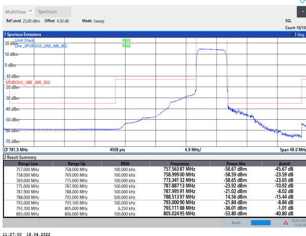
Band14-5MHz-QPSK-23305-25RB#0
