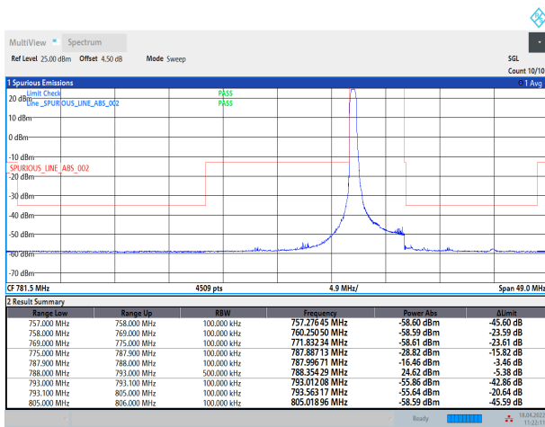
Band14-5MHz-QPSK-23305-1RB#0
