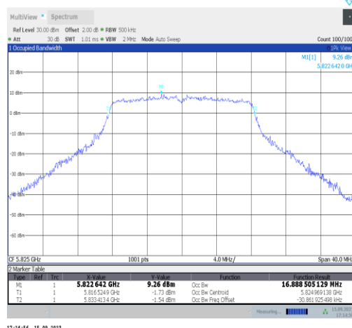
11a-Ant1-5825
