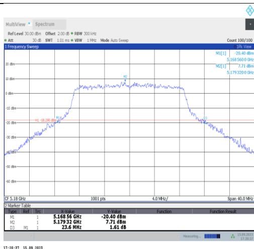
11n20SISO-Ant1-5180
