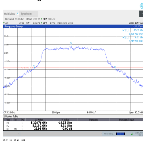
11n20SISO-Ant1-5220
