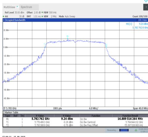
11a-Ant1-5785
