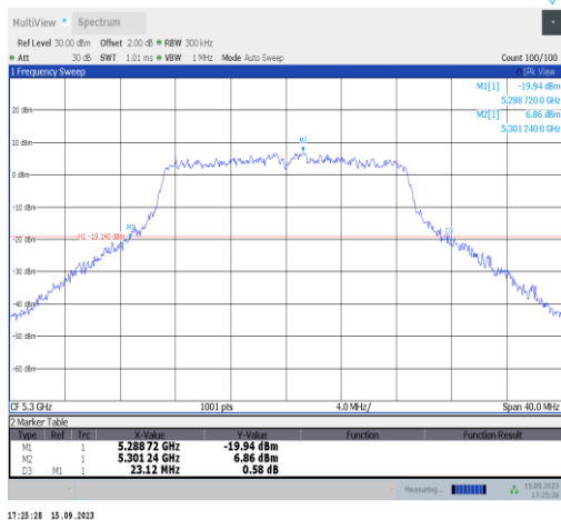
11n20SISO-Ant1-5300
