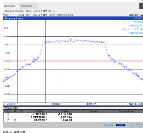
11n20SISO-Ant1-5320
