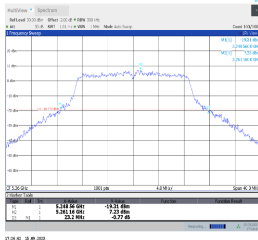
11n20SISO-Ant1-5260
