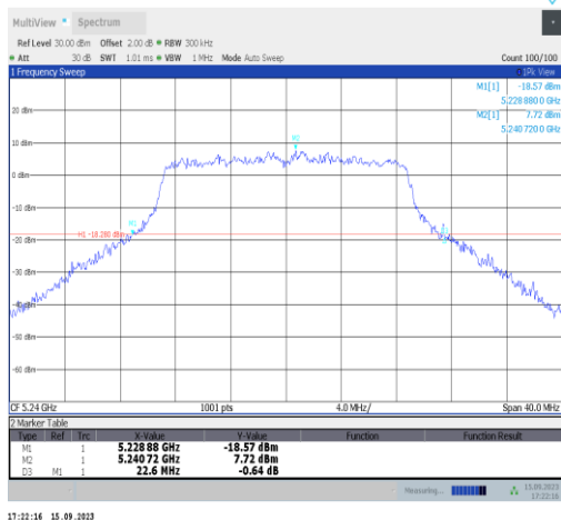
11n20SISO-Ant1-5240
