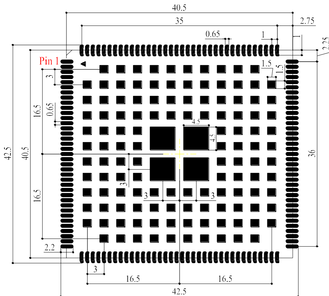
Figure 42: Recommended Footprint
