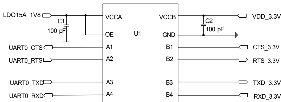
Figure 13: Reference Circuit with Level-shifting Chip for UART0
