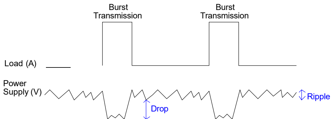
Figure 3: Power Supply Limits During Burst Transmission
