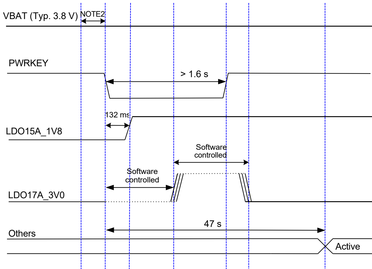
Figure 8: Turn-on Timing
