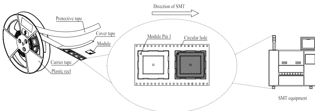
Figure 48: Mounting Direction
