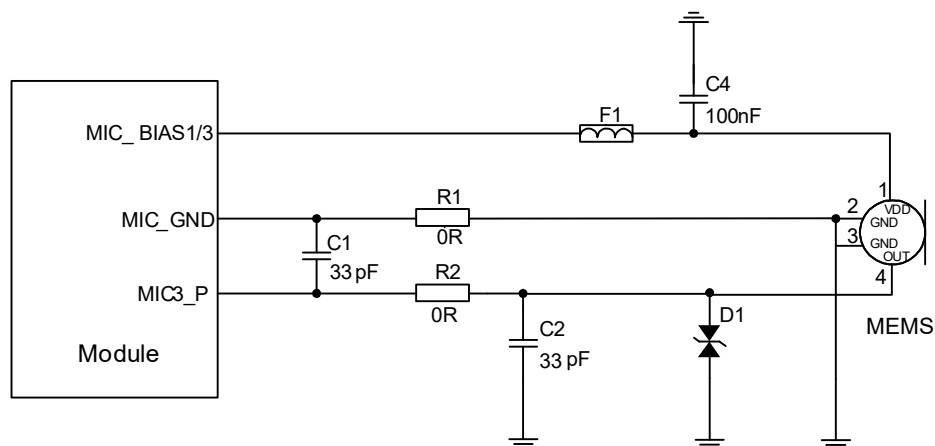
Figure 24: Reference Design for MEMS Microphone Interface
