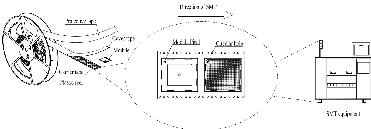
Figure 47: Mounting Direction
