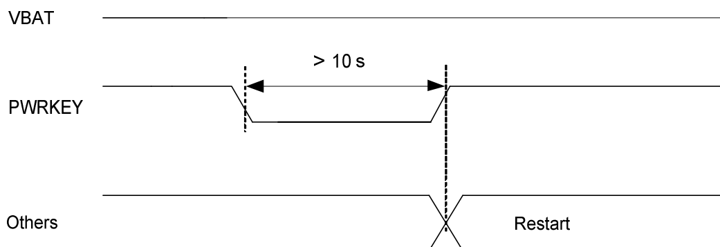
Figure 9: Power-down Timing
