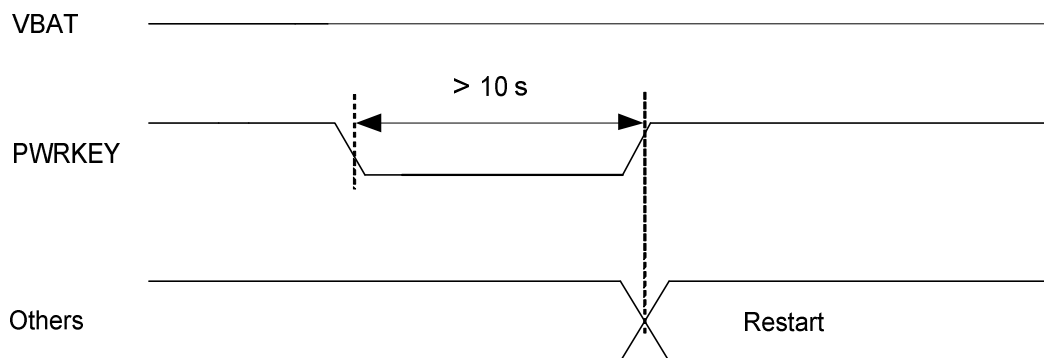
Figure 9: Power-down Timing
