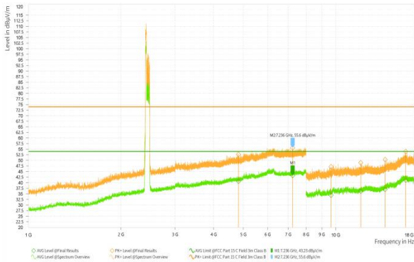
Wi-Fi 2.4_11AX20_2462_High
