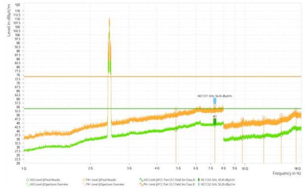
Wi-Fi 2.4_11AX40_2422_High
