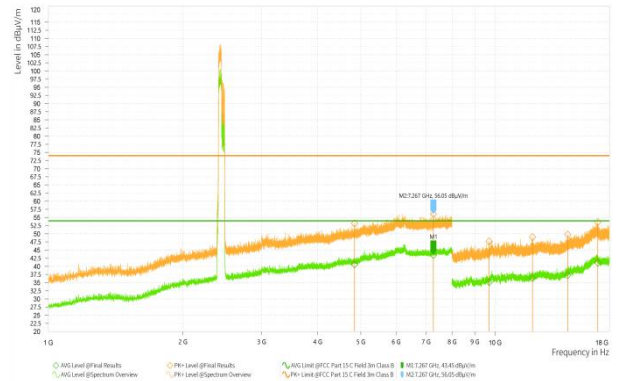
Wi-Fi 2.4_11AX40_2452_High
