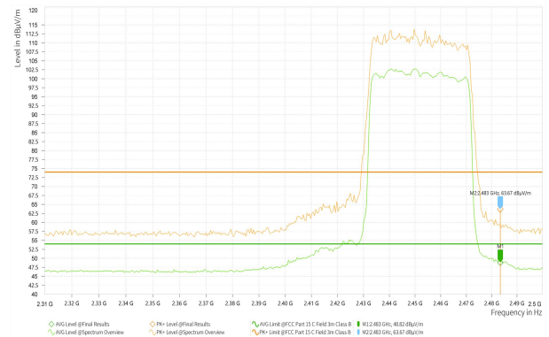
Wi-Fi 2.4_11AX40_2452_edge
