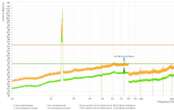
Wi-Fi 2.4_11AX40_2437_High
