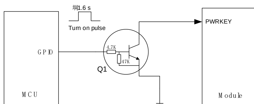
Figure 6: Turn On the Module Using Driving Circuit
