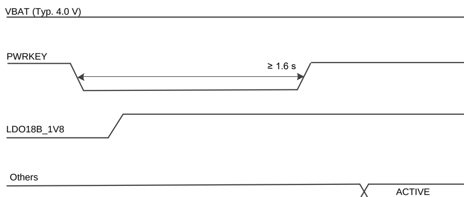
Figure 8: Turn-on Timing
