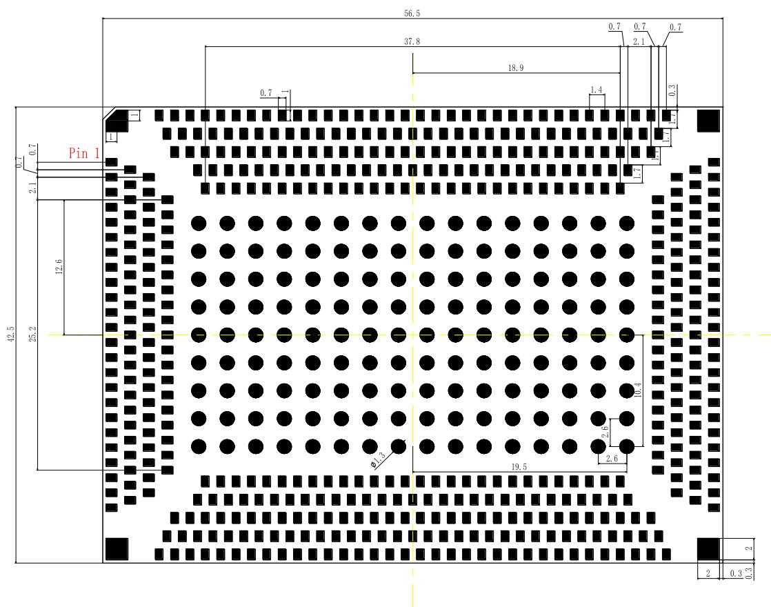
Figure 40: Recommended Footprint
