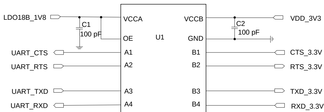
Figure 18: Reference Circuit with Level-Shifting Chip (for UART)
