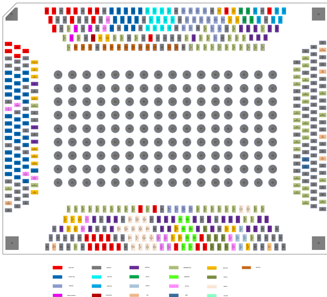
Figure 1: Pin Assignment
