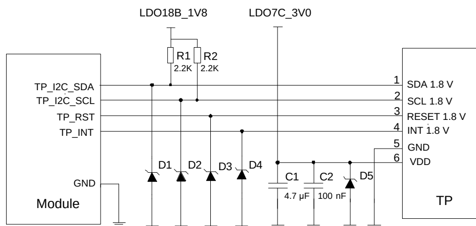
Figure 22: Reference Circuit for TP Interface
