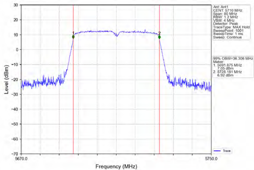
802.11n(HT40)_HCH_5710MHz_Ant1_NTN
