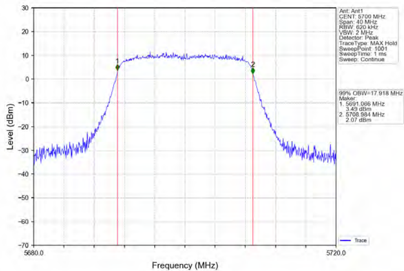
802.11n(HT20)_HCH_5700MHz_Ant1_NTN
