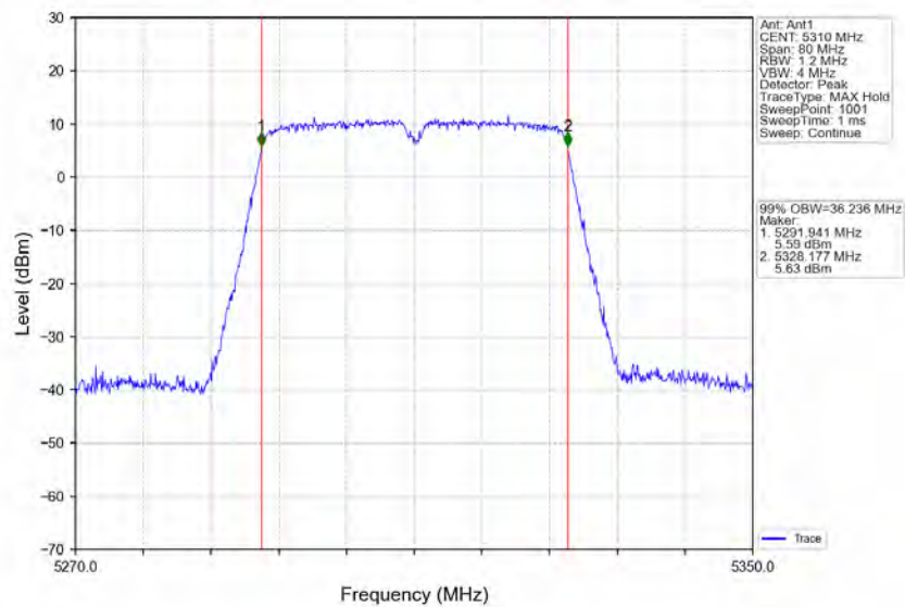
802.11n(HT40)_HCH_5310MHz_Ant1_NTN
