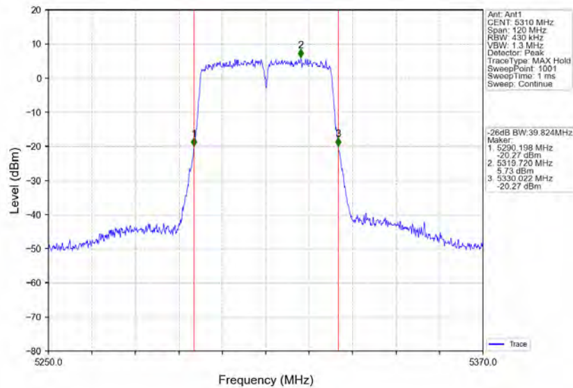
802.11n(HT40)_HCH_5310MHz_Ant1_NTN
