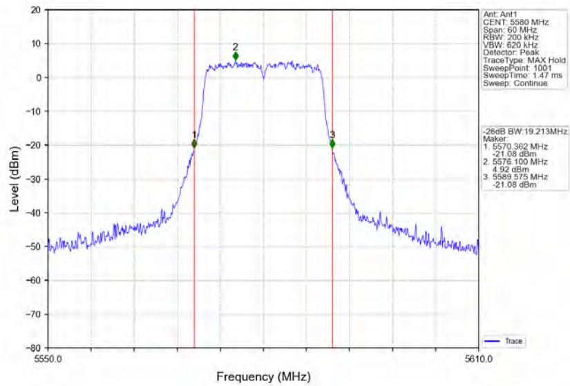
802.11a_MCH_5580MHz_Ant1_NTV
