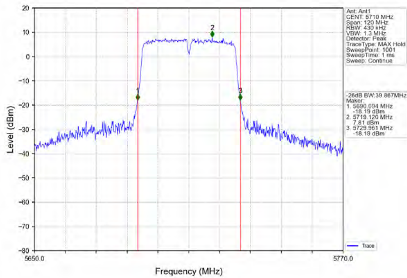
802.11n(HT40)_HCH_5710MHz_Ant1_NTN
