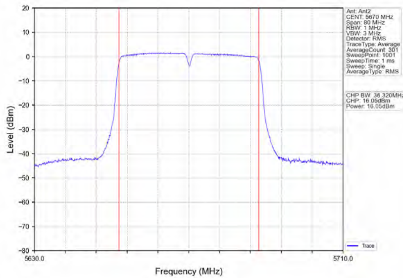
802.11n(HT40)_HCH_5670MHz_Ant2_NTN
