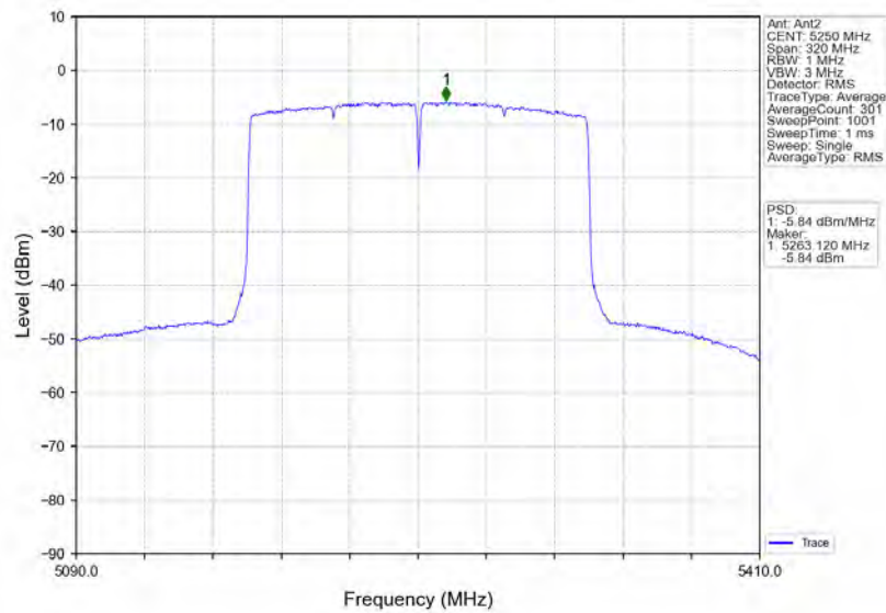
802.11ax(HEW160) MCH 5250MHz 2xRU996 Left MIMO NTN
