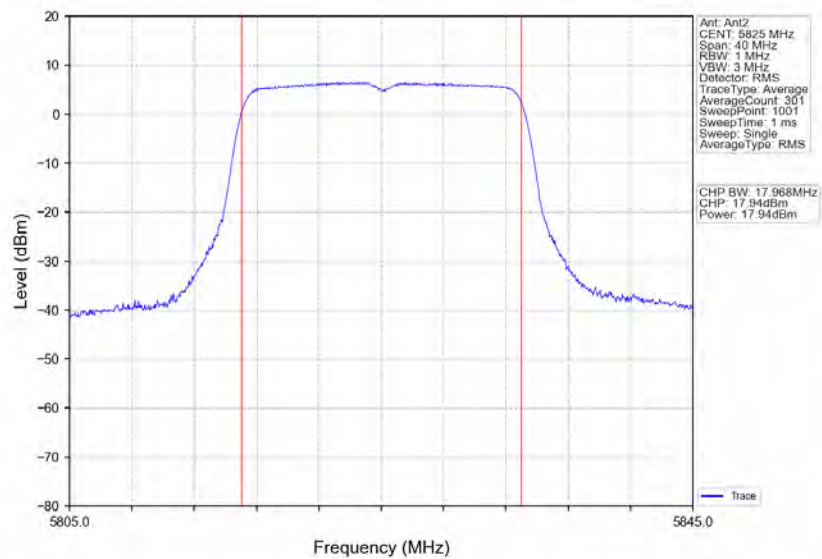
802.11n(HT20)_HCH_5825MHz_Ant2_NTN
