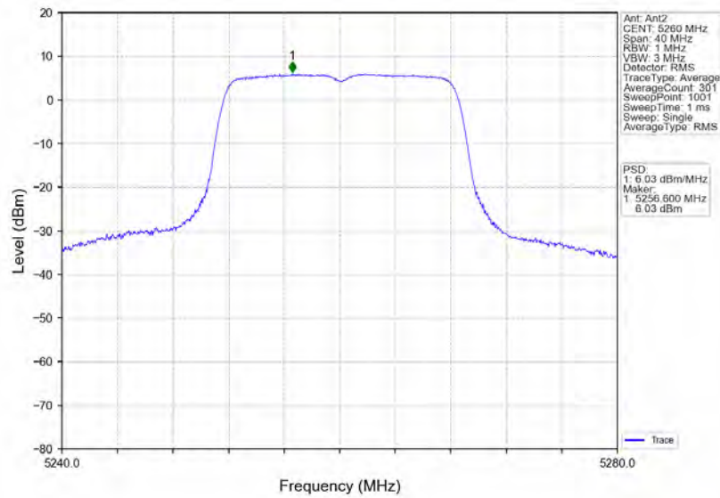
802.11a_LCH_5260MHz_Ant2_NTNV
