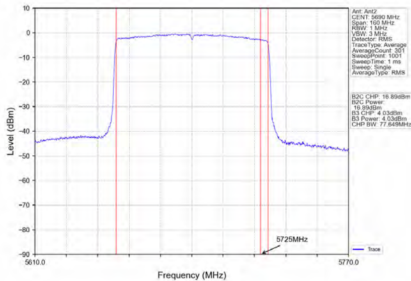
802.11ax(HEW80) HCH 5690MHz RU996 Left Ant2 NTNv
