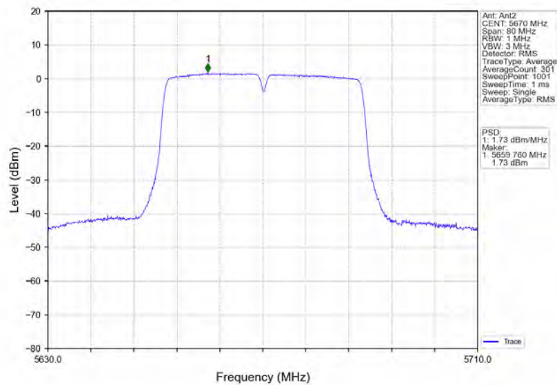
802.11n(HT40)_HCH_5670MHz_Ant2_NTN
