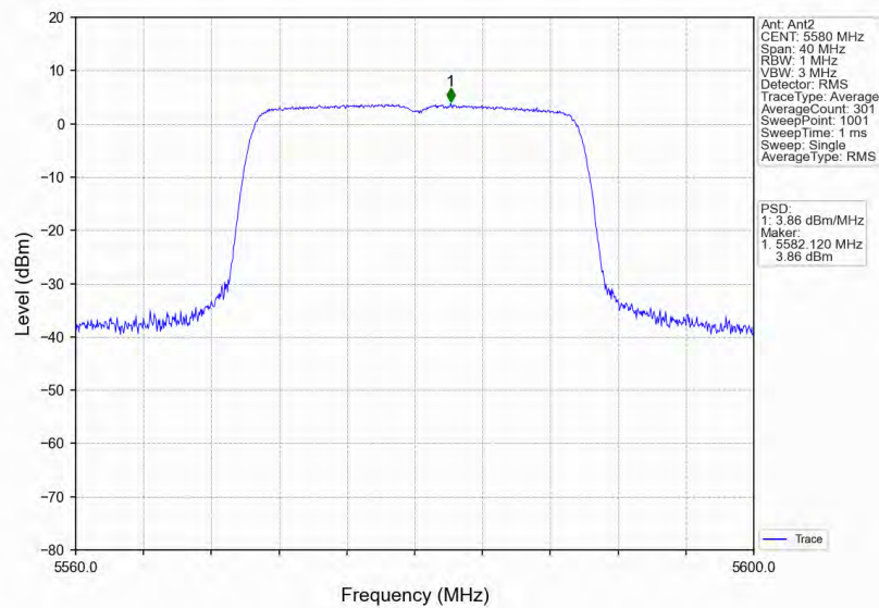
802.11ax(HEW20) MCH 5580MHz RU242 Left Ant2 NTN
