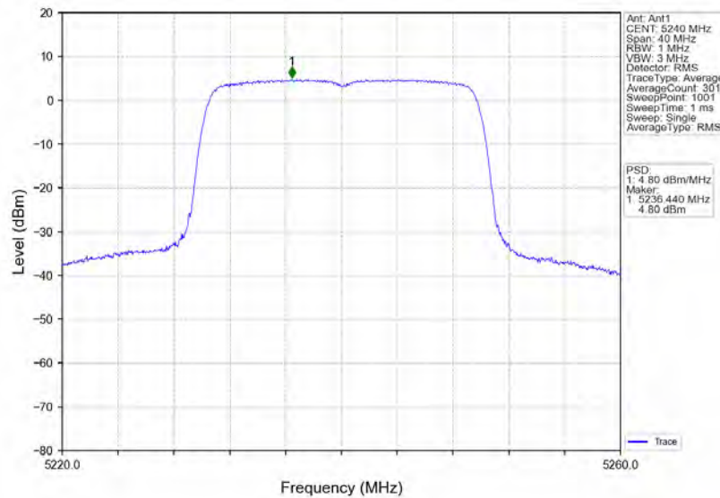
802.11ax(HEW20) HCH 5240MHz RU242 Left Ant1 NTN
