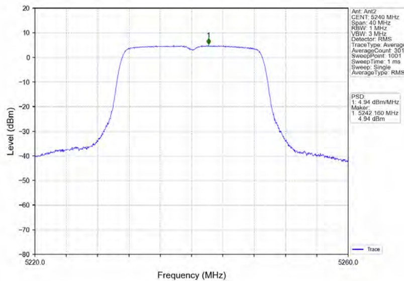
802.11n(HT20)_HCH_5240MHz_Ant2_NTN
