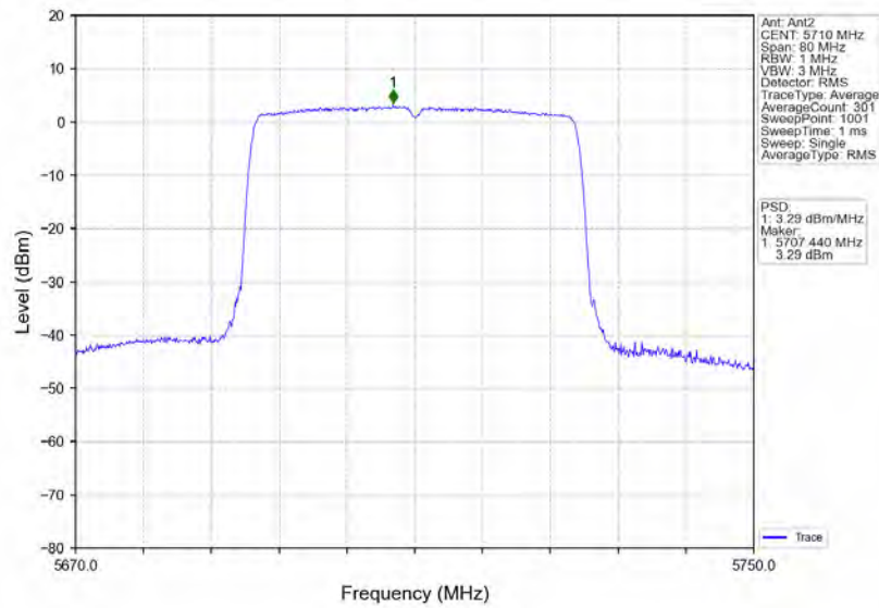
802.11ax(HEW40) HCH 5710MHz RU484 Left Ant2 NTN
