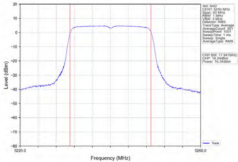
802.11n(HT20)_HCH_5240MHz_Ant2_NTN
