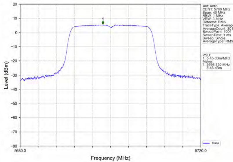
802.11n(HT20)_HCH_5700MHz_Ant2_NTN
