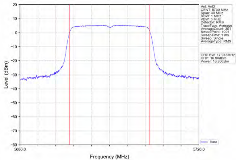
802.11n(HT20)_HCH_5700MHz_Ant2_NTN
