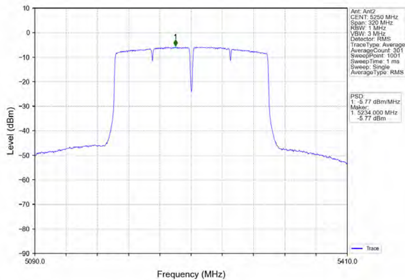
802.11ac(VHT160) MCH_5250MHz_Ant2_NTNV
