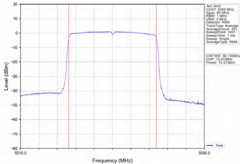
802.11ax(HEW40) MCH 5550MHz RU484 Left Ant2 NTN
