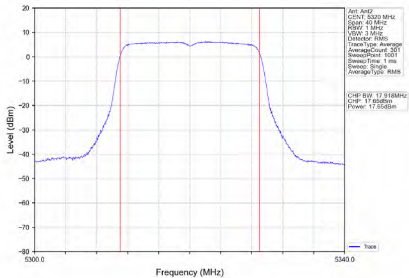
802.11n(HT20)_HCH_5320MHz_Ant2_NTN
