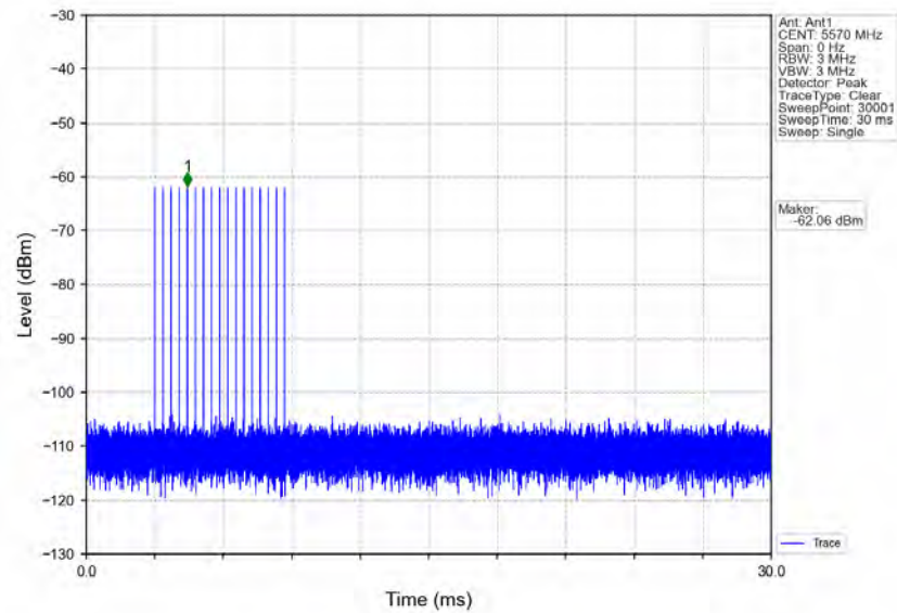
Signal Calibration 802.11ax(HEW160) 2C 5570MHz RadarType4 Trial0
