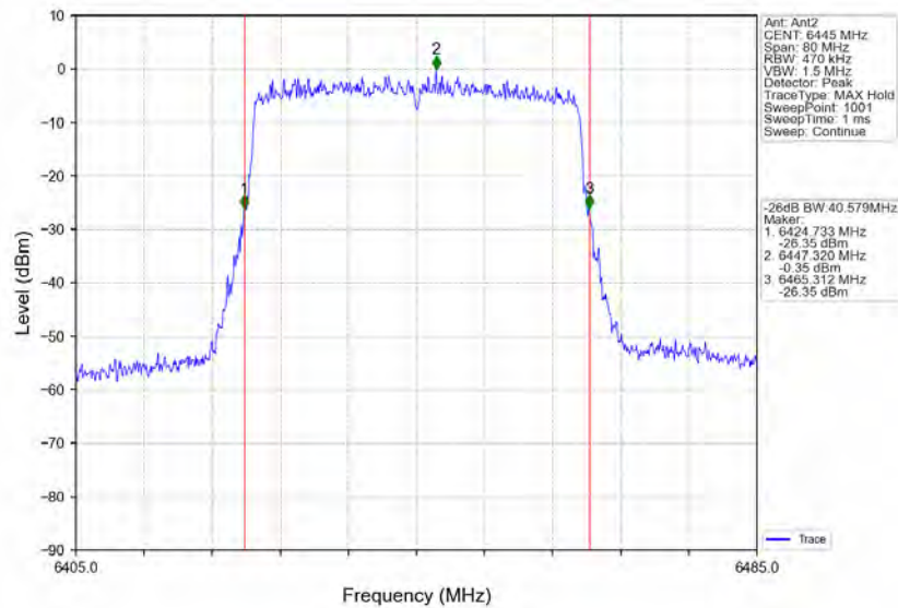
802.11ax(HEW40)_LCH_6445MHz_RU484_Left_Ant2_NTNV
