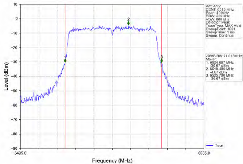
802.11ax(HEW20)_HCH_6515MHz_RU242_Left_Ant2_NTNV
