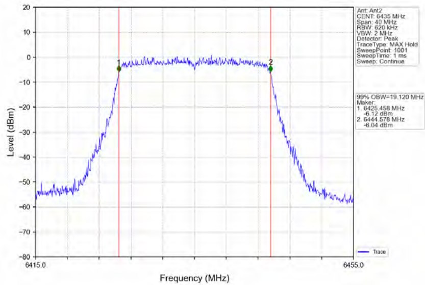
802.11ax(HEW20)_LCH_6435MHz_RU242_Left_Ant2_NTNV
