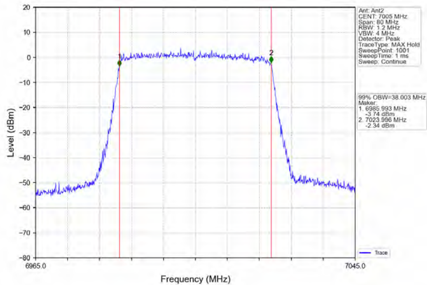
802.11ax(HEW40)_MCH_7005MHz_RU484_Left_Ant2_NTNV
