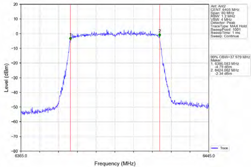
802.11ax(HEW40)_HCH_6405MHz_RU484_Left_Ant2_NTNV
