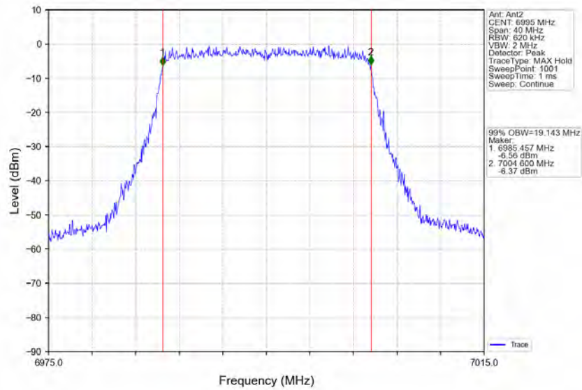
802.11ax(HEW20)_MCH_6995MHz_RU242_Left_Ant2_NTNV
