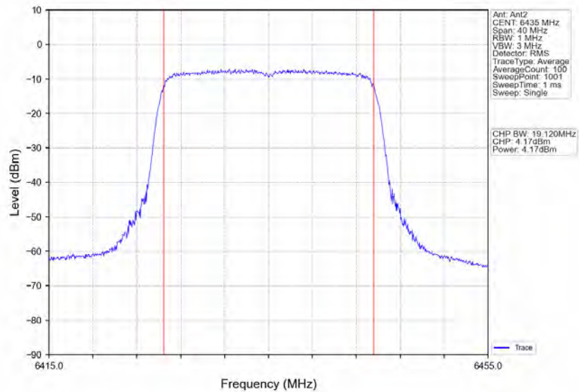
802.11ax(HEW20)_LCH_6435MHz_RU242_Left_Ant2_NTNV
