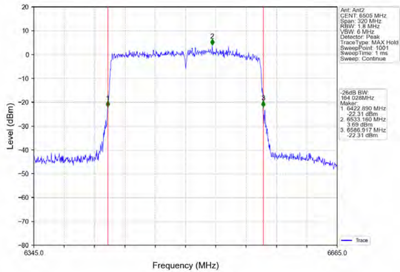
802.11ax(HEW160)_HCH_6505MHz_2xRU996_Left_Ant2_NTNV
