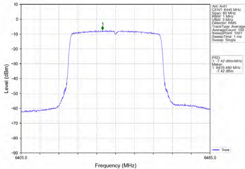
802.11ax(HEW40)_LCH_6445MHz_RU484_Left_Ant1_NTNV
