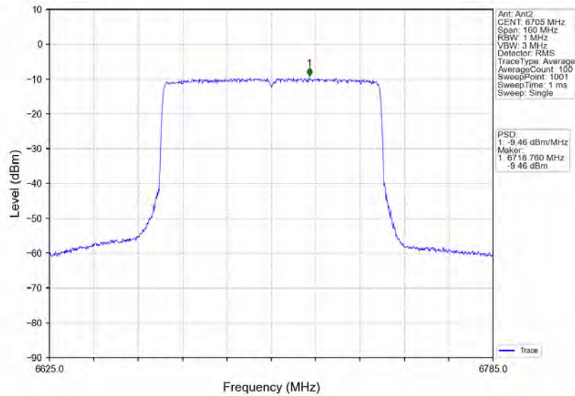
802.11ax(HEW80)_MCH_6705MHz_RU996_Left_MIMO_NTNV
