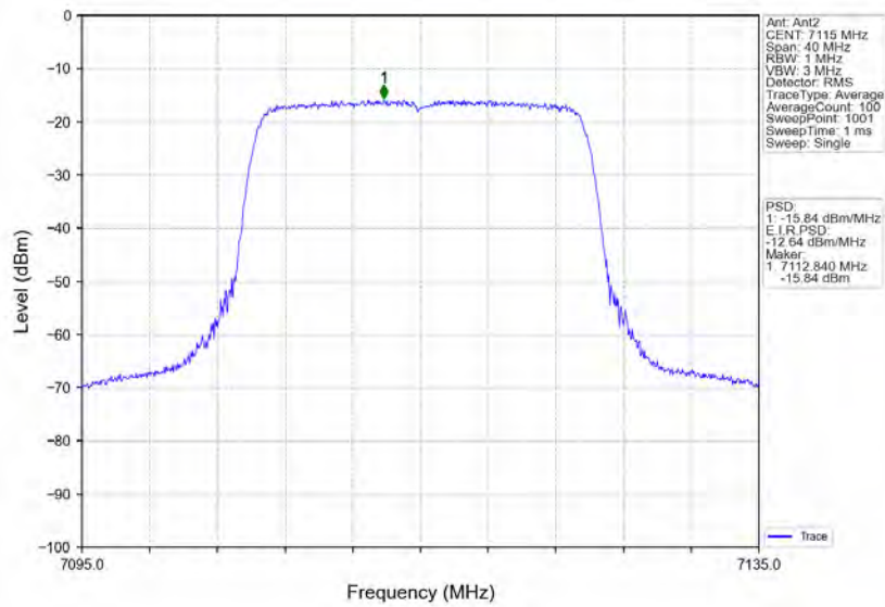
802.11ax(HEW20)_HCH_7115MHz_RU242_Left Ant2_NTNV
