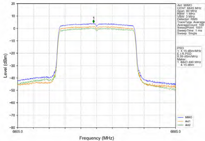
802.11ax(HEW40)_HCH_6845MHz_RU484_Left_MIMO_NTNV
