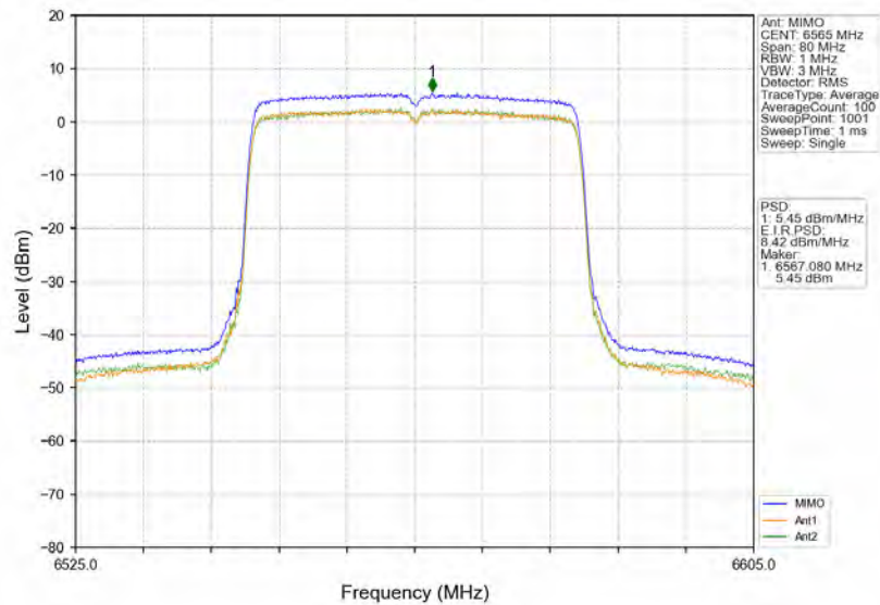
802.11ax(HEW40)_LCH_6565MHz_RU484_Left_MIMO_NTNV
