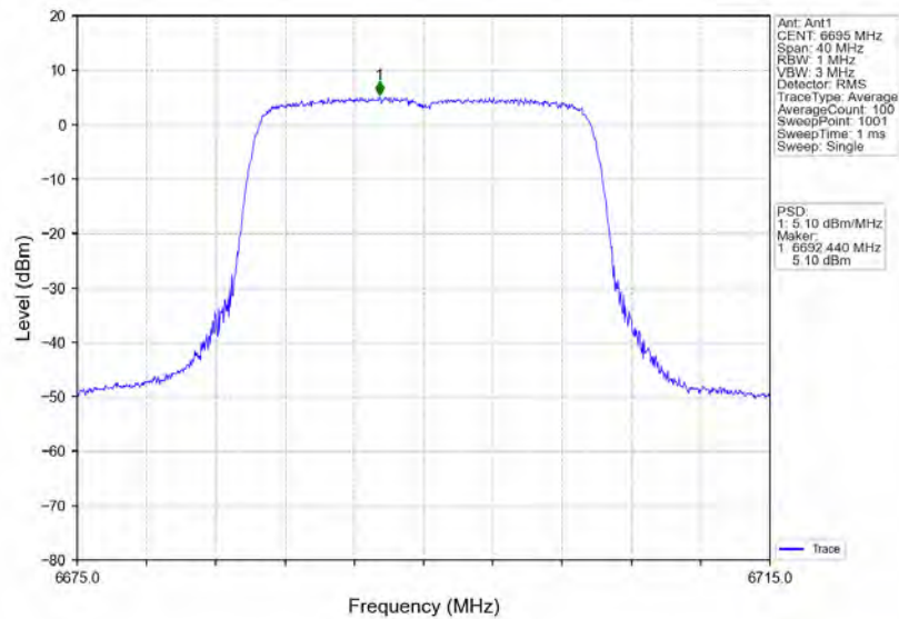
802.11ax(HEW20)_MCH_6695MHz_RU242_Left_Ant1_NTNV
