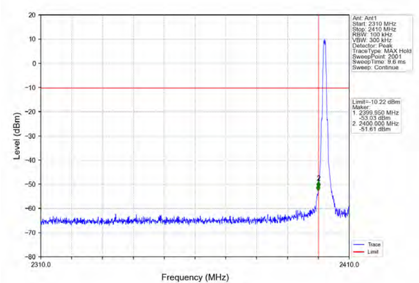
1M_LCH_2402MHz_Ant1_NTNV
