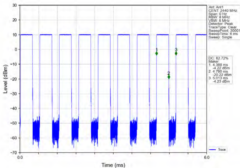
1M_MCH_2440MHz_Ant1_NTNV
