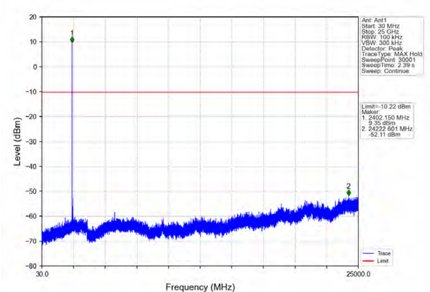
1M_LCH_2402MHz_Ant1_NTNV
