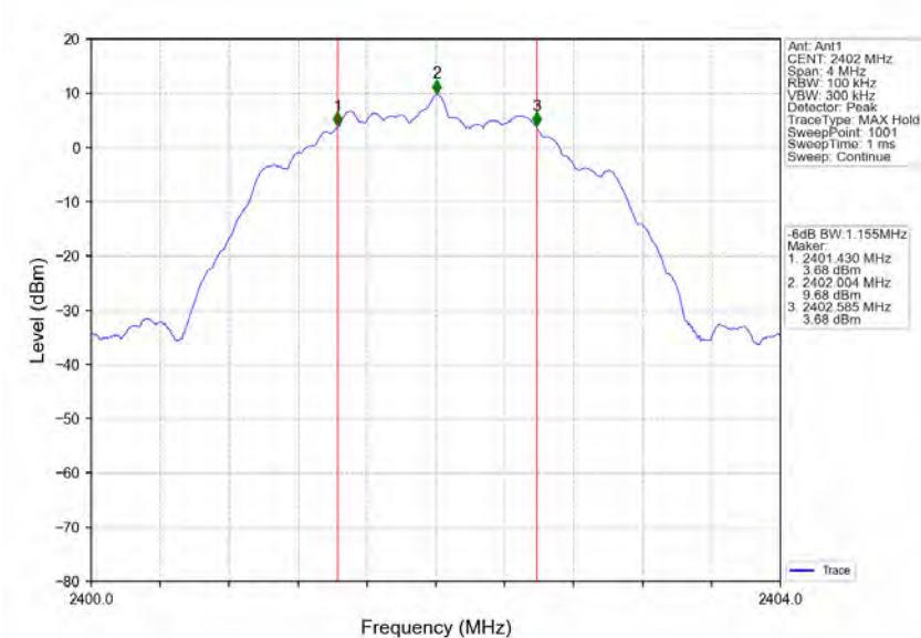
2M_LCH_2402MHz_Ant1_NTNV
