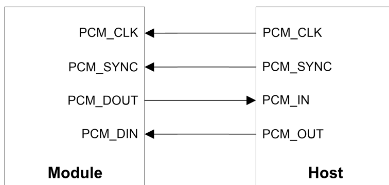
Figure 11: PCM Interface Connection
