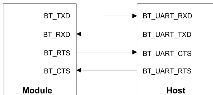
Figure 10: Bluetooth UART Connection
