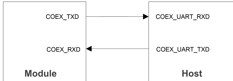
Figure 12: Coexistence Interface Connection
