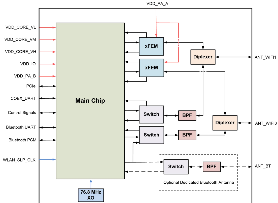
Figure 1: Functional Diagram
