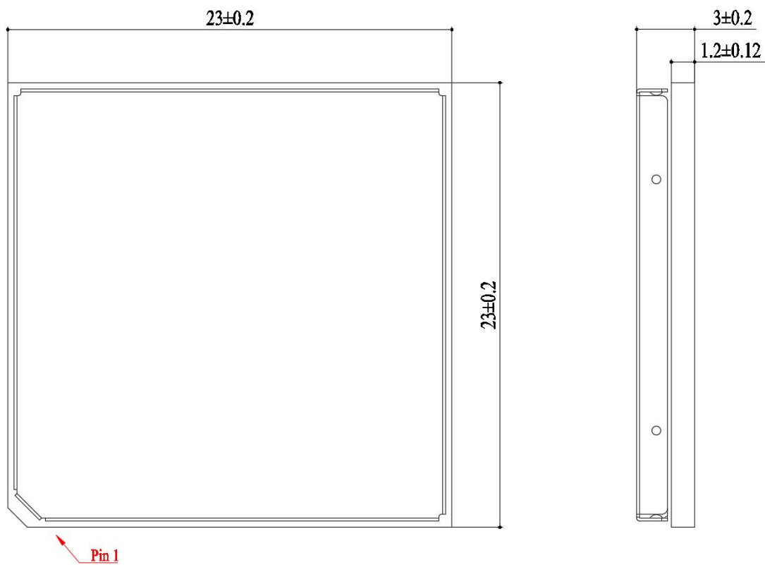
Figure 22: Top and Side Dimensions
