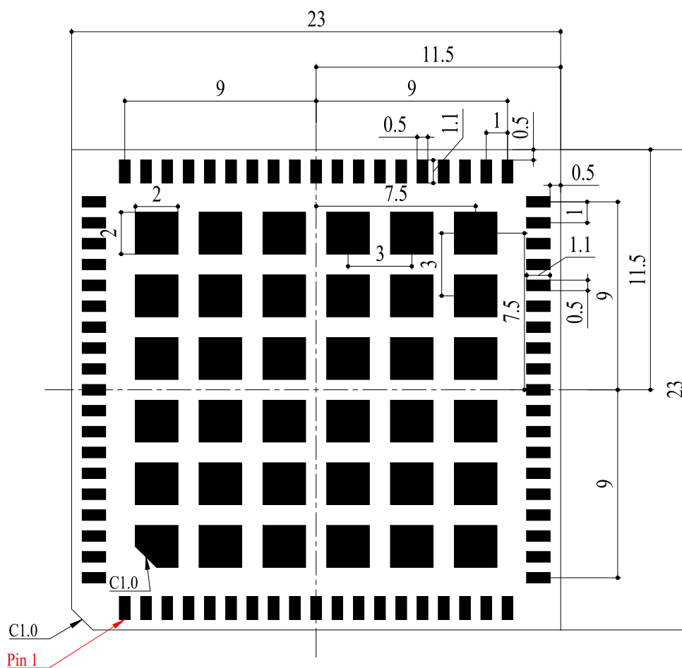
Figure 24: Recommended Footprint
