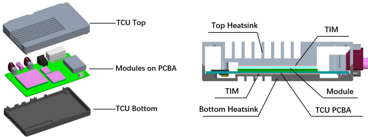
Figure 21: Heatsink Design Example
