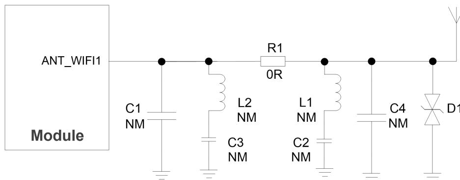
Figure 15: Reference Circuit for RF Antenna Interfaces
