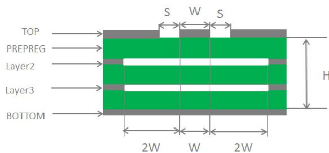
Figure 19: Coplanar Waveguide Design on a 4-layer PCB (Layer 4 as Reference Ground)
