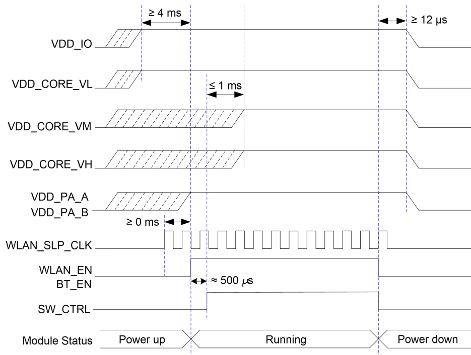
Figure 6: Timing of Power Up and Power Down
