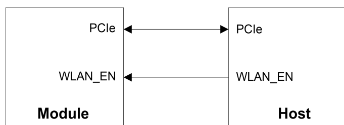
Figure 7: Wi-Fi Application Interface Connection
