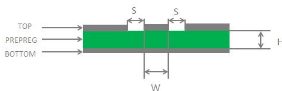
Figure 17: Coplanar Waveguide Design on a 2-layer PCB
