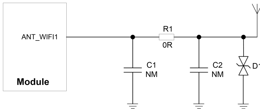
Figure 14: Reference Design for RF Antenna Interfaces
