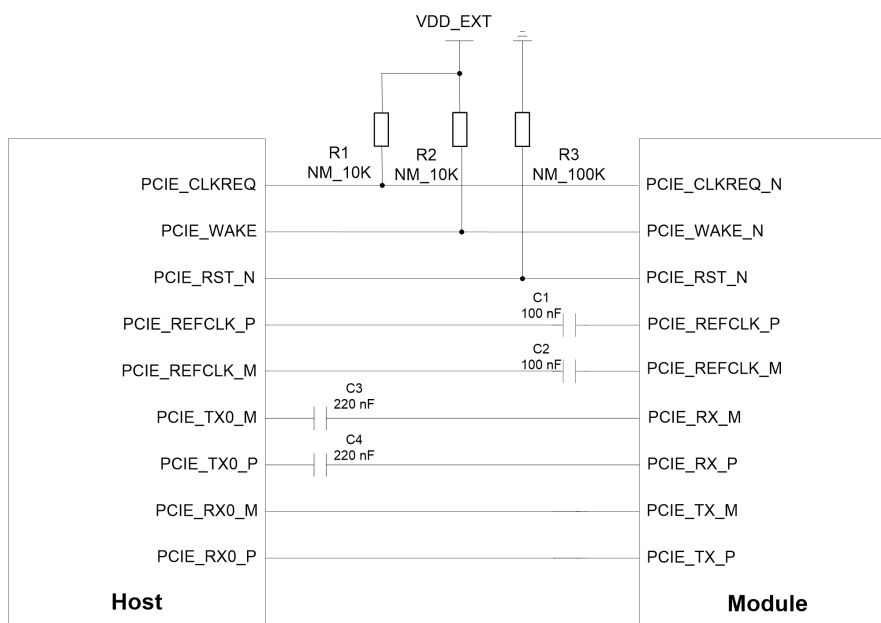
Figure 8: PCIe Interface Connection
