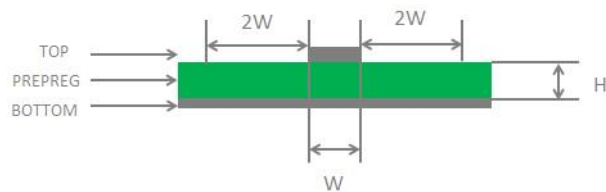
Figure 16: Microstrip Design on a 2-layer PCB
