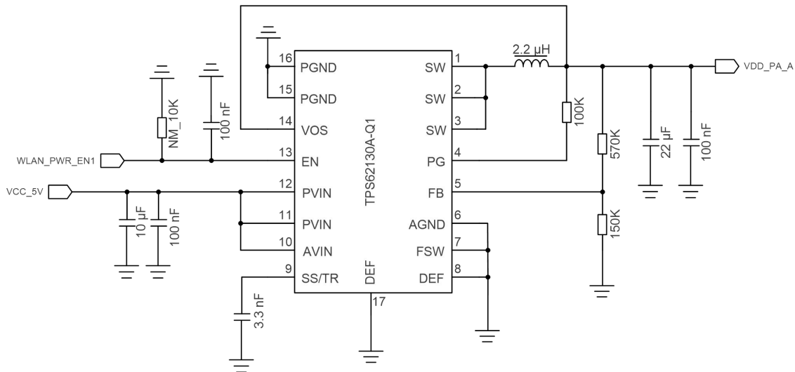
Figure 4: Reference Circuit for VDD_PA_A
