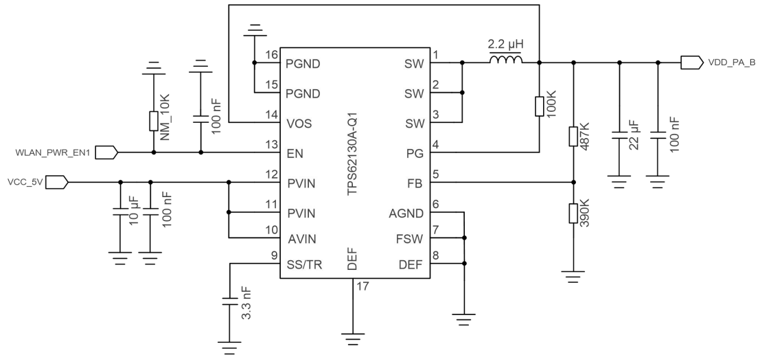
Figure 5: Reference Circuit for VDD_PA_B
