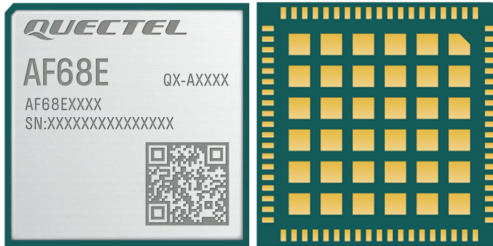
Figure 25: Top and Bottom Views
