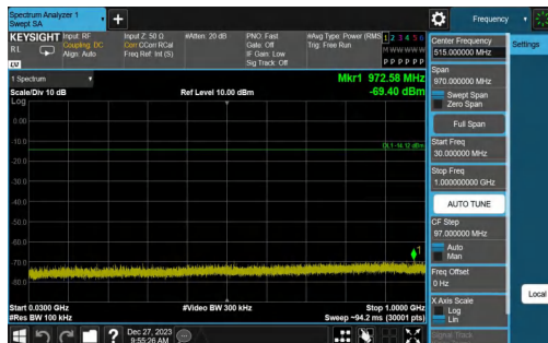
BLE_1M-Ant0-2480-30~1000-PASS
