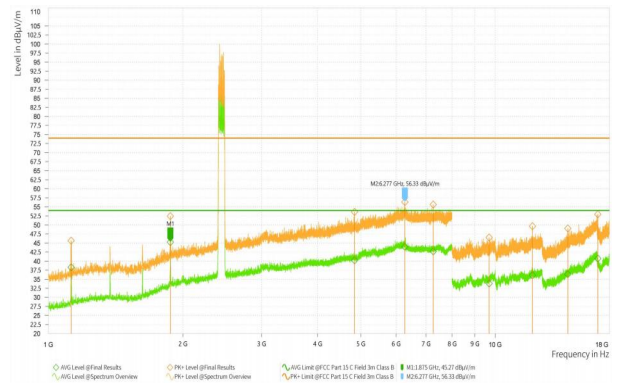
Wi-Fi 2.4G_11N40_2452_High
