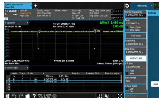
NTNV-11N40MIMO-Ant1-2452
