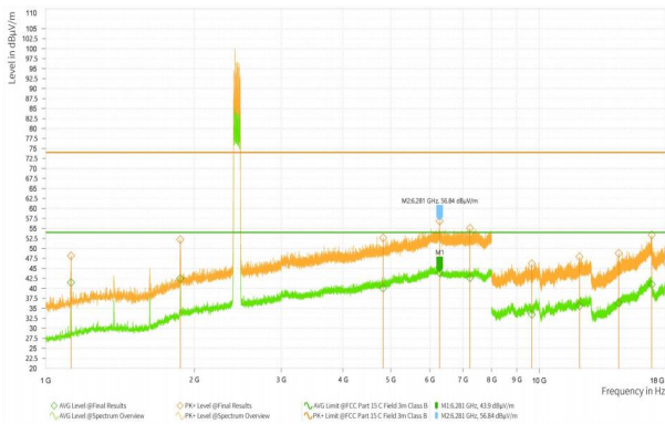
Wi-Fi 2.4G_11N20_2462_High
