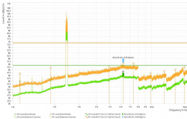
Wi-Fi 2.4G_11N40_2437_High
