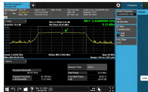
11N40SISO-Ant1-2437
