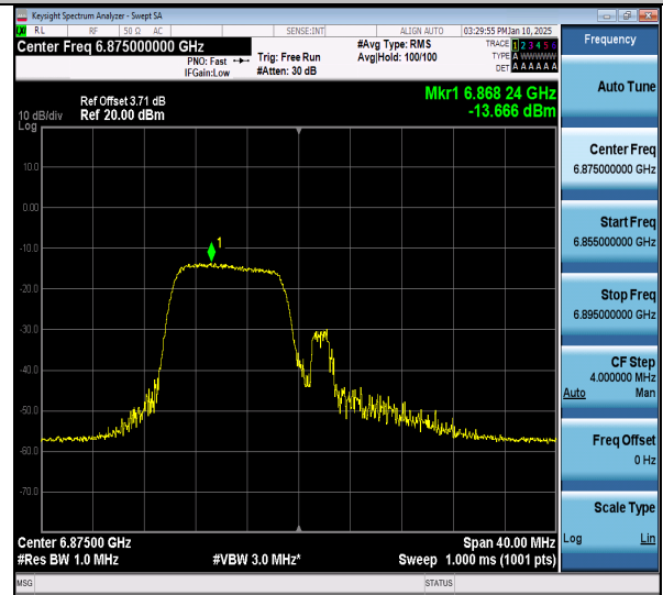
11ax20MIMO-Ant1-6875-106Tone-RU53-PASS
