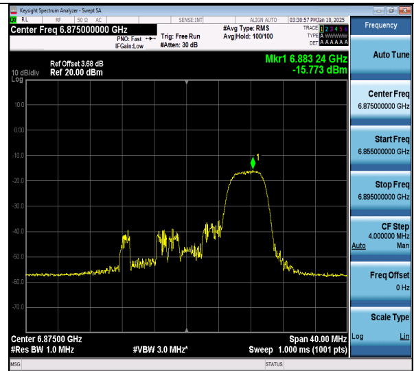
11ax20MIMO-Ant2-6875-52Tone-RU40-PASS
