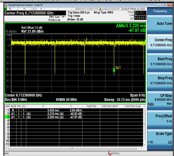
NTNV-11ax80MIMO-Ant2-6705-484Tone-RU66
