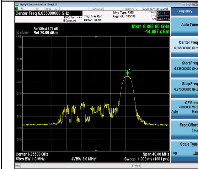
11ax20MIMO-Ant1-6855-26Tone-RU8-PASS
