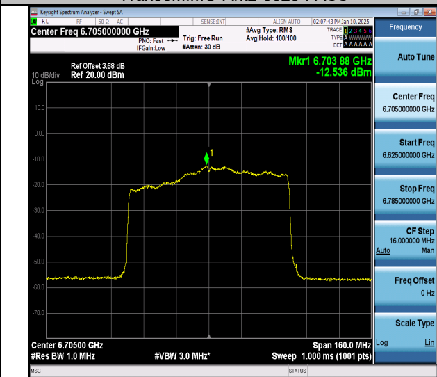
11ax80MIMO-Ant2-6705-PASS
