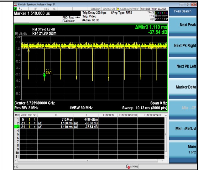
NTNV-11ax160MIMO-Ant2-6665-996Tone-RU68
