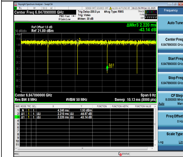
NTNV-11ax80MIMO-Ant1-6865-484Tone-RU65
