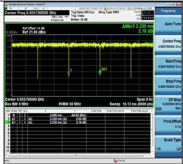
NTNV-11ax80MIMO-Ant2-6865-484Tone-RU65
