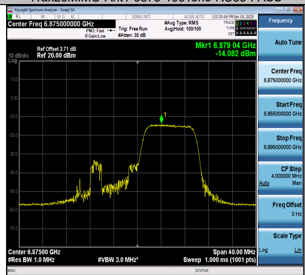
11ax20MIMO-Ant1-6875-106Tone-RU54-PASS
