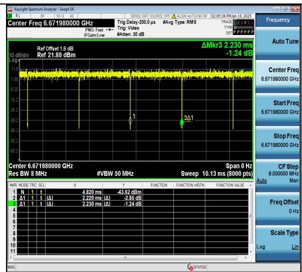
NTNV-11ax80MIMO-Ant2-6705-484Tone-RU65
