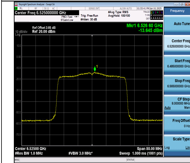
11ax40MIMO-Ant1-6525-PASS
