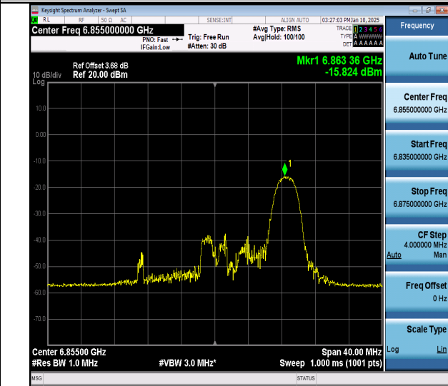
11ax20MIMO-Ant2-6855-26Tone-RU8-PASS
