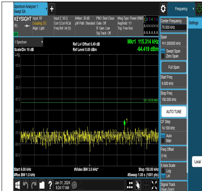
Band4-1312-0.009~0.15MHz-PASS
