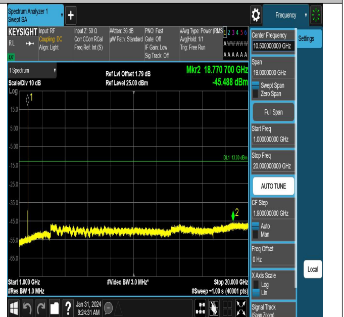
Band4-1312-1000~20000MHz-PASS
