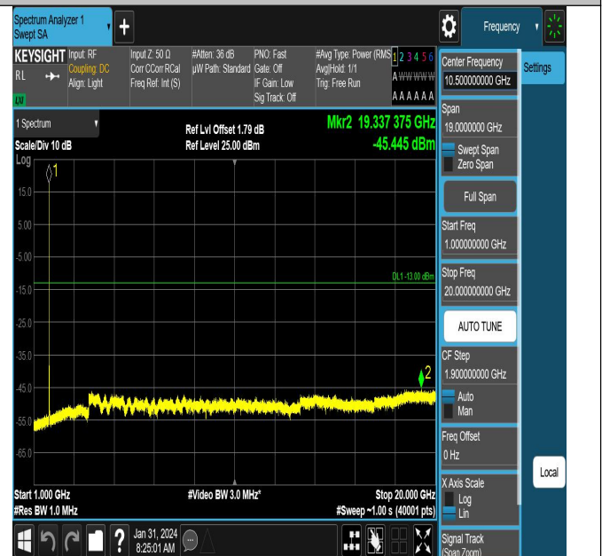
Band4-1413-1000~20000MHz-PASS
