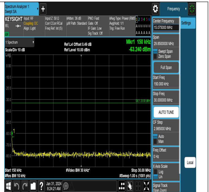
Band4-1312-0.15~30MHz-PASS
