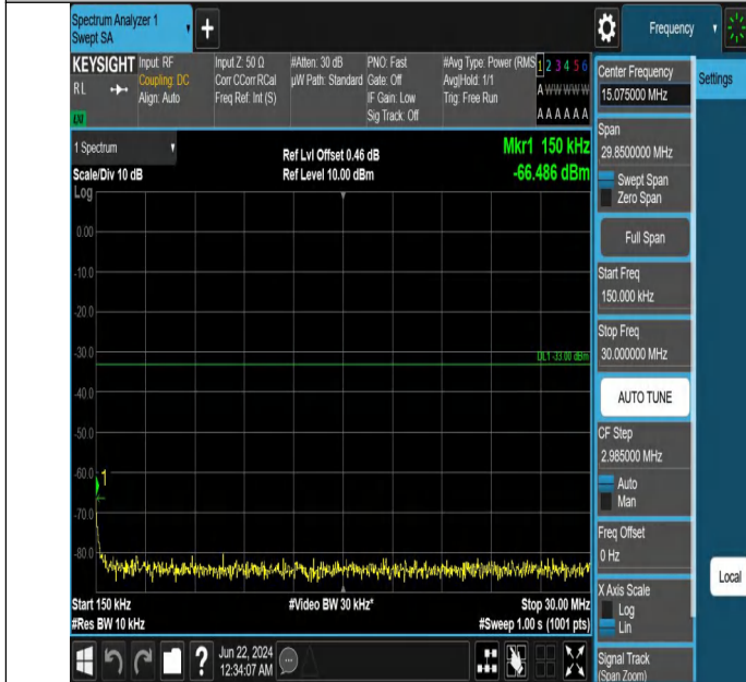
Band2_3MHz_QPSK_19185_1RB#14_0.15~30_0.15~30
