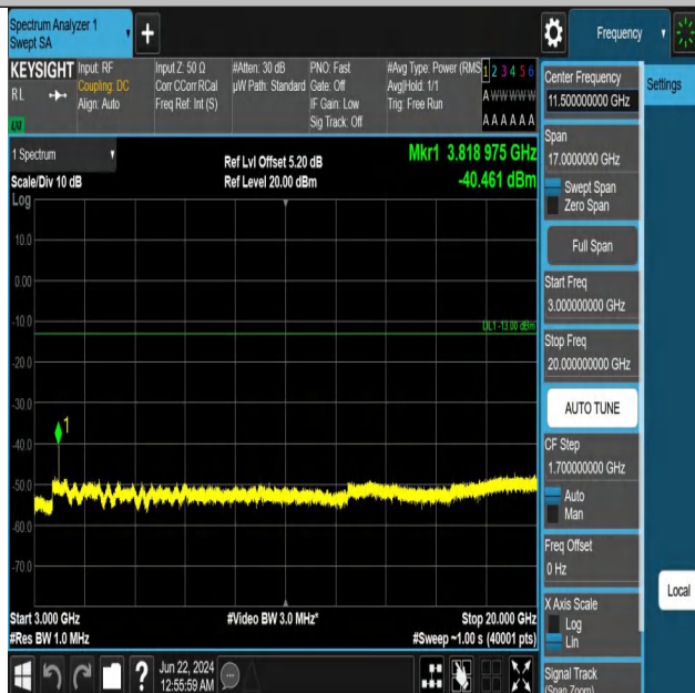
Band2_5MHz_QPSK_19175_1RB#24_3000~20000_3000~20000
