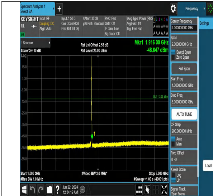
Band2_3MHz_QPSK_19185_1RB#14_1000~3000_1000~3000
