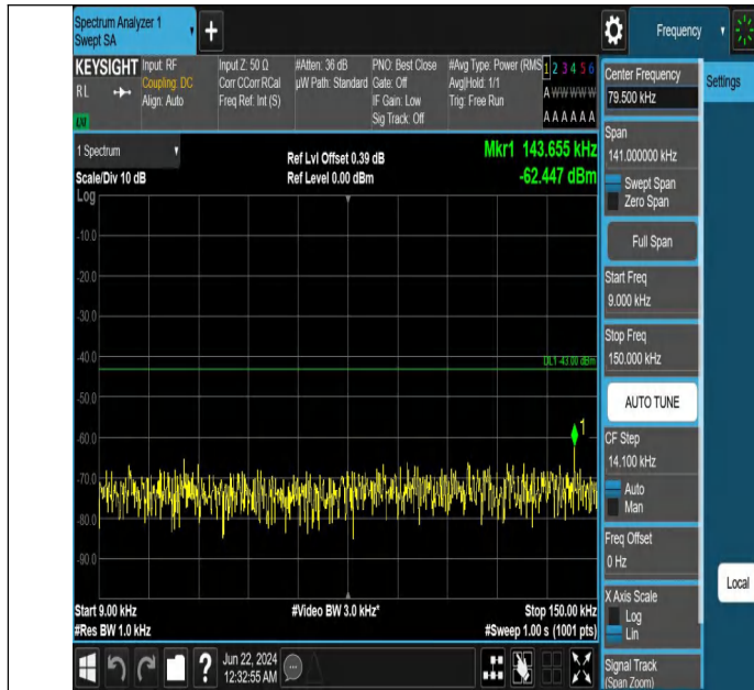
Band2_3MHz_QPSK_19185_1RB#0_0.009~0.15_0.009~0.15
