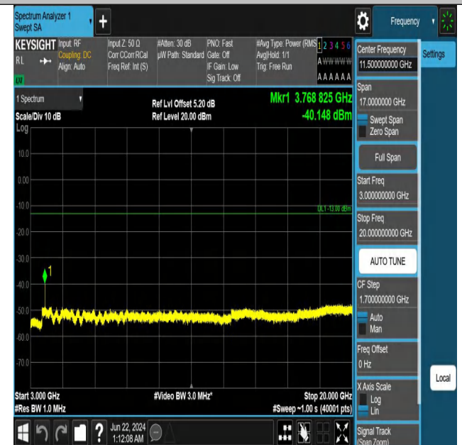
Band2_10MHz_QPSK_18900_1RB#49_3000~20000_3000~2000
