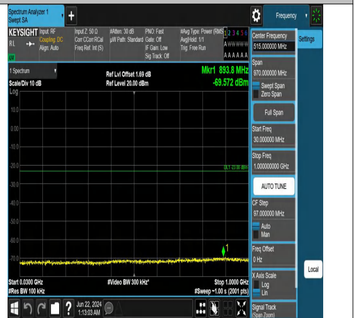
Band2_10MHz_QPSK_19150_1RB#0_30~1000_30~1000
