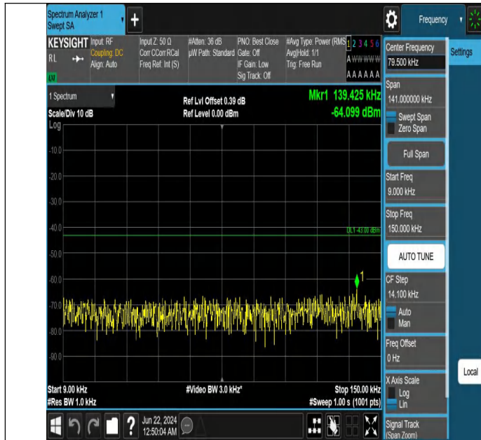
Band2_5MHz_QPSK_18625_25RB#0_0.009~0.15_0.009~0.15
