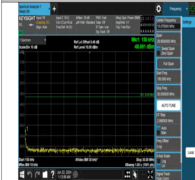
Band2_10MHz_QPSK_19150_1RB#0_0.15~30_0.15~30
