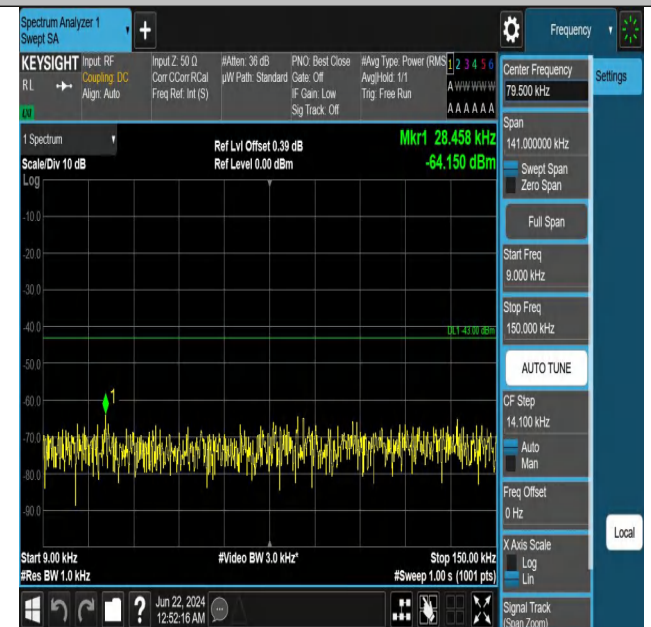
Band2_5MHz_QPSK_18900_1RB#24_0.009~0.15_0.009~0.15
