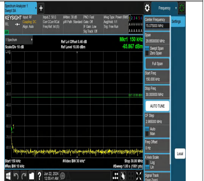
Band2_5MHz_QPSK_19175_1RB#24_0.15~30_0.15~30
