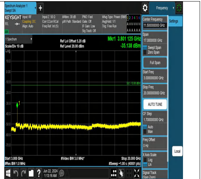
Band2_10MHz_QPSK_19150_1RB#0_3000~20000_3000~20000
