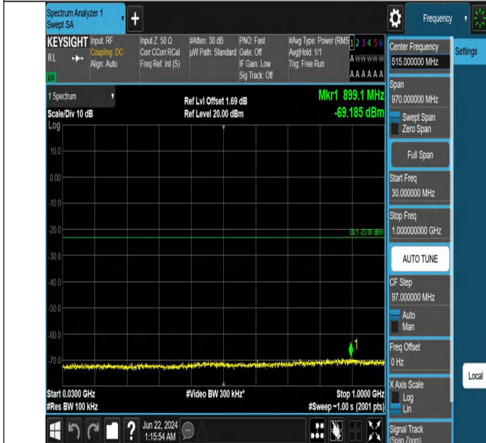
Band2_10MHz_QPSK_18900_50RB#0_30~1000_30~1000
