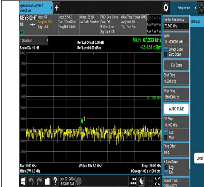
Band2_10MHz_QPSK_19150_1RB#49_0.009~0.15_0.009~0.15
