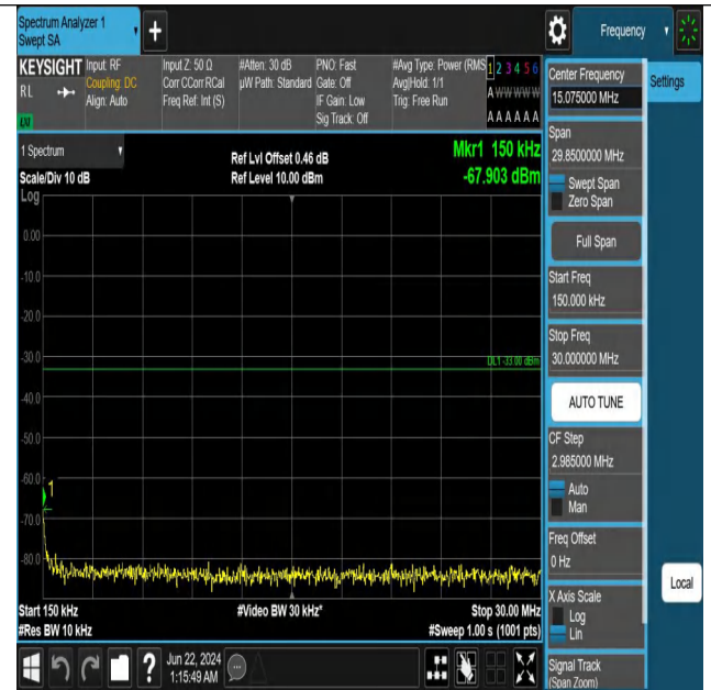
Band2_10MHz_QPSK_18900_50RB#0_0.15~30_0.15~30
