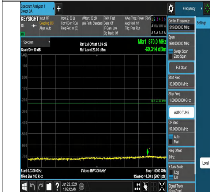
Band2_10MHz_QPSK_18650_1RB#49_30~1000_30~1000
