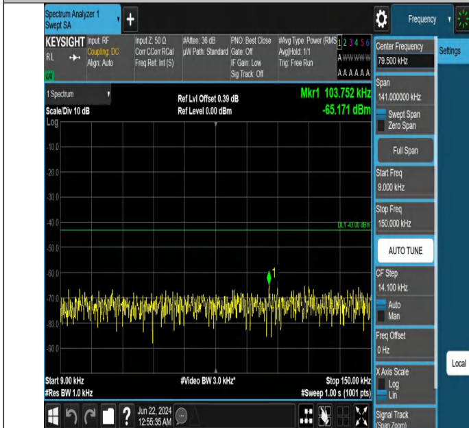
Band2_5MHz_QPSK_19175_1RB#24_0.009~0.15_0.009~0.15
