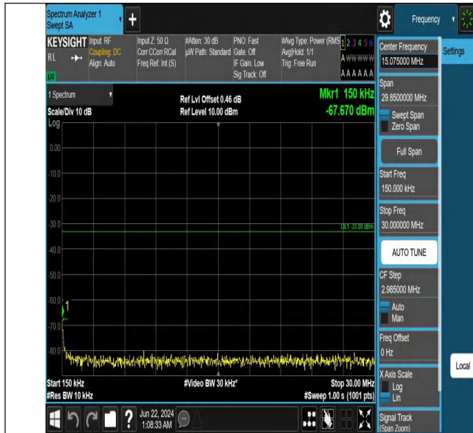
Band2_10MHz_QPSK_18650_1RB#0_0.15~30_0.15~30
