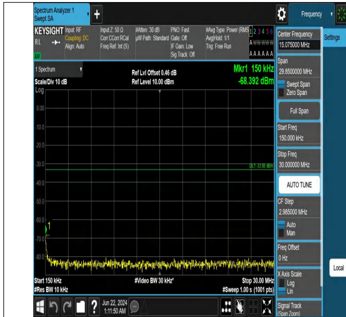
Band2_10MHz_QPSK_18900_1RB#49_0.15~30_0.15~30
