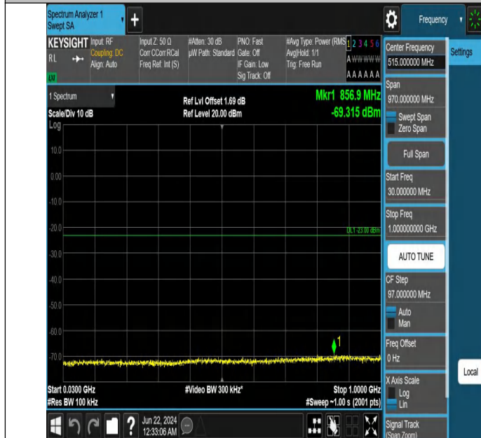
Band2_3MHz_QPSK_19185_1RB#0_30~1000_30~1000
