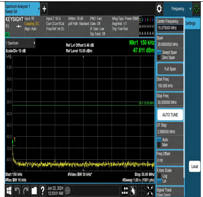
Band2_3MHz_QPSK_19185_1RB#0_0.15~30_0.15~30
