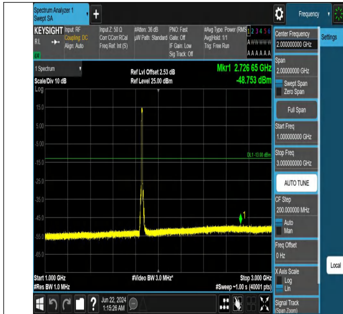
Band2_10MHz_QPSK_18650_50RB#0_1000~3000_1000~3000
