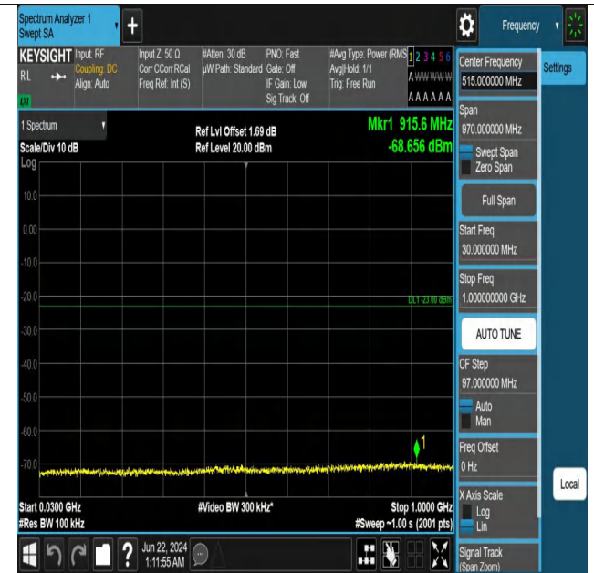
Band2_10MHz_QPSK_18900_1RB#49_30~1000_30~1000
