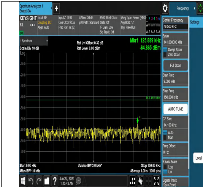
Band2_10MHz_QPSK_18900_50RB#0_0.009~0.15_0.009~0.15
