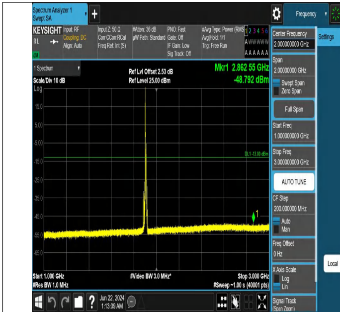
Band2_10MHz_QPSK_19150_1RB#0_1000~3000_1000~3000
