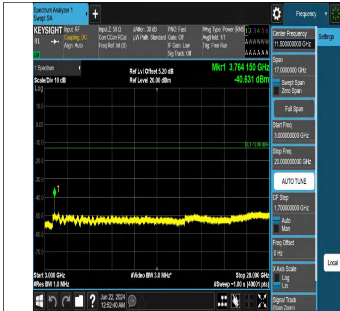
Band2_5MHz_QPSK_18900_1RB#24_3000~20000_3000~20000
