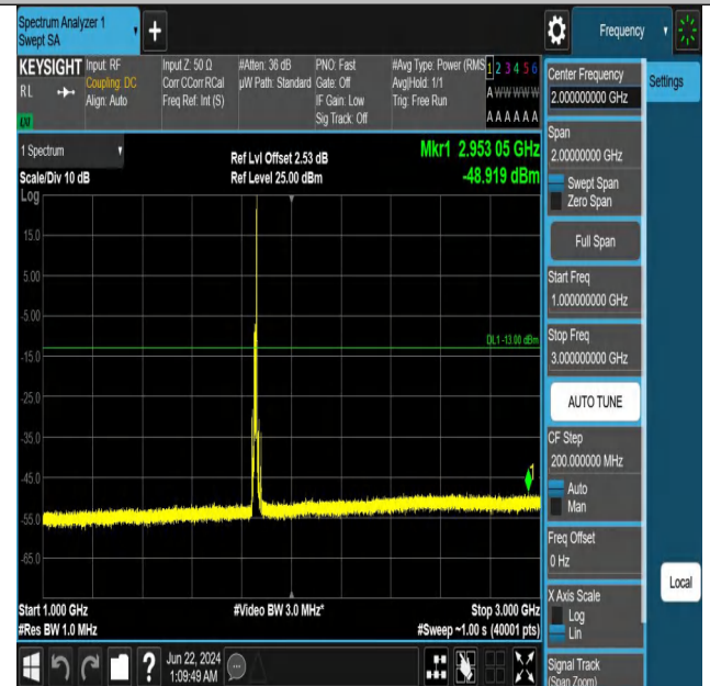
Band2_10MHz_QPSK_18650_1RB#49_1000~3000_1000~3000
