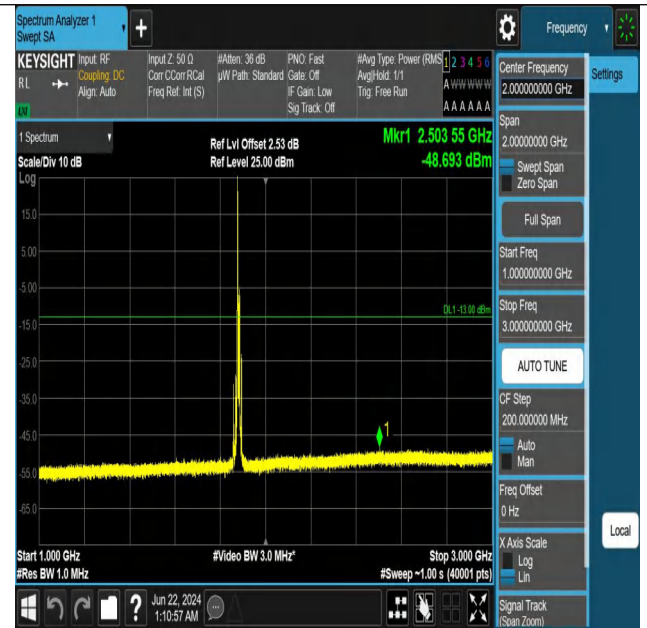
Band2_10MHz_QPSK_18900_1RB#0_1000~3000_1000~3000
