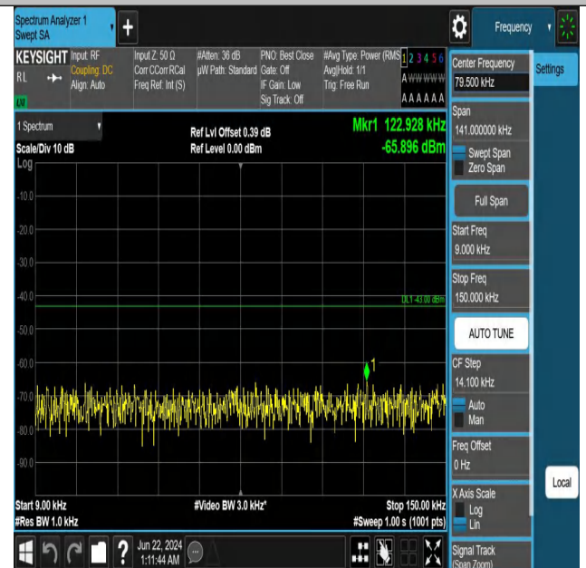
Band2_10MHz_QPSK_18900_1RB#49_0.009~0.15_0.009~0.15
