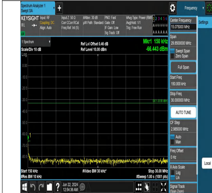
Band2_5MHz_QPSK_19175_1RB#0_0.15~30_0.15~30
