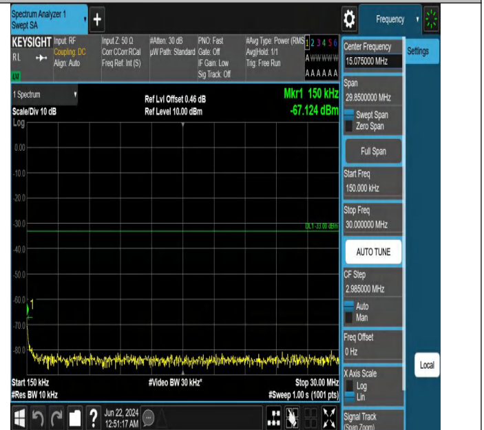
Band2_5MHz_QPSK_18900_1RB#0_0.15~30_0.15~30
