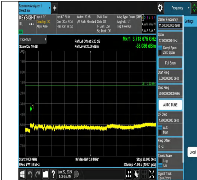
Band2_10MHz_QPSK_18650_1RB#49_3000~20000_3000~2000
