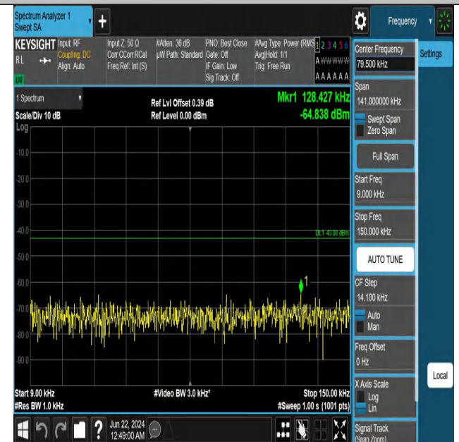
Band2_5MHz_QPSK_18625_1RB#24_0.009~0.15_0.009~0.15
