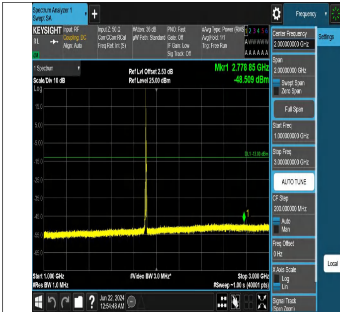
Band2_5MHz_QPSK_19175_1RB#0_1000~3000_1000~3000
