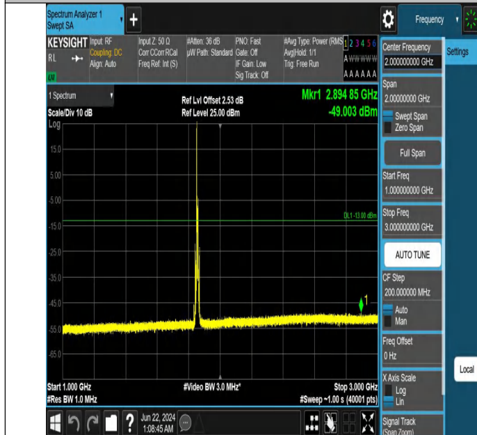
Band2_10MHz_QPSK_18650_1RB#0_1000~3000_1000~3000
