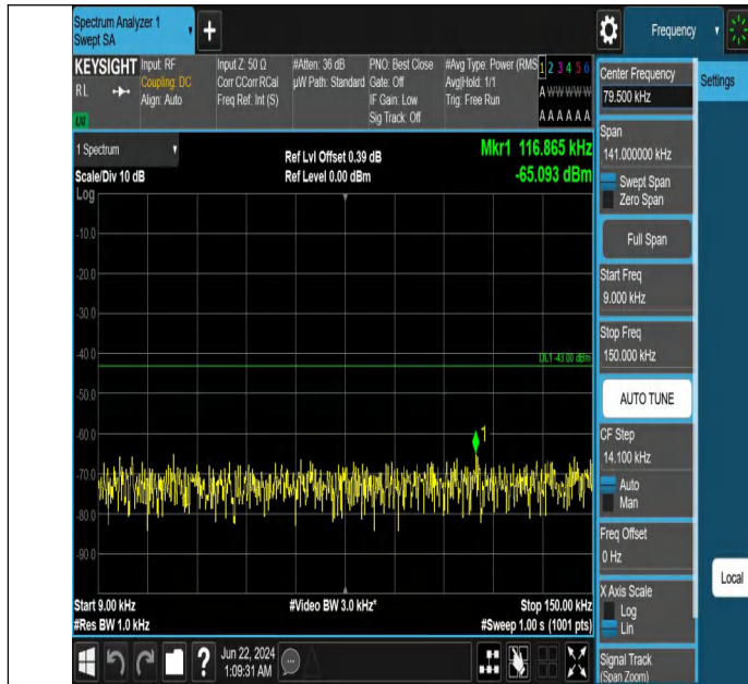
Band2_10MHz_QPSK_18650_1RB#49_0.009~0.15_0.009~0.15
