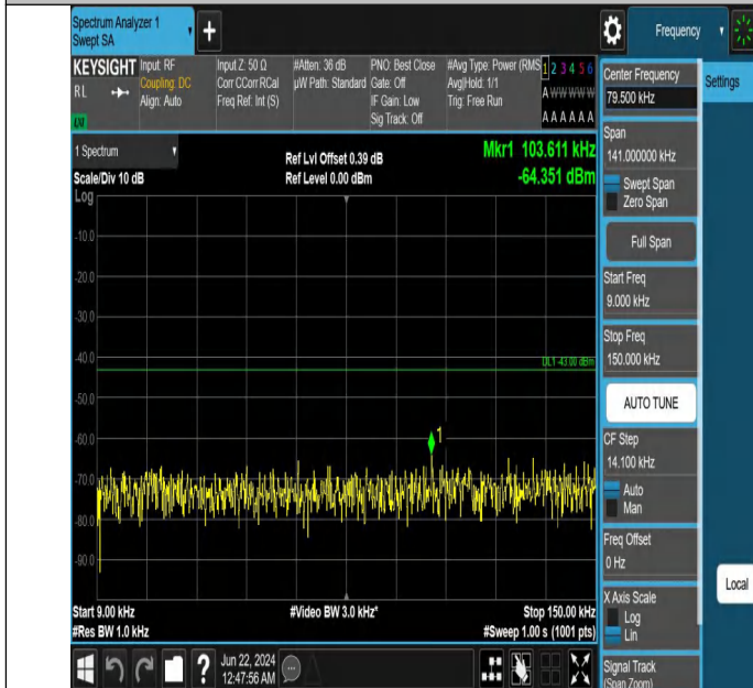
Band2_5MHz_QPSK_18625_1RB#0_0.009~0.15_0.009~0.15
