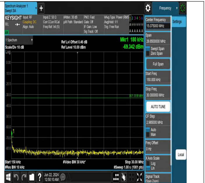
Band2_5MHz_QPSK_18625_25RB#0_0.15~30_0.15~30
