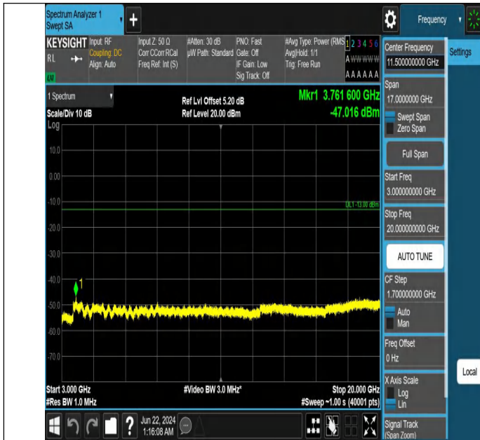
Band2_10MHz_QPSK_18900_50RB#0_3000~20000_3000~2000
