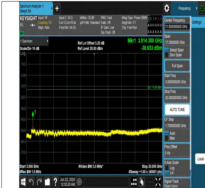
Band2_3MHz_QPSK_19185_1RB#0_3000~20000_3000~20000
