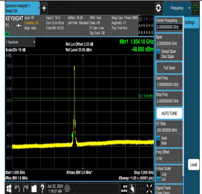
Band2_10MHz_QPSK_18900_50RB#0_1000~3000_1000~3000
