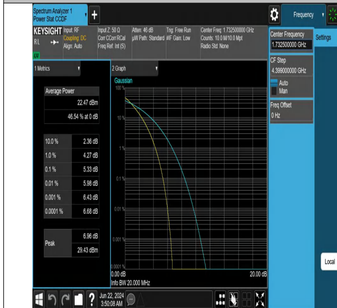
Band4-20MHz-QPSK-20175-100RB#0-PASS
