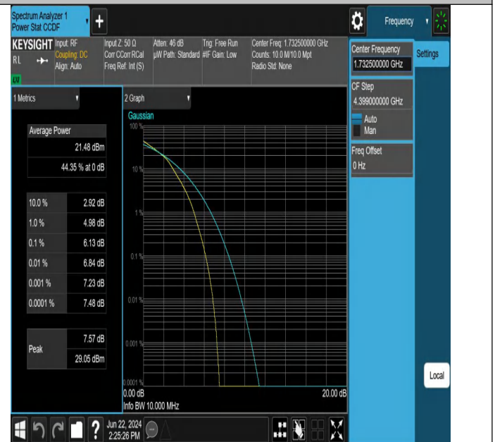
Band4-10MHz-16QAM-20175-27RB#0-PASS
