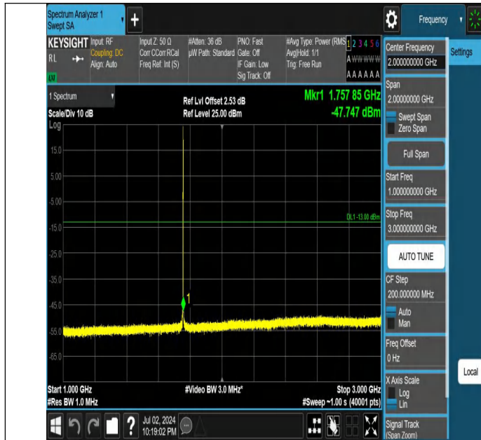
Band4-1.4MHz-QPSK-20393-1RB#5-1000~3000-PASS
