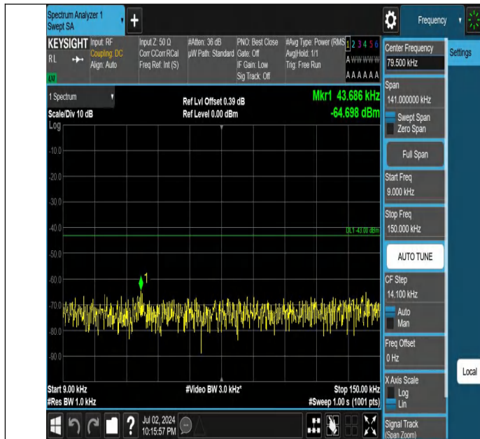
Band4-1.4MHz-QPSK-19957-1RB#0-0.009~0.15-PASS
