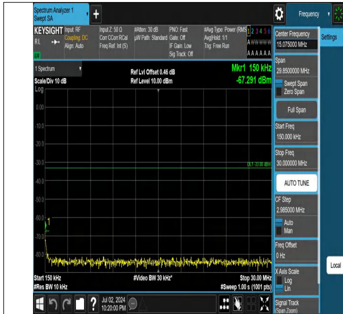
Band4-3MHz-QPSK-19965-1RB#14-0.15~30-PASS
