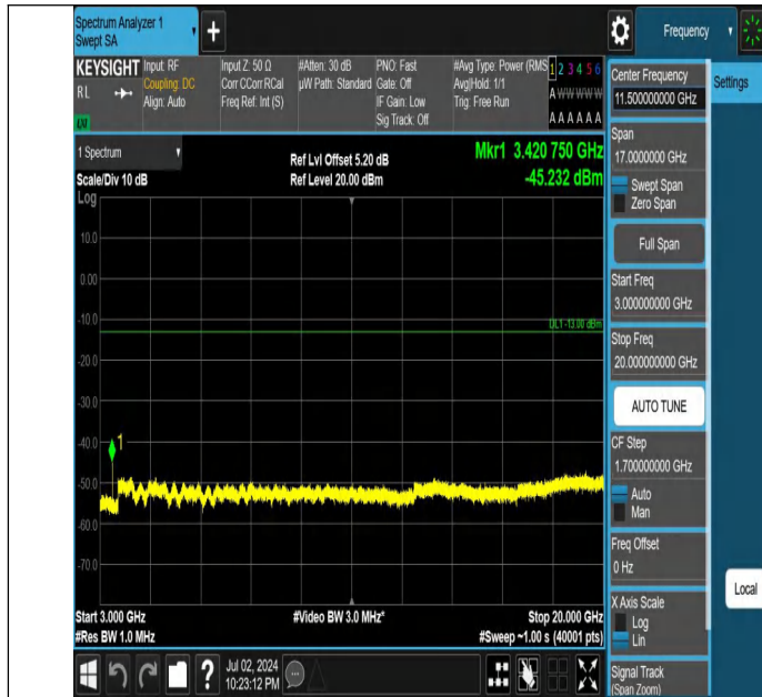
Band4-5MHz-QPSK-19975-1RB#0-3000~20000-PASS
