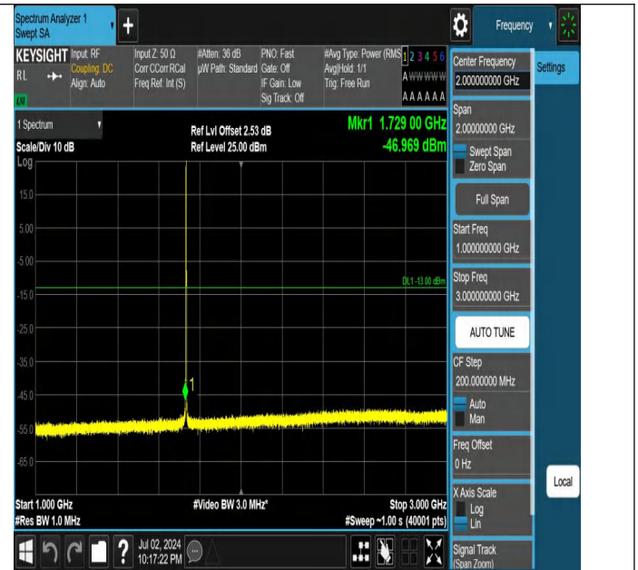
Band4-1.4MHz-QPSK-20175-1RB#0-1000~3000-PASS
