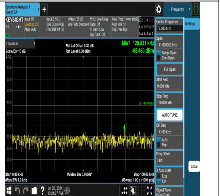
Band4-5MHz-QPSK-20175-1RB#24-0.009~0.15-PASS
