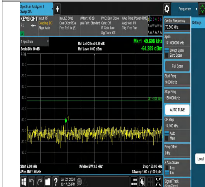
Band4-1.4MHz-QPSK-20175-1RB#0-0.009~0.15-PASS
