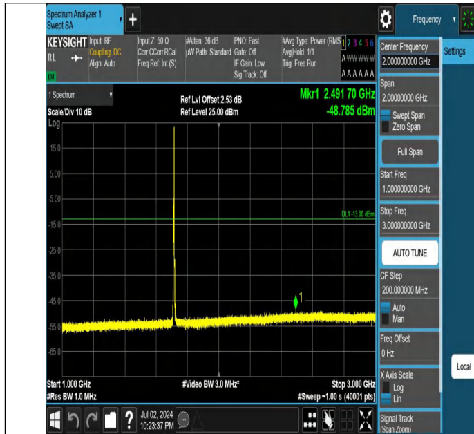
Band4-5MHz-QPSK-19975-1RB#24-1000~3000-PASS
