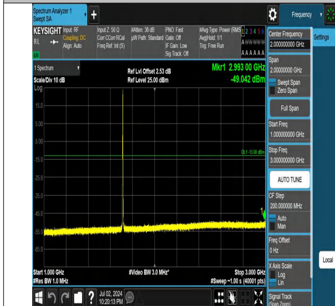
Band4-3MHz-QPSK-19965-1RB#14-1000~3000-PASS
