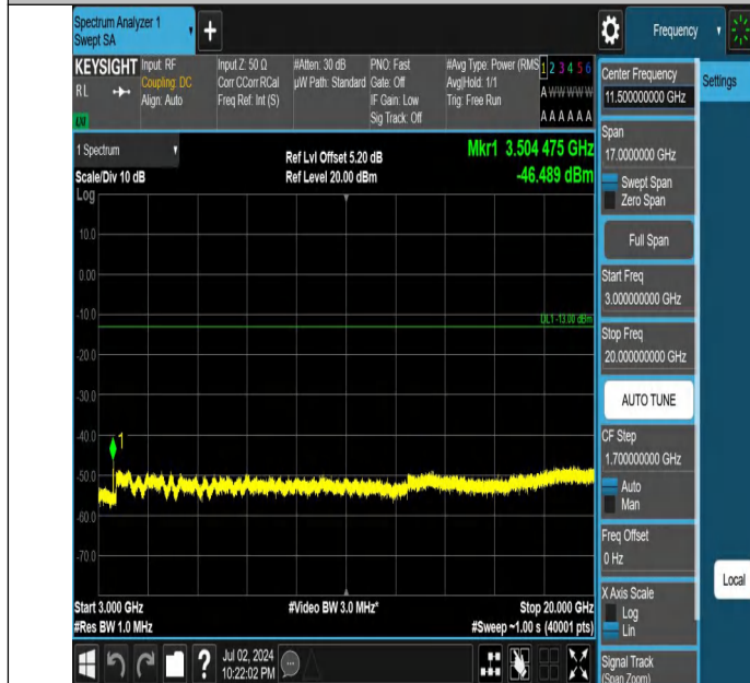
Band4-3MHz-QPSK-20385-1RB#0-3000~20000-PASS
