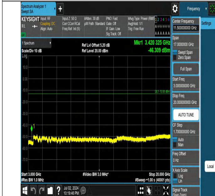
Band4-3MHz-QPSK-19965-1RB#0-3000~20000-PASS
