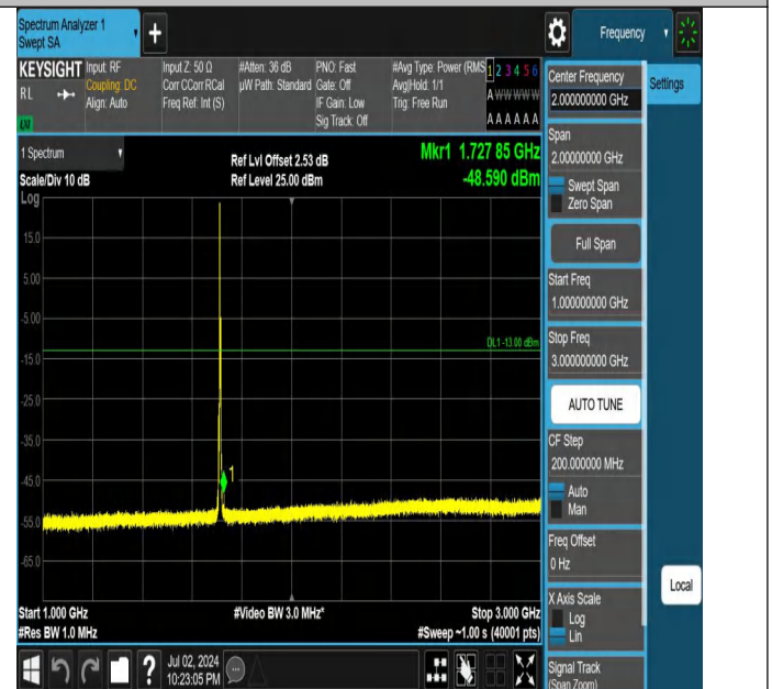
Band4-5MHz-QPSK-19975-1RB#0-1000~3000-PASS
