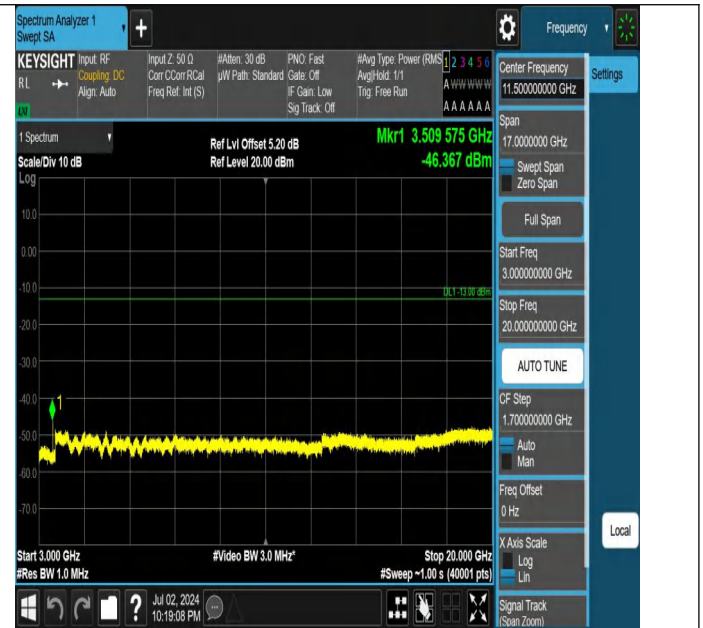
Band4-1.4MHz-QPSK-20393-1RB#5-3000~20000-PASS
