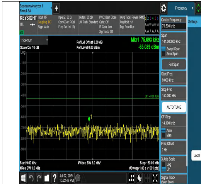
Band4-5MHz-QPSK-19975-1RB#0-0.009~0.15-PASS
