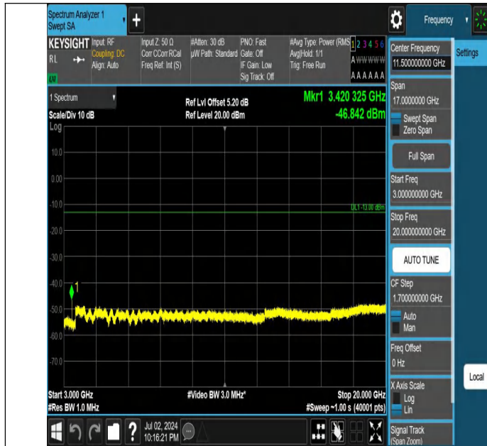
Band4-1.4MHz-QPSK-19957-1RB#0-3000~20000-PASS
