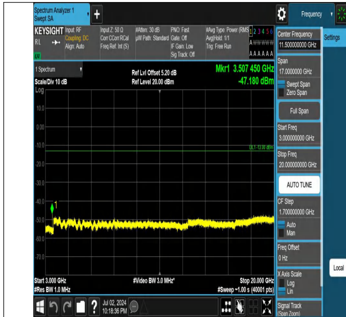
Band4-1.4MHz-QPSK-20393-1RB#0-3000~20000-PASS
