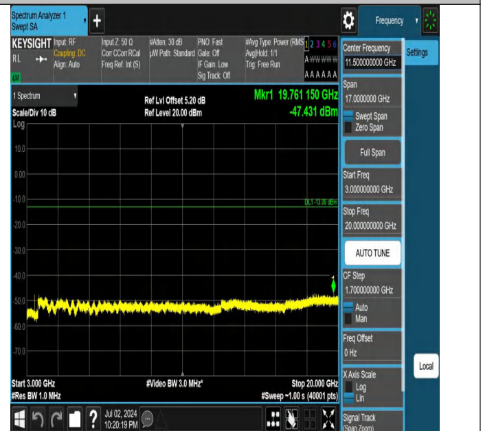
Band4-3MHz-QPSK-19965-1RB#14-3000~20000-PASS
