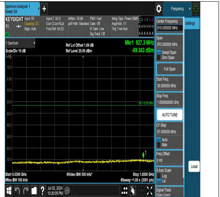
Band4-3MHz-QPSK-19965-1RB#14-30~1000-PASS
