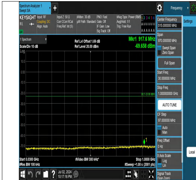
Band4-1.4MHz-QPSK-20175-1RB#0-30~1000-PASS
