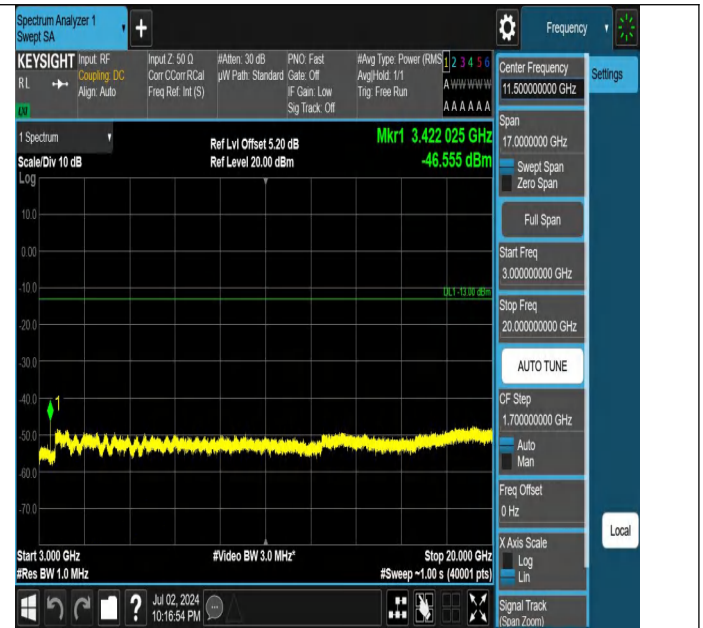
Band4-1.4MHz-QPSK-19957-1RB#5-3000~20000-PASS
