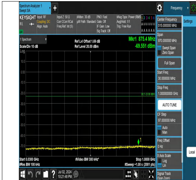
Band4-3MHz-QPSK-20385-1RB#0-30~1000-PASS
