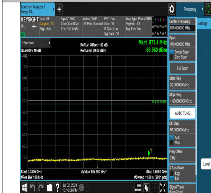
Band4-1.4MHz-QPSK-19957-1RB#0-30~1000-PASS
