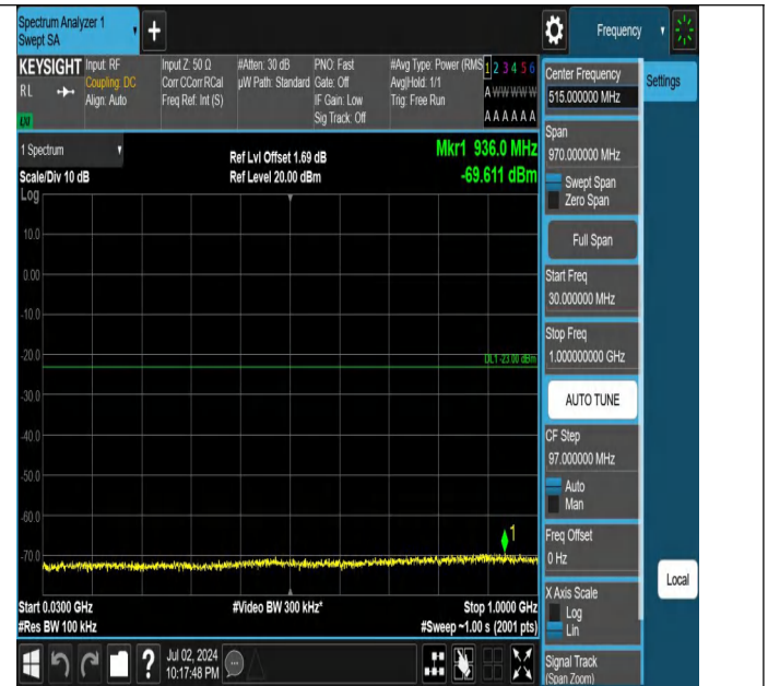
Band4-1.4MHz-QPSK-20175-1RB#5-30~1000-PASS
