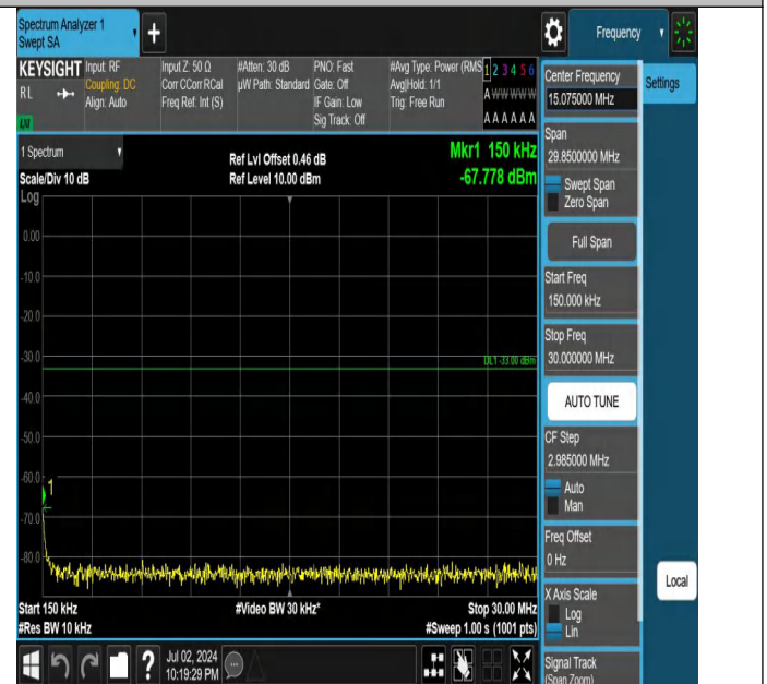
Band4-3MHz-QPSK-19965-1RB#0-0.15~30-PASS
