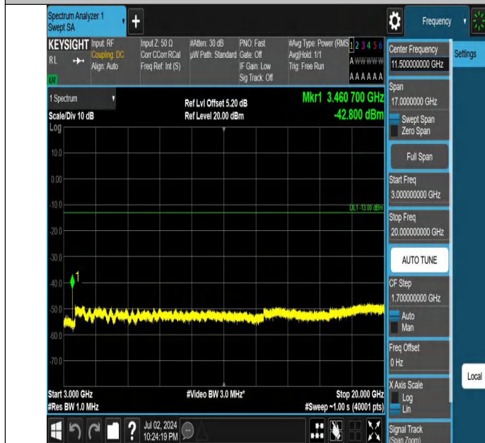
Band4-5MHz-QPSK-20175-1RB#0-3000~20000-PASS
