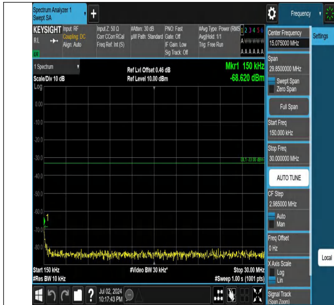
Band4-1.4MHz-QPSK-20175-1RB#5-0.15~30-PASS
