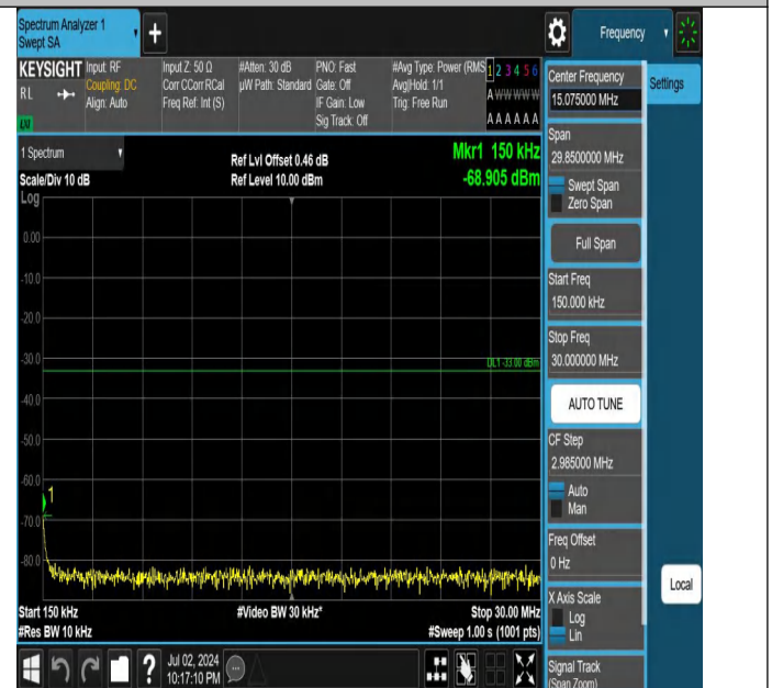
Band4-1.4MHz-QPSK-20175-1RB#0-0.15~30-PASS
