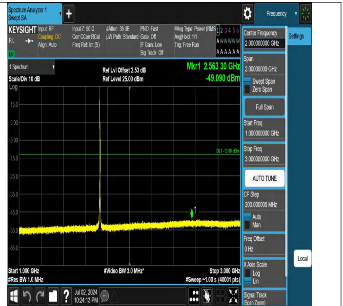
Band4-5MHz-QPSK-20175-1RB#0-1000~3000-PASS
