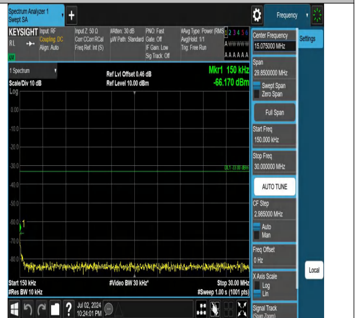
Band4-5MHz-QPSK-20175-1RB#0-0.15~30-PASS
