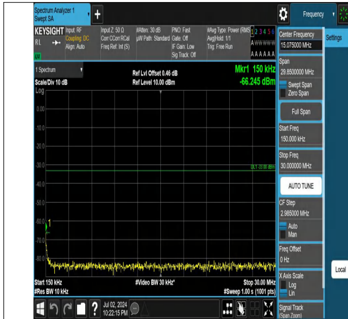
Band4-3MHz-QPSK-20385-1RB#14-0.15~30-PASS
