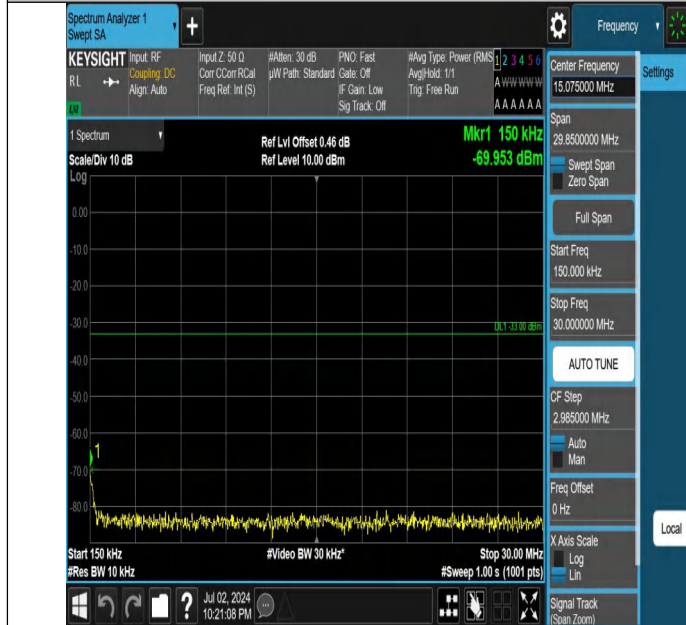
Band4-3MHz-QPSK-20175-1RB#14-0.15~30-PASS
