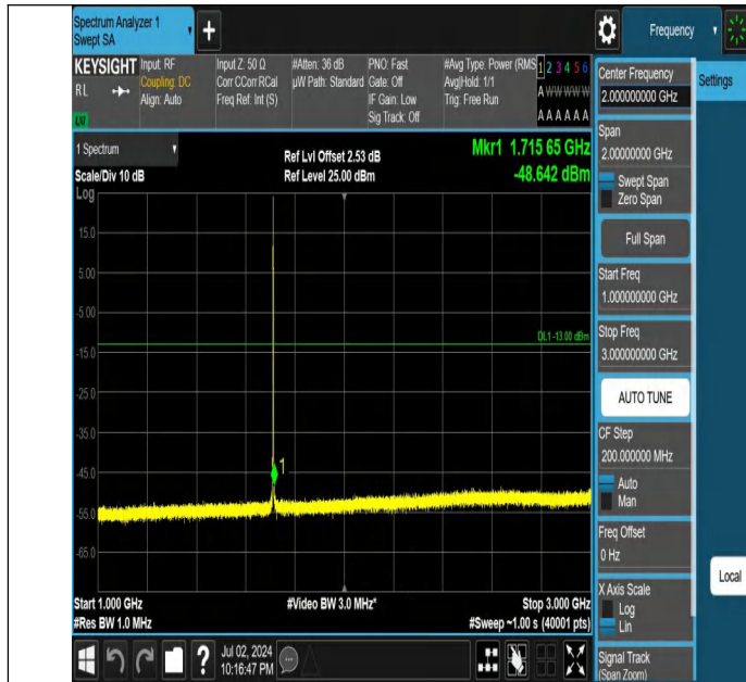
Band4-1.4MHz-QPSK-19957-1RB#5-1000~3000-PASS
