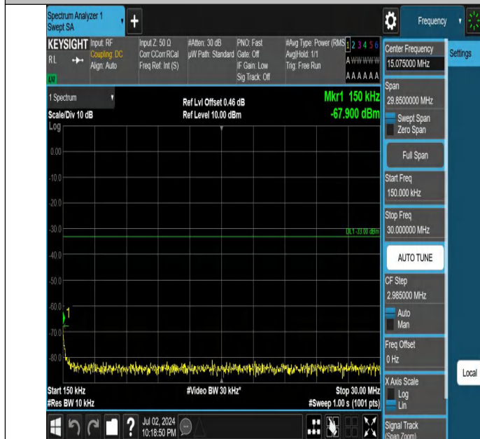
Band4-1.4MHz-QPSK-20393-1RB#5-0.15~30-PASS
