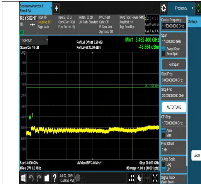
Band4-3MHz-QPSK-20175-1RB#0-3000~20000-PASS
