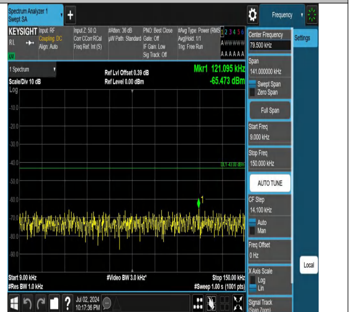
Band4-1.4MHz-QPSK-20175-1RB#5-0.009~0.15-PASS
