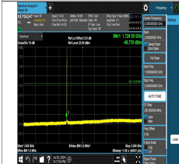
Band4-1.4MHz-QPSK-20175-1RB#5-1000~3000-PASS
