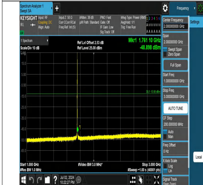
Band4-3MHz-QPSK-20385-1RB#14-1000~3000-PASS
