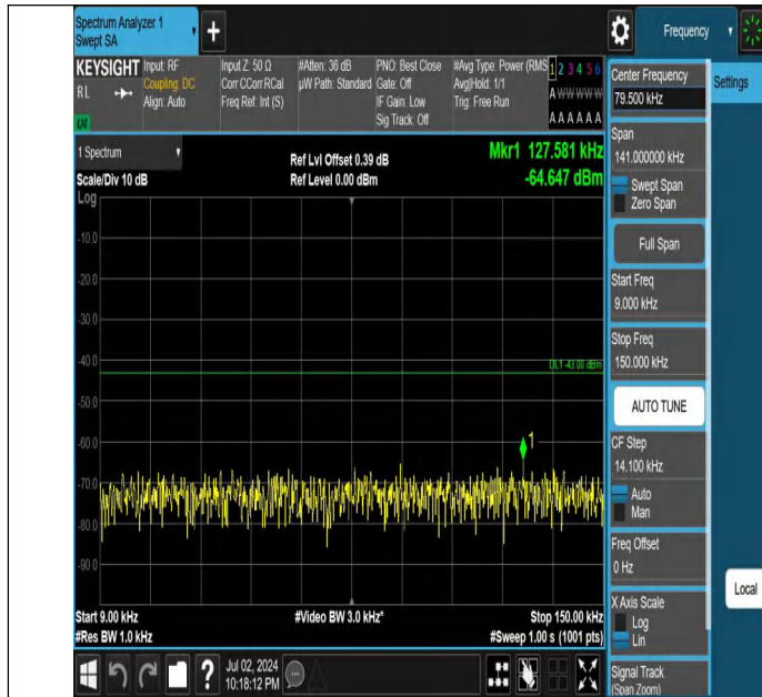
Band4-1.4MHz-QPSK-20393-1RB#0-0.009~0.15-PASS
