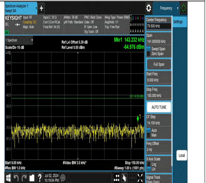
Band4-3MHz-QPSK-19965-1RB#14-0.009~0.15-PASS
