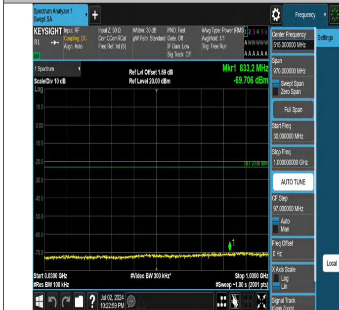
Band4-5MHz-QPSK-19975-1RB#0-30~1000-PASS
