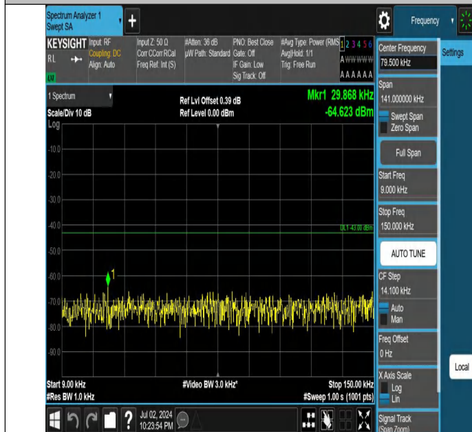
Band4-5MHz-QPSK-20175-1RB#0-0.009~0.15-PASS
