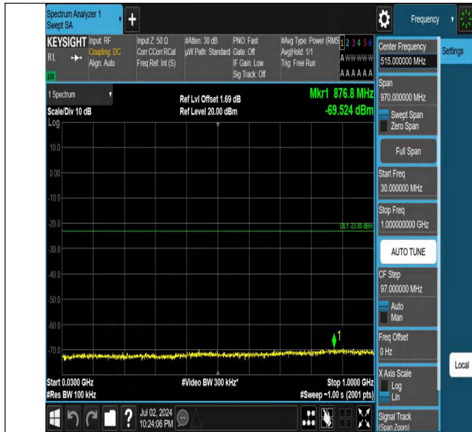
Band4-5MHz-QPSK-20175-1RB#0-30~1000-PASS
