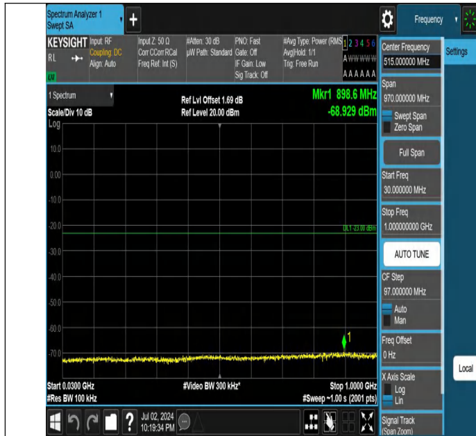
Band4-3MHz-QPSK-19965-1RB#0-30~1000-PASS
