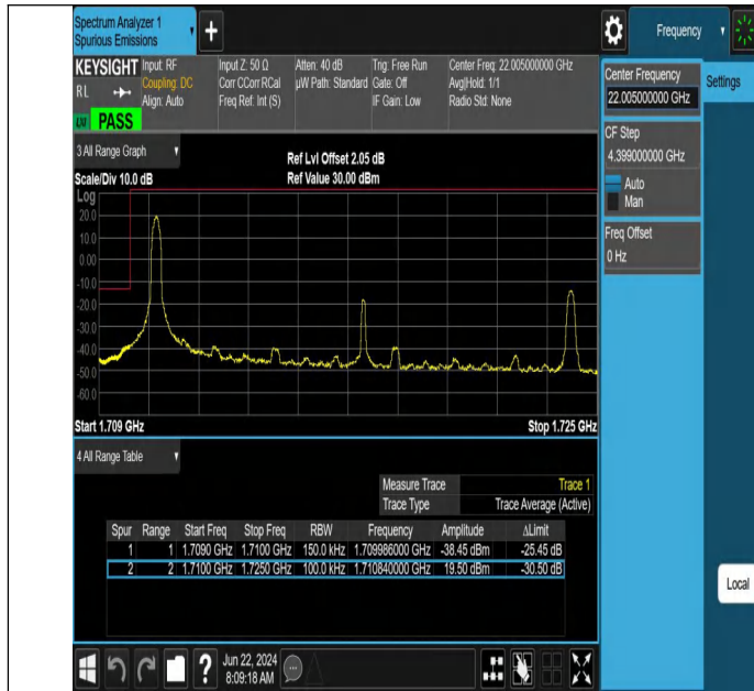
Band66-15MHz-QPSK-132047-1RB#0-PASS
