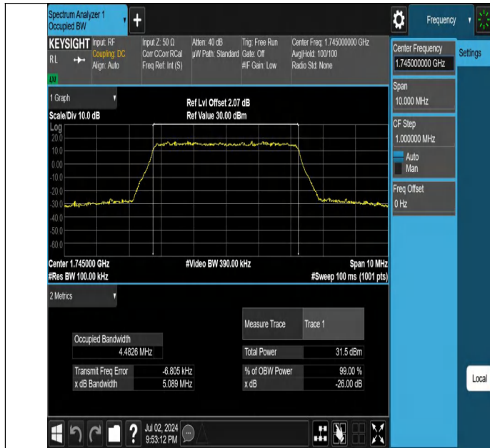
Band66-5MHz-QPSK-132322-25RB#0-PASS
