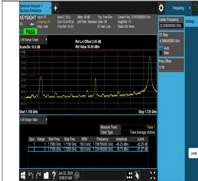
Band66-15MHz-QPSK-132047-1RB#74-PASS
