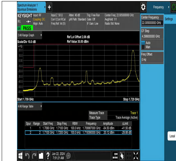
Band66-10MHz-QPSK-132022-1RB#49-PASS
