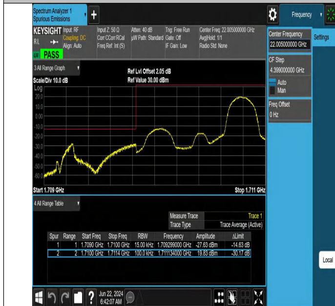
Band66-1.4MHz-QPSK-131979-1RB#5-PASS
