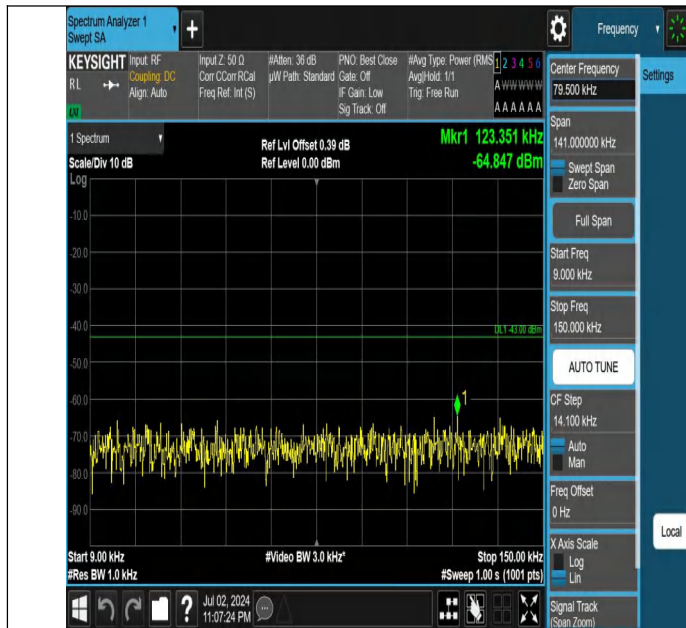
Band66-1.4MHz-QPSK-131979-1RB#0-0.009~0.15-PASS
