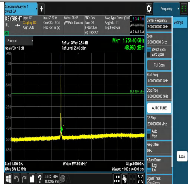
Band66-3MHz-QPSK-132322-1RB#0-1000~3000-PASS
