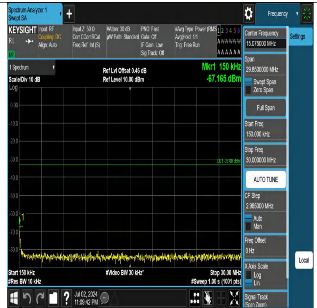
Band66-1.4MHz-QPSK-132665-1RB#0-0.15~30-PASS
