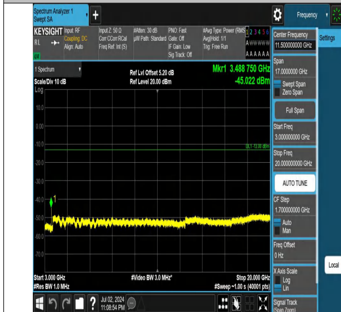
Band66-1.4MHz-QPSK-132322-1RB#0-3000~20000-PASS
