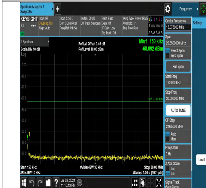
Band66-1.4MHz-QPSK-132665-1RB#5-0.15~30-PASS
