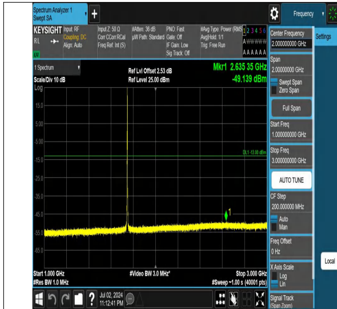
Band66-3MHz-QPSK-132322-1RB#14-1000~3000-PASS
