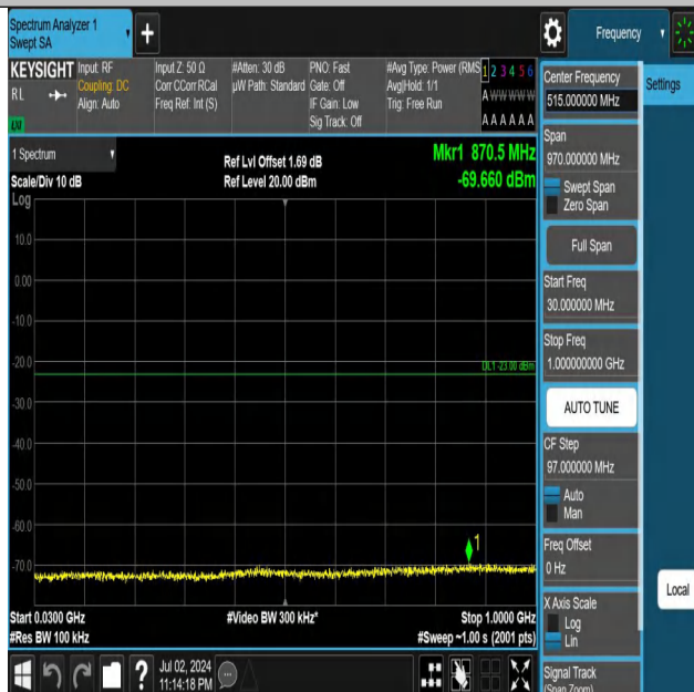
Band66-5MHz-QPSK-131997-1RB#0-30~1000-PASS
