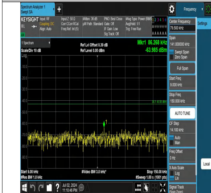
Band66-3MHz-QPSK-131987-1RB#0-0.009~0.15-PASS
