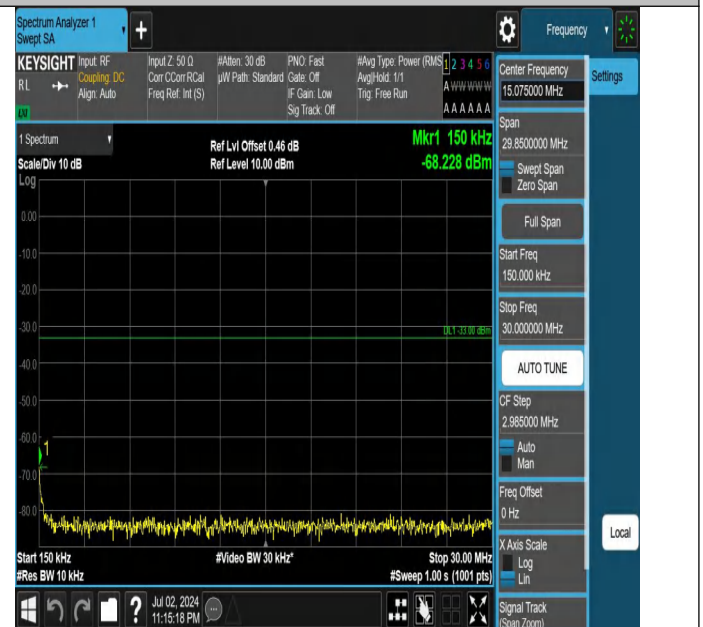
Band66-5MHz-QPSK-132322-1RB#0-0.15~30-PASS
