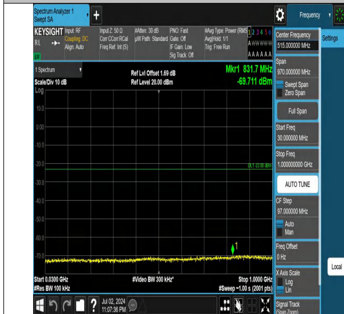
Band66-1.4MHz-QPSK-131979-1RB#0-30~1000-PASS
