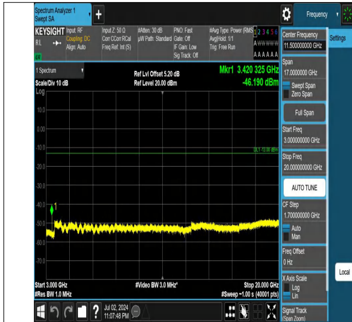
Band66-1.4MHz-QPSK-131979-1RB#0-3000~20000-PASS
