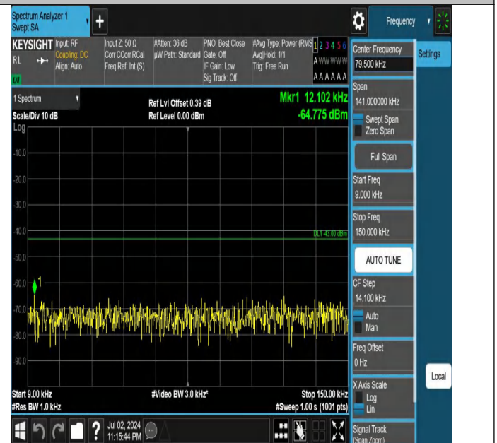
Band66-5MHz-QPSK-132322-1RB#24-0.009~0.15-PASS
