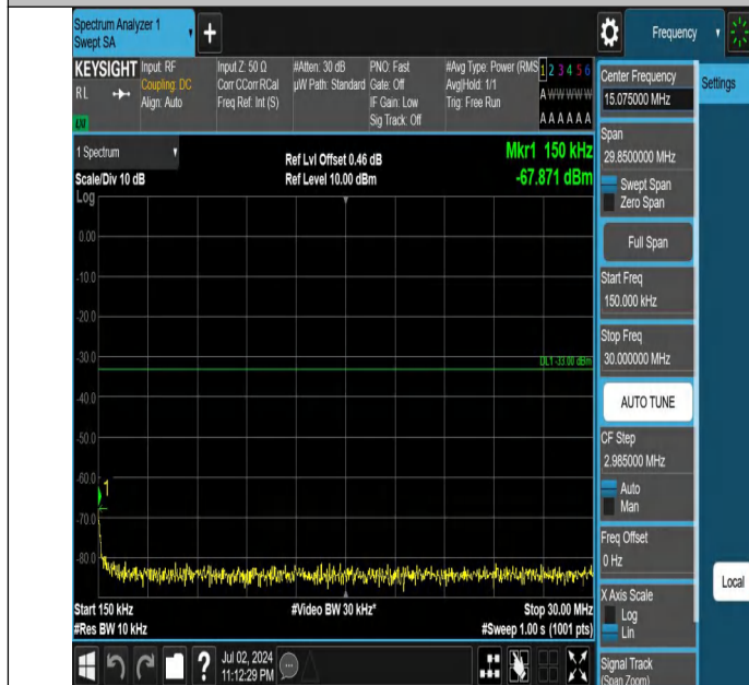
Band66-3MHz-QPSK-132322-1RB#14-0.15~30-PASS
