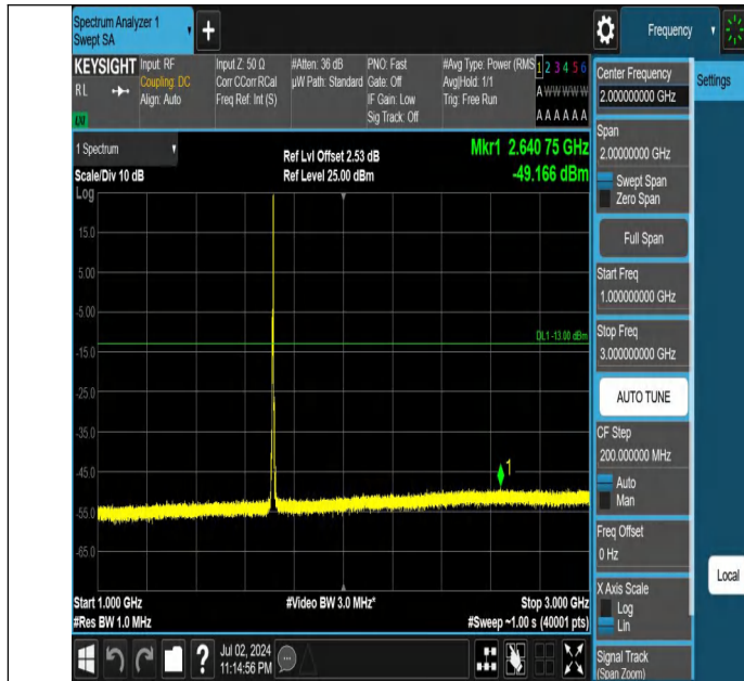
Band66-5MHz-QPSK-131997-1RB#24-1000~3000-PASS
