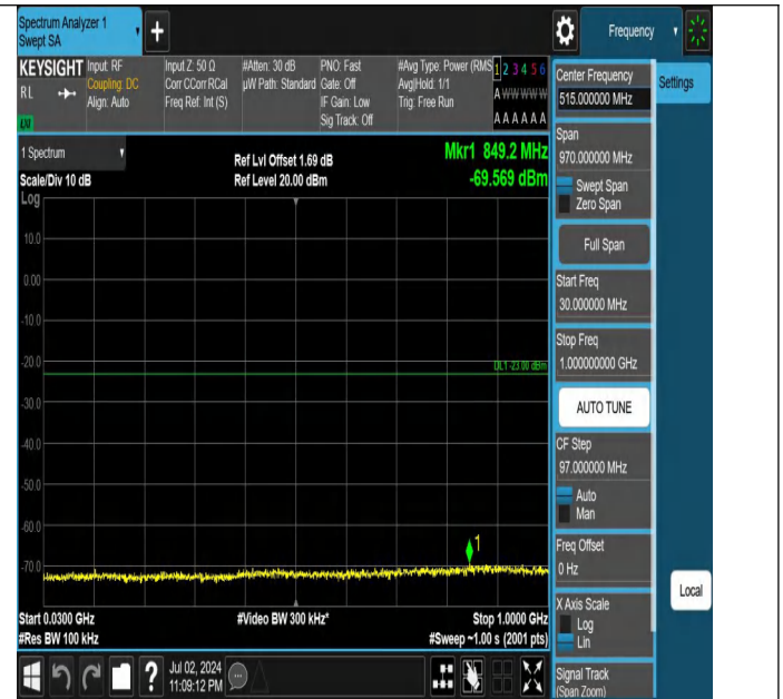
Band66-1.4MHz-QPSK-132322-1RB#5-30~1000-PASS
