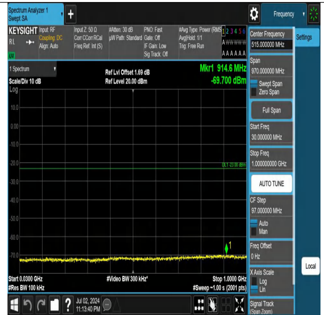
Band66-3MHz-QPSK-132657-1RB#14-30~1000-PASS
