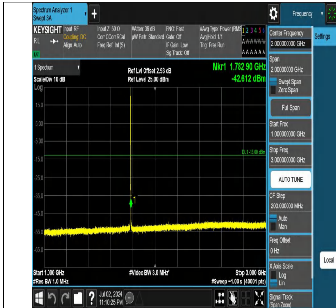
Band66-1.4MHz-QPSK-132665-1RB#5-1000~3000-PASS
