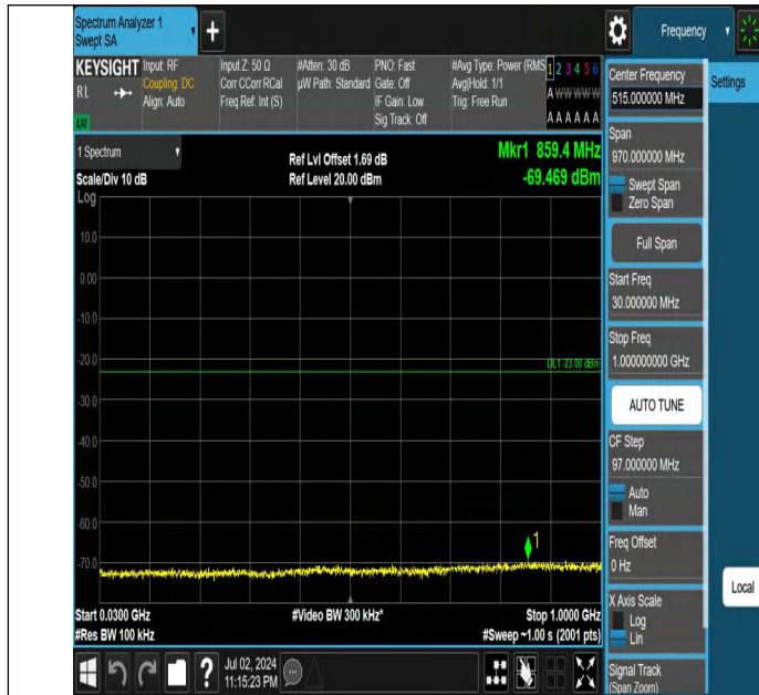
Band66-5MHz-QPSK-132322-1RB#0-30~1000-PASS
