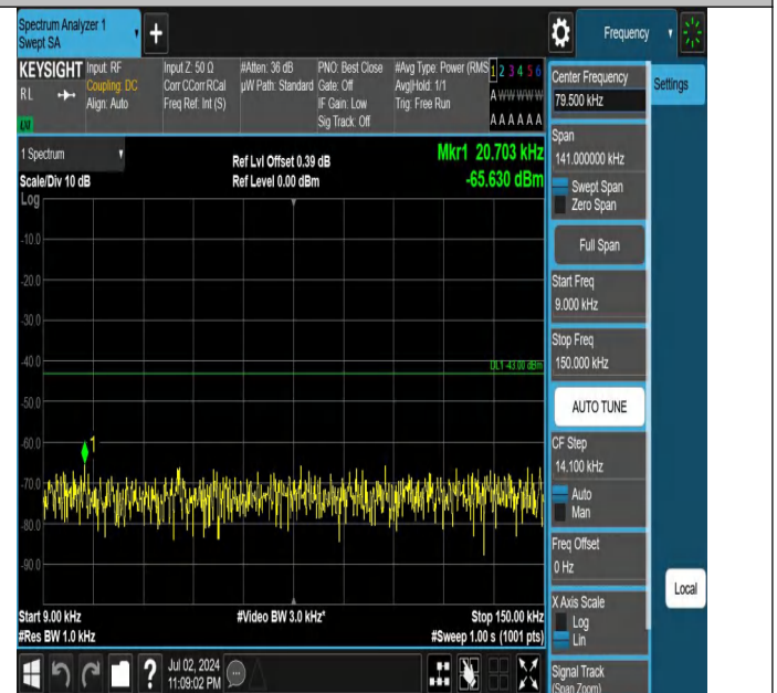
Band66-1.4MHz-QPSK-132322-1RB#5-0.009~0.15-PASS
