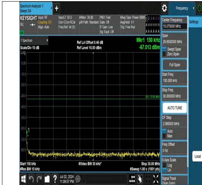
Band66-1.4MHz-QPSK-132322-1RB#5-0.15~30-PASS
