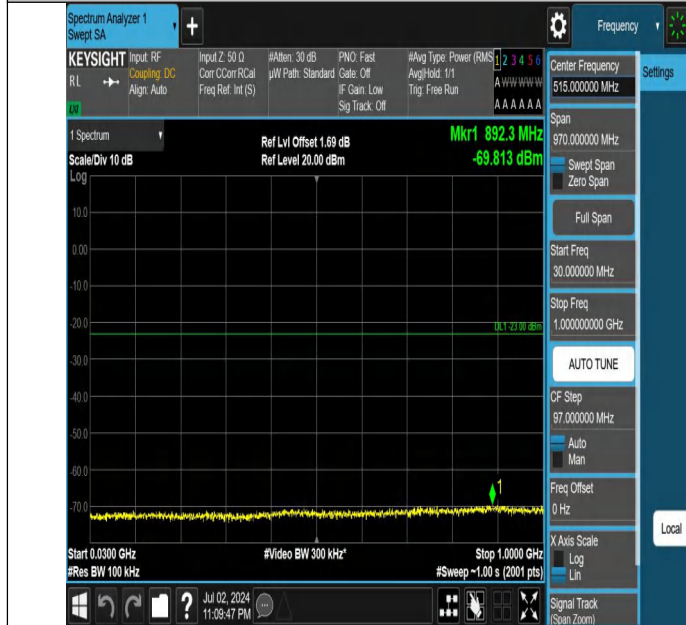
Band66-1.4MHz-QPSK-132665-1RB#0-30~1000-PASS
