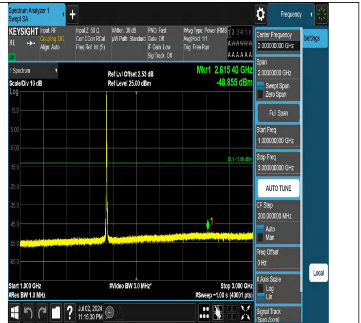
Band66-5MHz-QPSK-132322-1RB#0-1000~3000-PASS
