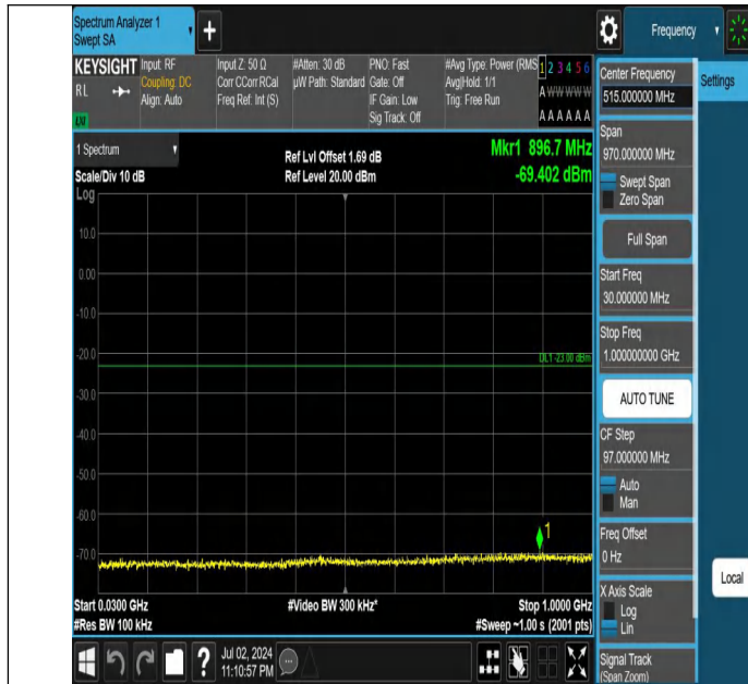
Band66-3MHz-QPSK-131987-1RB#0-30~1000-PASS
