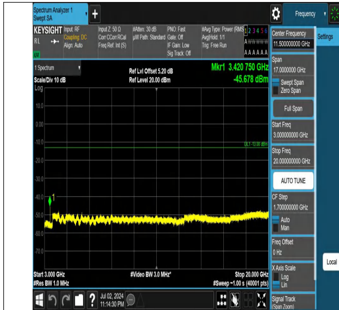
Band66-5MHz-QPSK-131997-1RB#0-3000~20000-PASS
