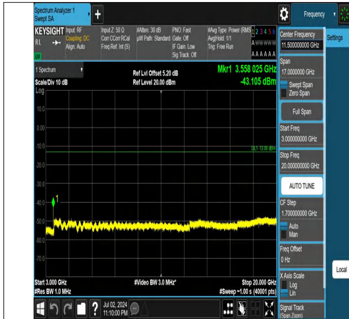
Band66-1.4MHz-QPSK-132665-1RB#0-3000~20000-PASS
