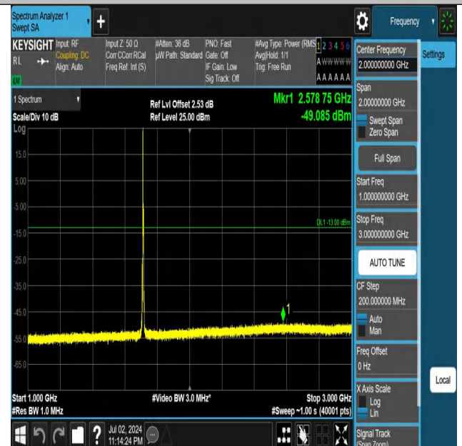
Band66-5MHz-QPSK-131997-1RB#0-1000~3000-PASS
