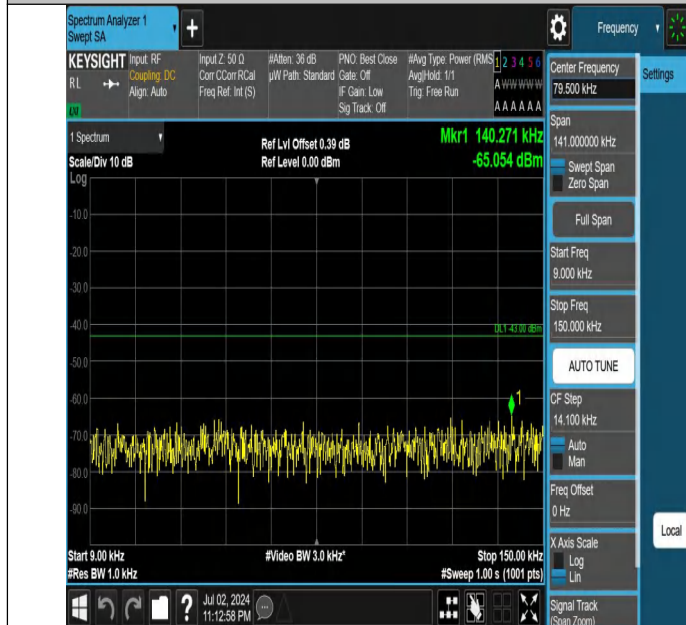
Band66-3MHz-QPSK-132657-1RB#0-0.009~0.15-PASS
