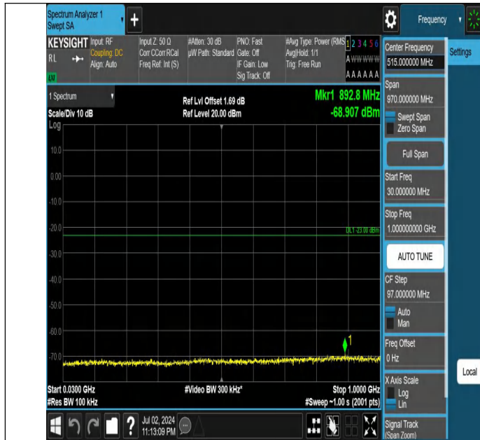
Band66-3MHz-QPSK-132657-1RB#0-30~1000-PASS
