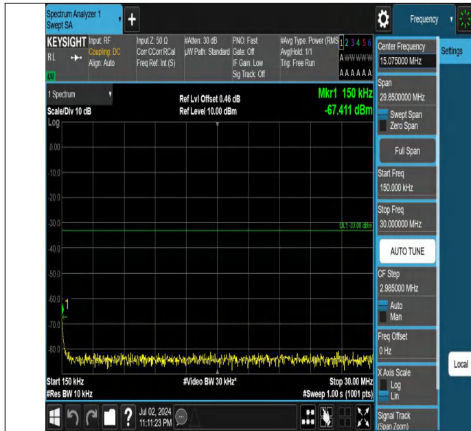
Band66-3MHz-QPSK-131987-1RB#14-0.15~30-PASS
