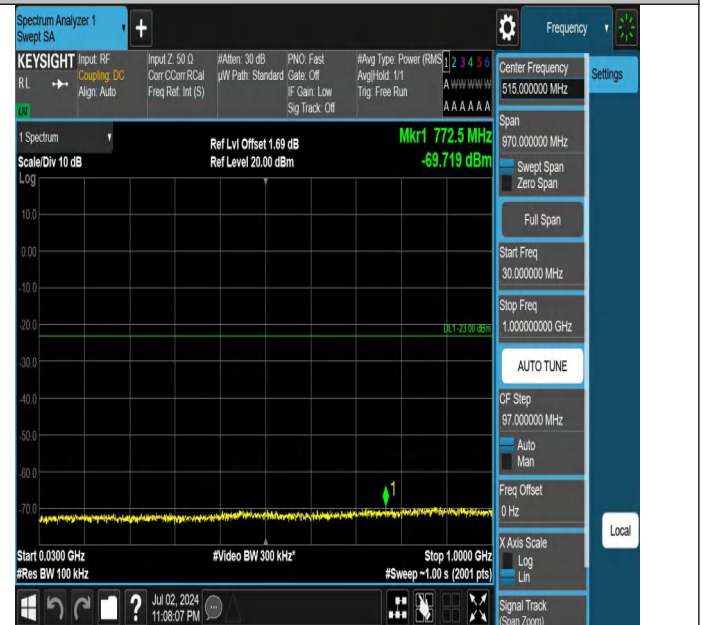
Band66-1.4MHz-QPSK-131979-1RB#5-30~1000-PASS
