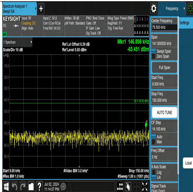
Band66-5MHz-QPSK-131997-1RB#0-0.009~0.15-PASS
