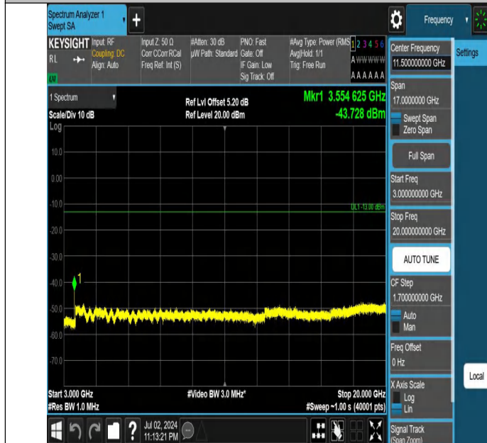
Band66-3MHz-QPSK-132657-1RB#0-3000~20000-PASS
