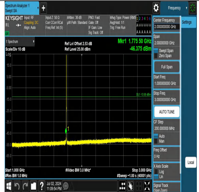
Band66-1.4MHz-QPSK-132665-1RB#0-1000~3000-PASS
