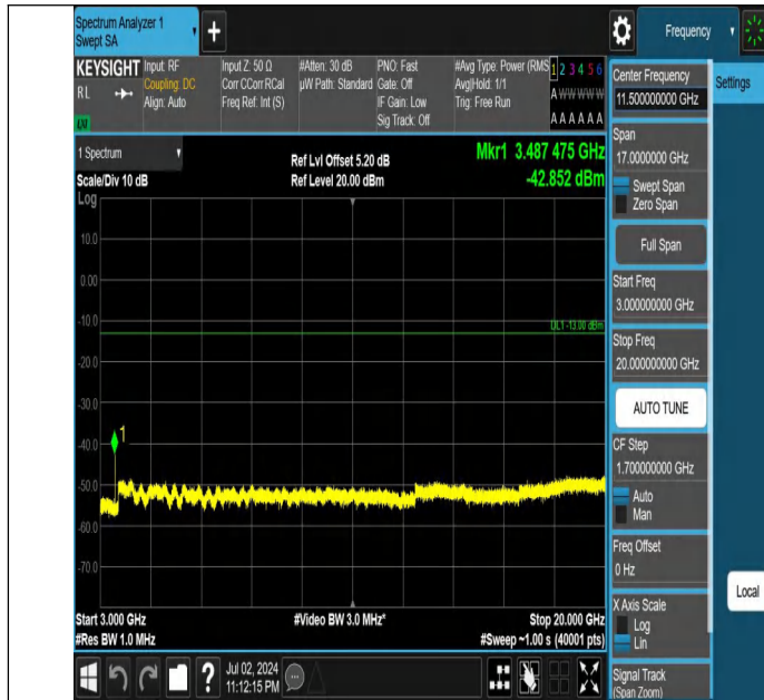
Band66-3MHz-QPSK-132322-1RB#0-3000~20000-PASS
