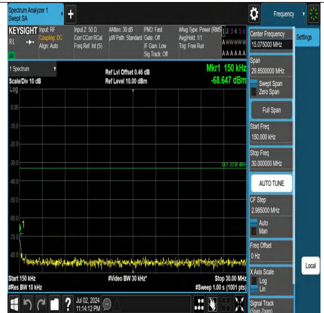
Band66-5MHz-QPSK-131997-1RB#0-0.15~30-PASS
