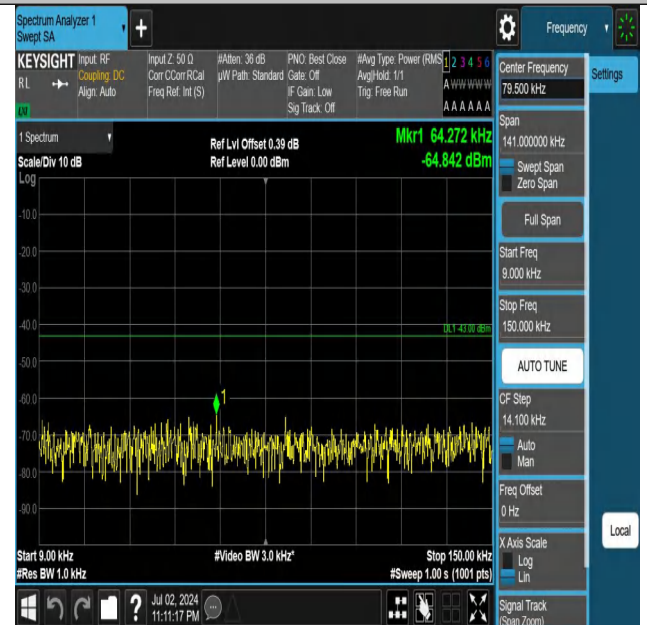
Band66-3MHz-QPSK-131987-1RB#14-0.009~0.15-PASS
