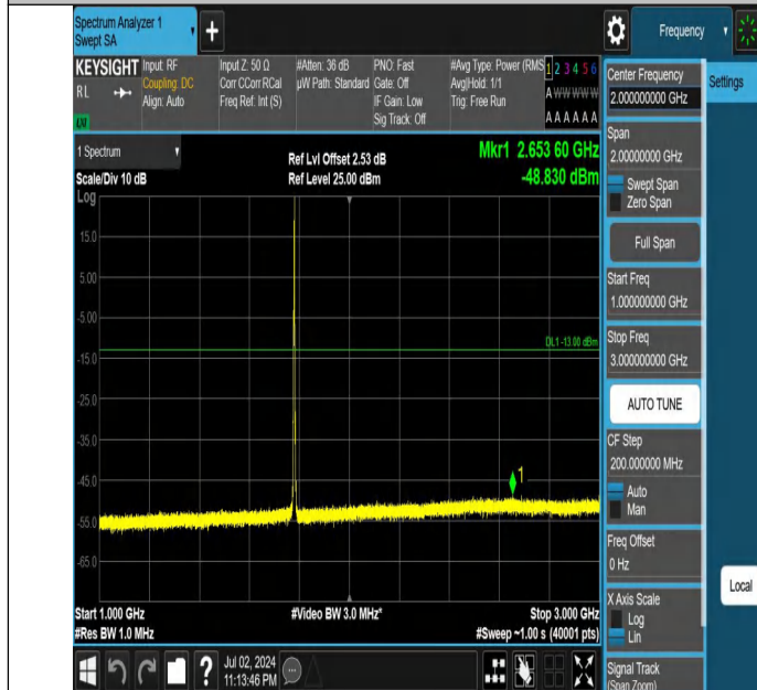
Band66-3MHz-QPSK-132657-1RB#14-1000~3000-PASS
