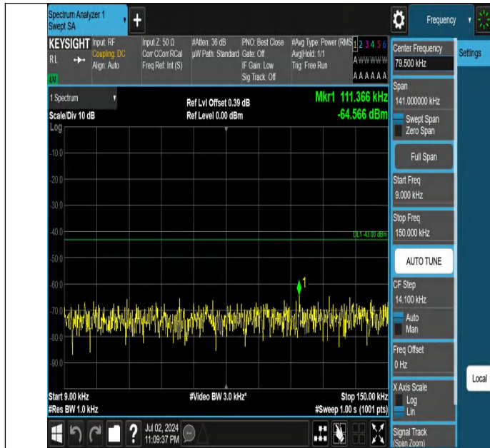
Band66-1.4MHz-QPSK-132665-1RB#0-0.009~0.15-PASS
