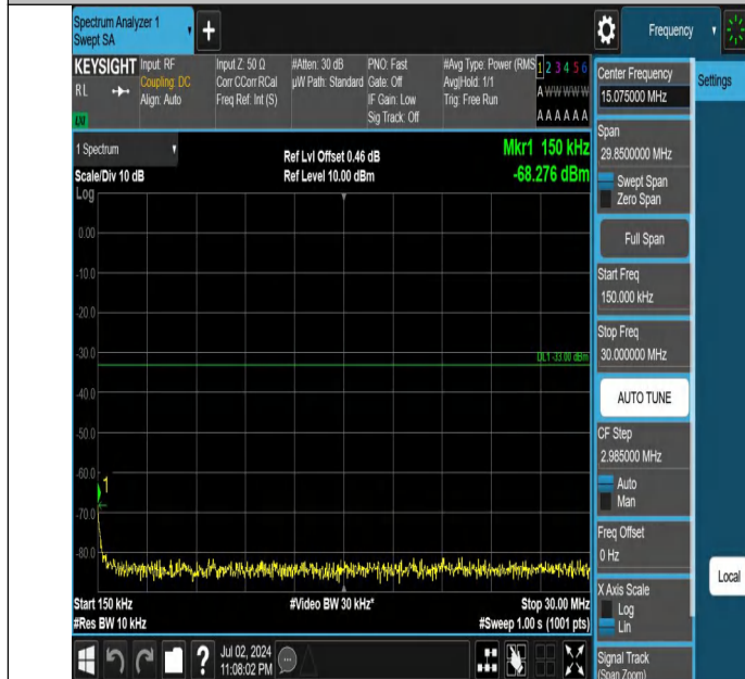
Band66-1.4MHz-QPSK-131979-1RB#5-0.15~30-PASS
