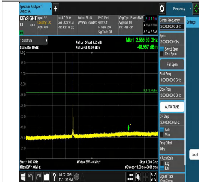
Band66-3MHz-QPSK-131987-1RB#14-1000~3000-PASS
