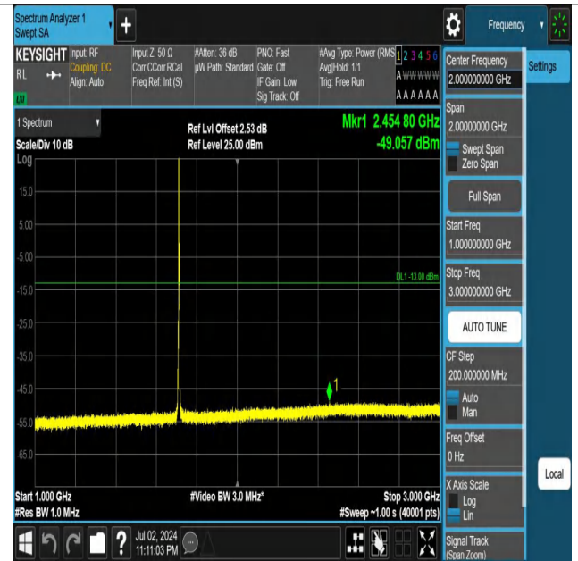
Band66-3MHz-QPSK-131987-1RB#0-1000~3000-PASS
