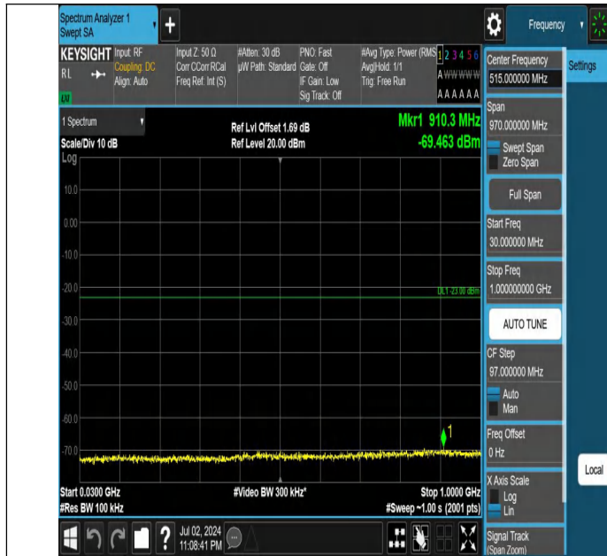
Band66-1.4MHz-QPSK-132322-1RB#0-30~1000-PASS
