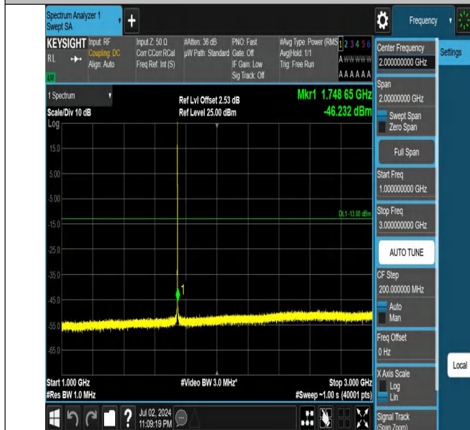
Band66-1.4MHz-QPSK-132322-1RB#5-1000~3000-PASS
