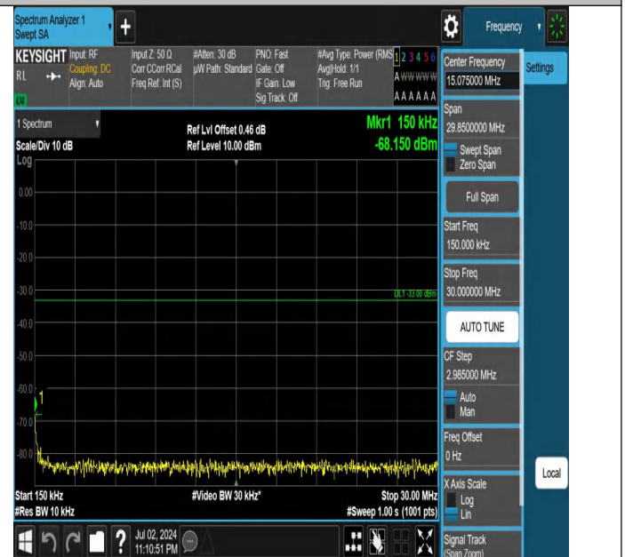
Band66-3MHz-QPSK-131987-1RB#0-0.15~30-PASS
