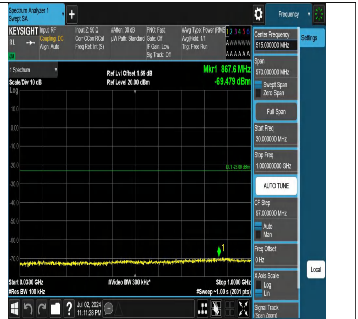
Band66-3MHz-QPSK-131987-1RB#14-30~1000-PASS
