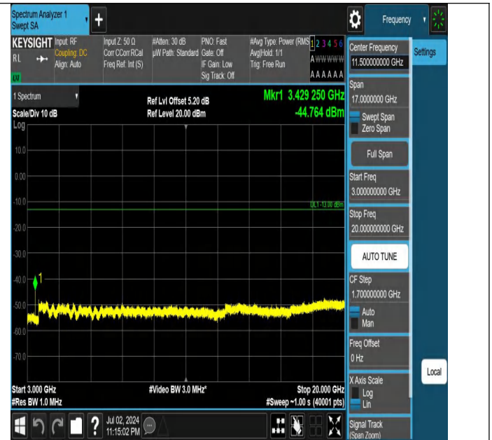
Band66-5MHz-QPSK-131997-1RB#24-3000~20000-PASS
