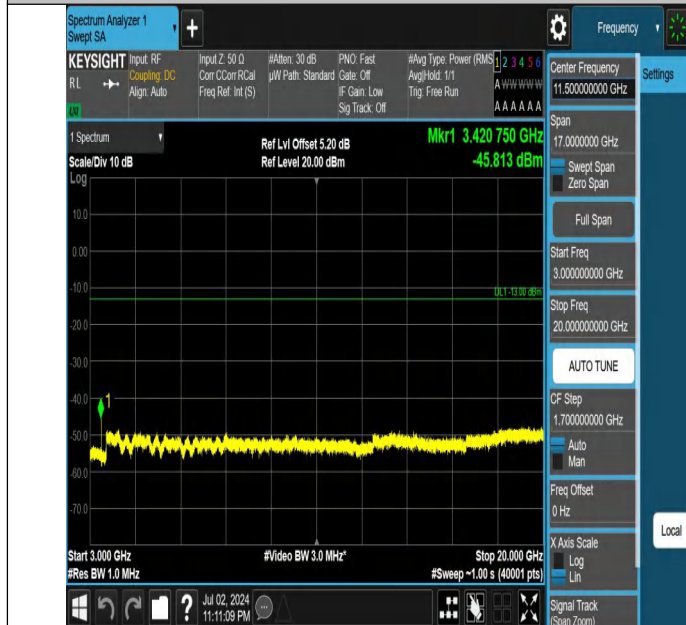
Band66-3MHz-QPSK-131987-1RB#0-3000~20000-PASS
