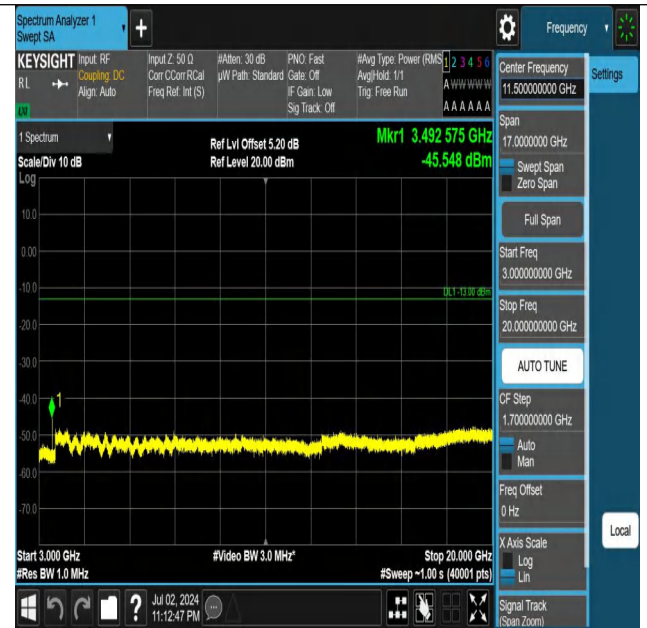
Band66-3MHz-QPSK-132322-1RB#14-3000~20000-PASS
