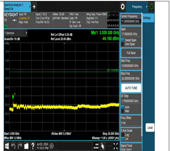
Band66-1.4MHz-QPSK-132665-1RB#5-3000~20000-PASS
