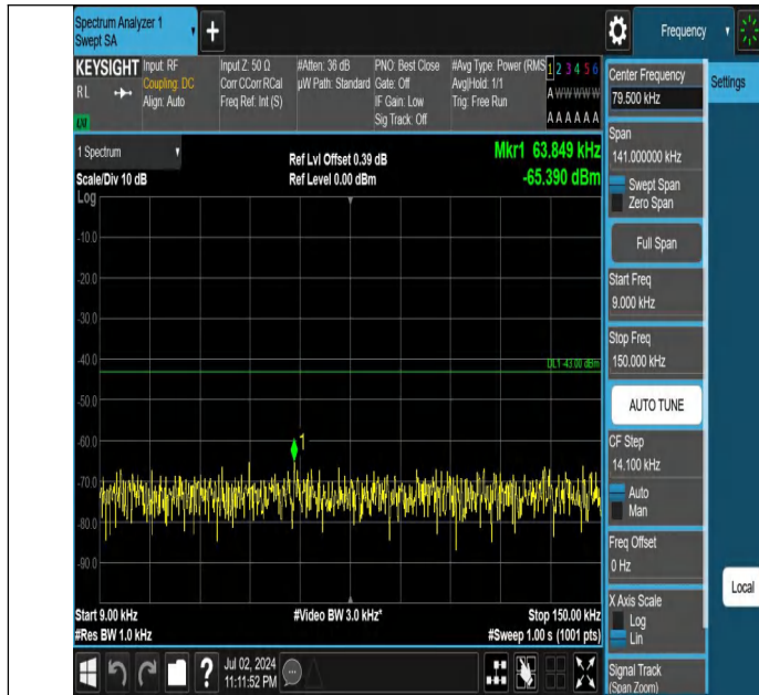
Band66-3MHz-QPSK-132322-1RB#0-0.009~0.15-PASS
