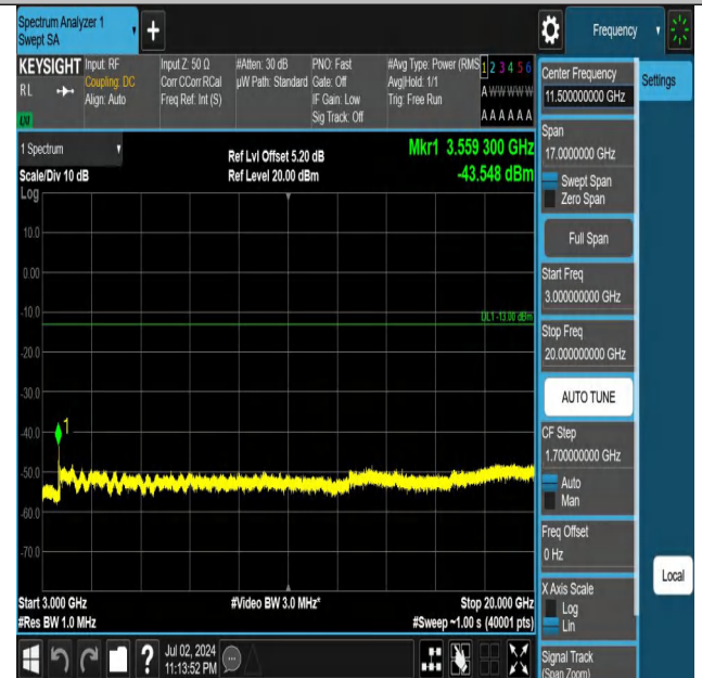
Band66-3MHz-QPSK-132657-1RB#14-3000~20000-PASS
