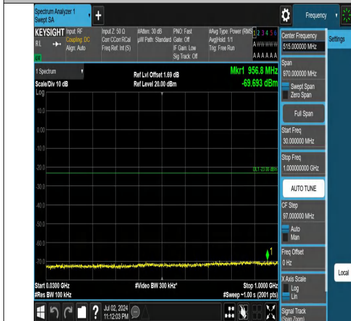
Band66-3MHz-QPSK-132322-1RB#0-30~1000-PASS
