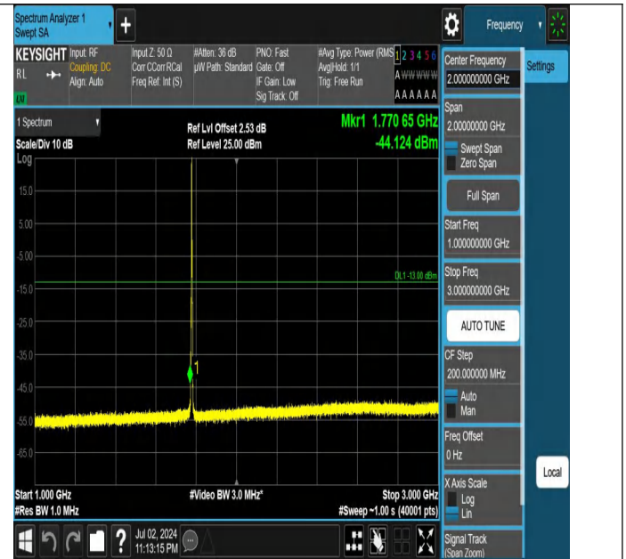
Band66-3MHz-QPSK-132657-1RB#0-1000~3000-PASS
