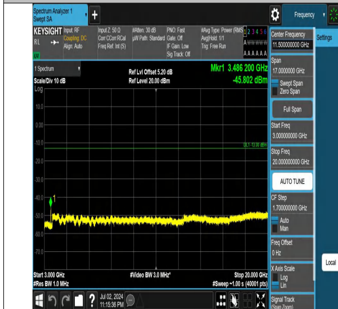
Band66-5MHz-QPSK-132322-1RB#0-3000~20000-PASS
