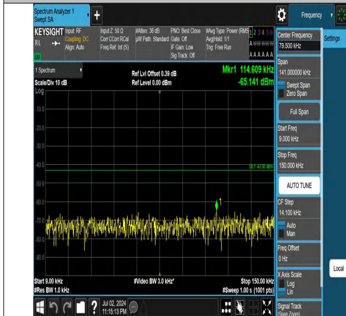
Band66-5MHz-QPSK-132322-1RB#0-0.009~0.15-PASS
