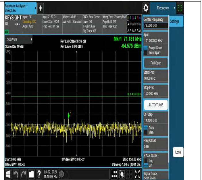
Band66-1.4MHz-QPSK-132665-1RB#5-0.009~0.15-PASS
