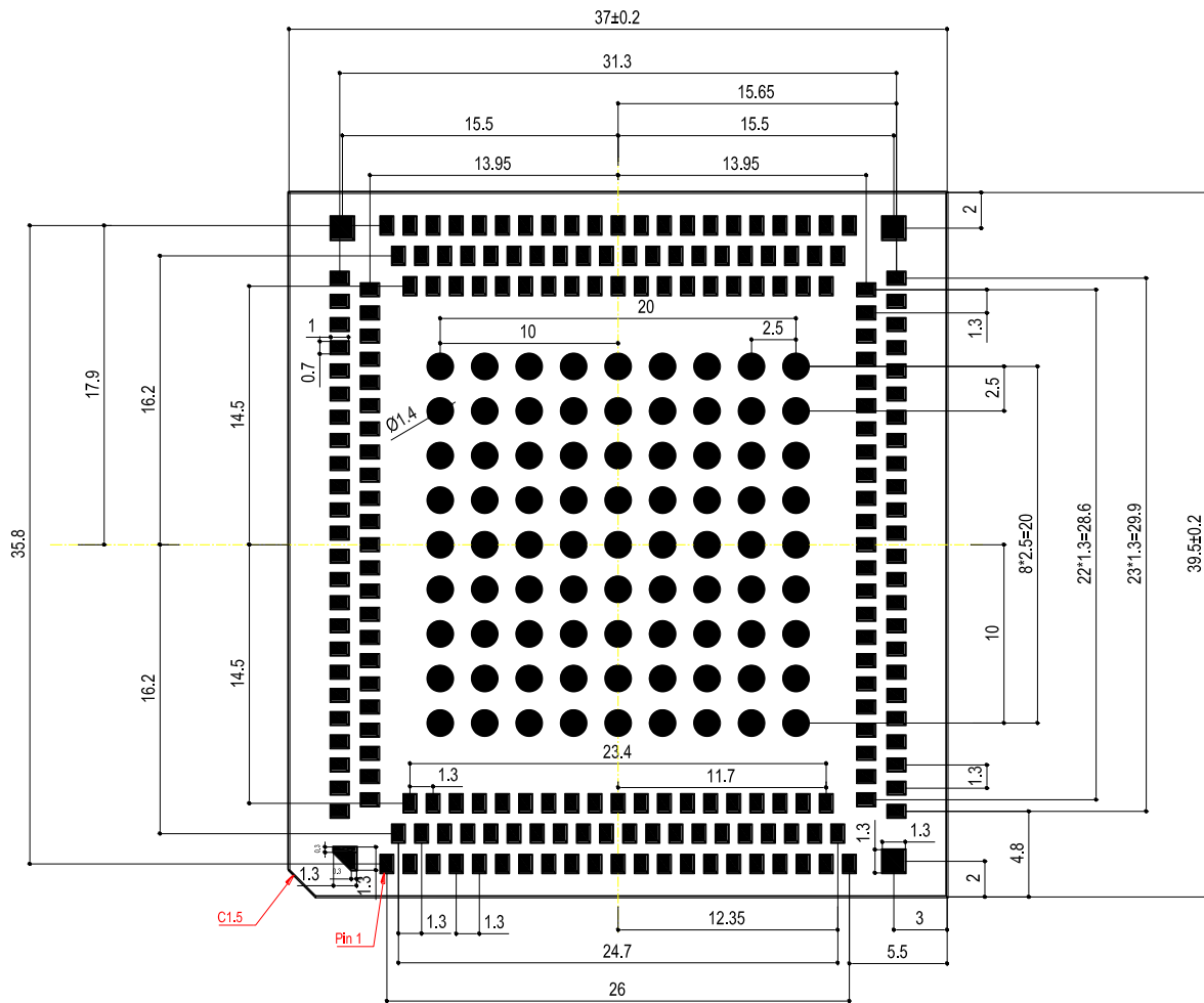
Figure 44: Recommended Footprint
