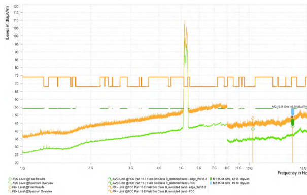
Wi-Fi 5G-11AX20_5240_High
