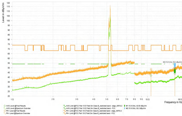
Wi-Fi 5G-11AX20_5500_High
