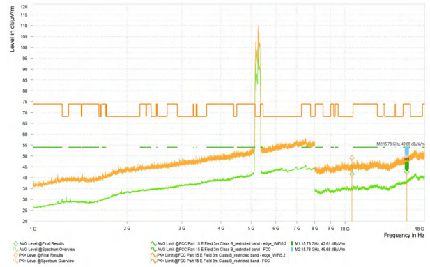
Wi-Fi 5G-11AX20_5320_High
