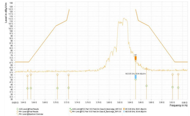
Wi-Fi 5G_11AX20_5825_52Tone_RU40
