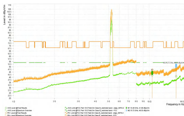
Wi-Fi 5G-11A_5300_High
