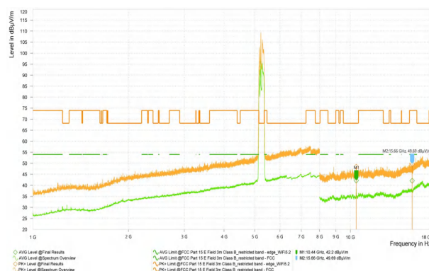
Wi-Fi 5G-11A_5260_High
