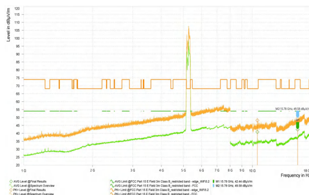
Wi-Fi 5G-11A_5320_High
