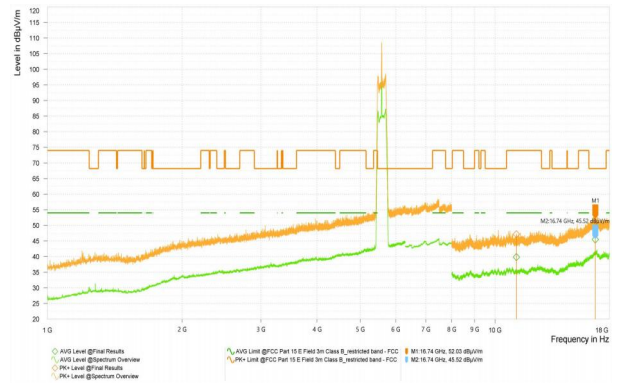
Wi-Fi 5G-11AX20_5720_High
