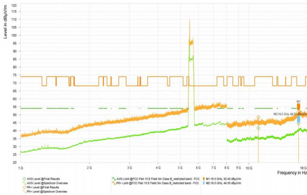
Wi-Fi 5G-11AX20_5700_High
