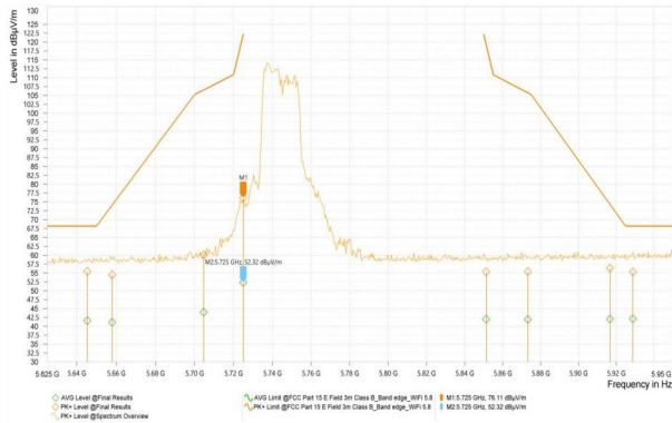
Wi-Fi 5G_11AX20_5745_52Tone_RU37
