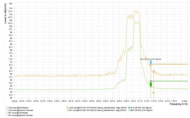
Wi-Fi 5G_11AX20_5700_52Tone_RU40
