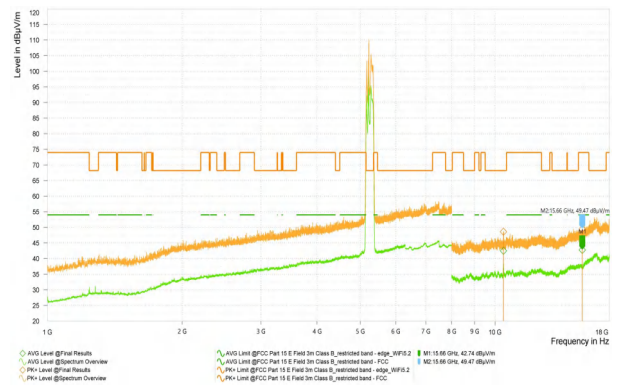
Wi-Fi 5G-11AX20_5260_High
