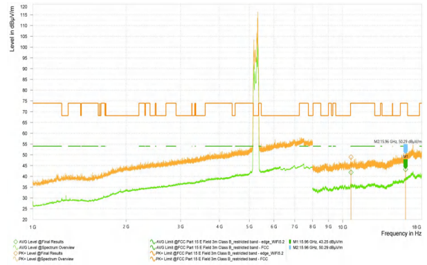
Wi-Fi 5G-11AX20_5580_High
