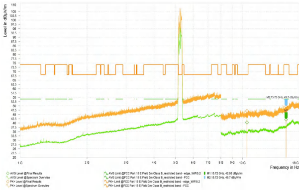
Wi-Fi 5G-11AX20_5300_High
