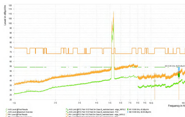
Wi-Fi 5G-11A_5580_High
