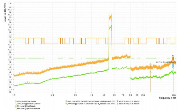
Wi-Fi 5G-11AX20_5220_High
