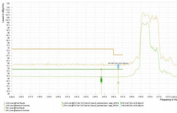
Wi-Fi 5G_11AX20_5500_52Tone_RU37
