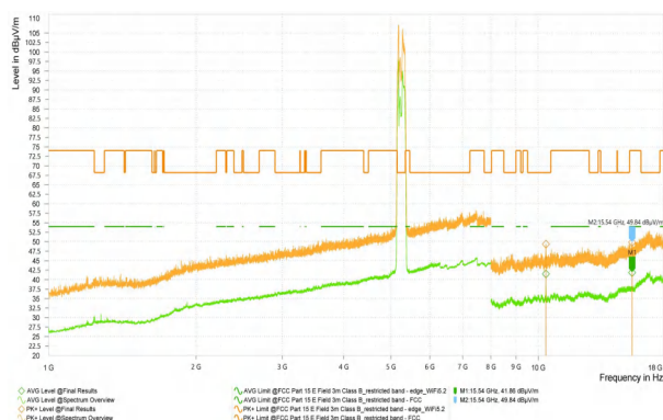
Wi-Fi 5G-11A_5240_High
