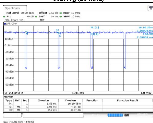
802.11g (20 MHz)
