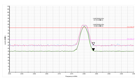
Thread-Channel 26 Peak+ Average
