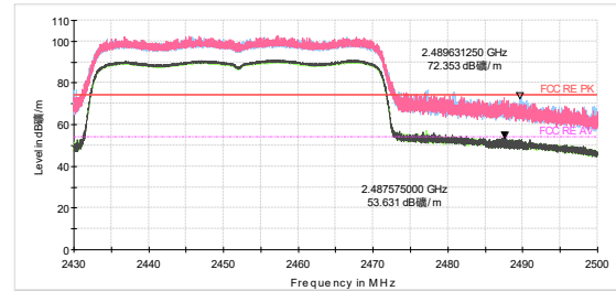
802.11ax HE40-Channel 9 Peak+ Average
