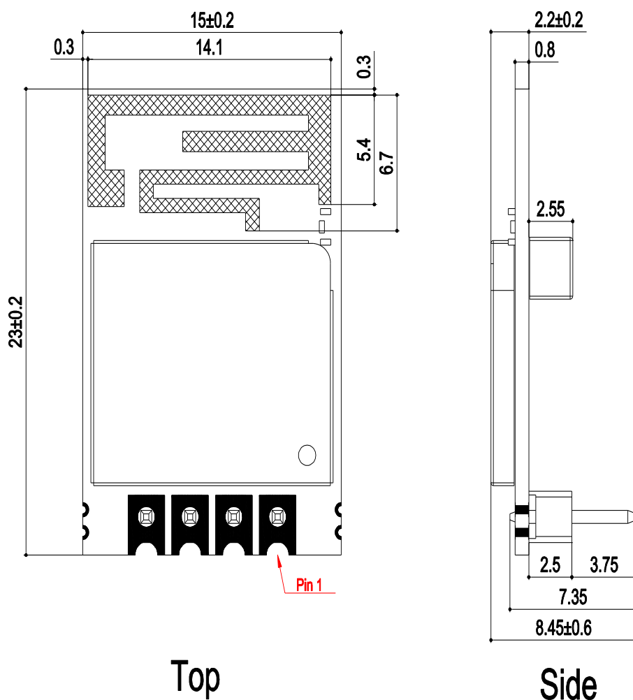
Figure 3: DIP Module Top and Side Dimensions
