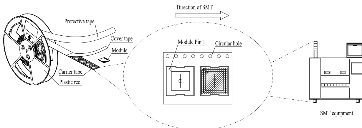
Figure 11: Mounting Direction
