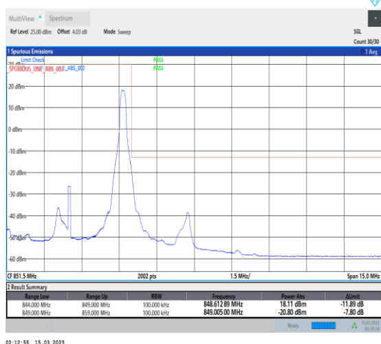
1-N5-PC3-15-5-H-5-CP-QPSK-Edge_1RB_Right-1@2 4-Ant1-1-seegraph-PASS-see graph
