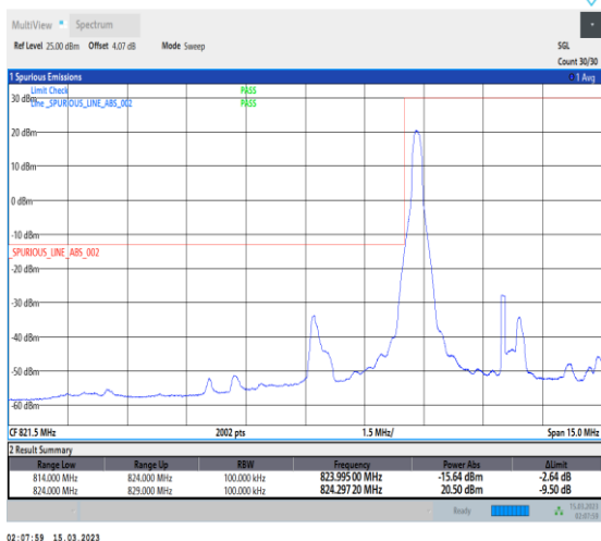
1-N5-PC3-15-5-L-1-DFT-PI2BPSK-Edge_1RB_Left-1 @0-Ant1-1-seegraph-PASS-see graph
