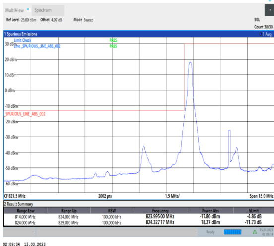
1-N5-PC3-15-5-L-4-CP-QPSK-Edge_1RB_Left-1@0-A nt1-1-seegraph-PASS-see graph
