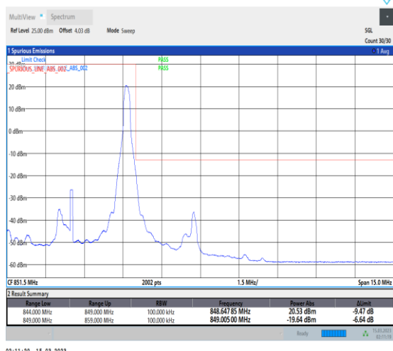
1-N5-PC3-15-5-H-2-DFT-PI2BPSK-Edge_1RB_Right-1 @24-Ant1-1-seegraph-PASS-see graph
