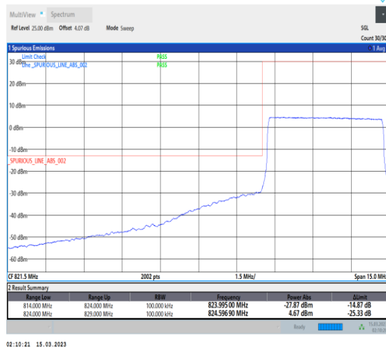
1-N5-PC3-15-5-L-6-CP-QPSK-Outer_Full-25@0-A nt1-1-seegraph-PASS-see graph
