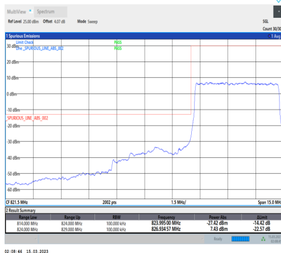
1-N5-PC3-15-5-L-3-DFT-PI2BPSK-Outer_Full-25 @0-Ant1-1-seegraph-PASS-see graph
