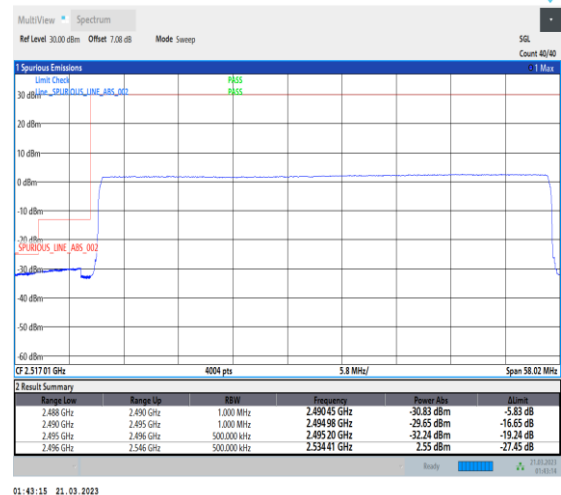
1-N41-30-50-L-6-CP-QPSK-Outer_Full-133@0-Ant1-1--PASS-see graph
