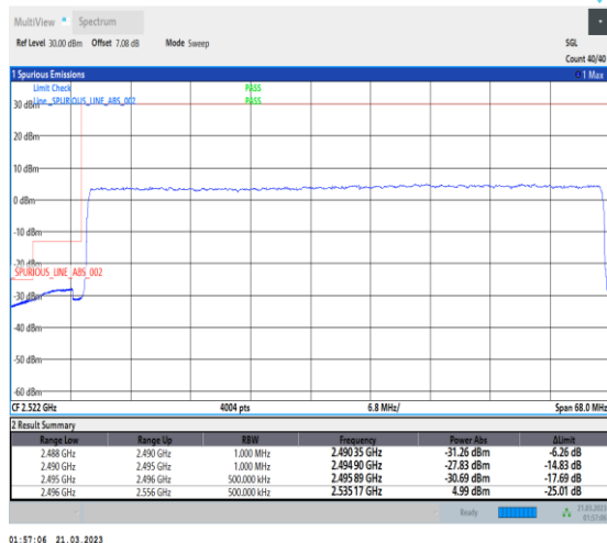
1-N41-30-60-L-3-DFT-PI2BPSK-Outer_Full-162@0-Ant1-1--PASS-see graph
