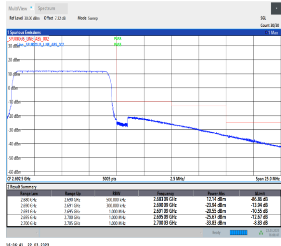
1-N41-30-10-H-6-CP-QPSK-Outer_Full-24@0-Ant1 1-1--PASS-see graph
