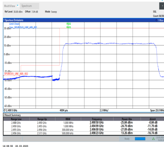
1-N41-30-15-L-6-CP-QPSK-Outer_Full-38@0-Ant1 1-1--PASS-see graph
