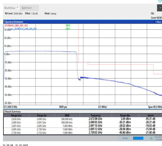
1-N41-30-40-H-6-CP-QPSK-Outer_Full-106@0-Ant1-1--PASS-see graph
