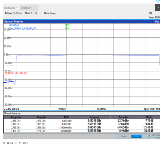
1-N41-30-100-L-6-CP-QPSK-Outer_Full-273@0-Ant1-1--PASS-see graph
