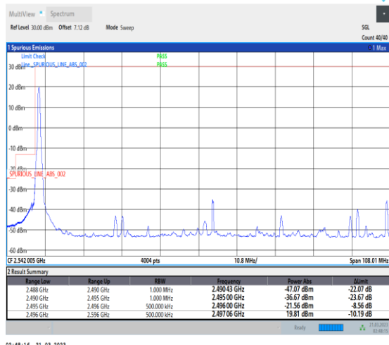
1-N41-30-100-L-1-DFT-PI2BPSK-Edge_1RB_Left-1@0-Ant1-1--PASS-see graph
