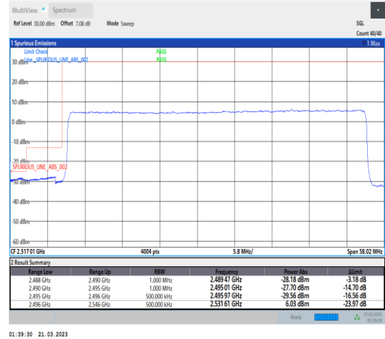
1-N41-30-50-L-3-DFT-PI2BPSK-Outer_Full-128@0-Ant1-1--PASS-see graph
