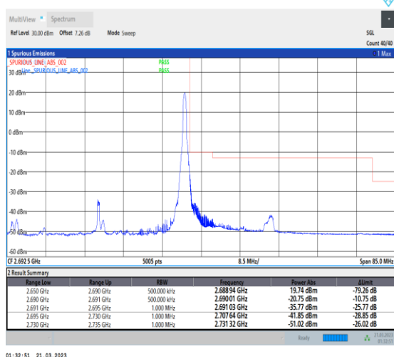
1-N41-30-40-H-5-CP-QPSK-Edge_1RB_Right-1@105-Ant1-1--PASS-see graph
