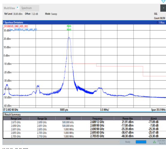
1-N41-30-15-H-5-CP-QPSK-Edge_1RB_Right-1@37-Ant1 1-1--PASS-see graph
