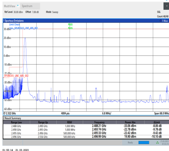
1-N41-30-60-L-1-DFT-PI2BPSK-Edge_1RB_Left-1@0-Ant1-1--PASS-see graph
