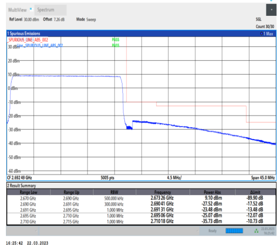
1-N41-30-20-H-6-CP-QPSK-Outer_Full-51@0-Ant1 1-1--PASS-see graph
