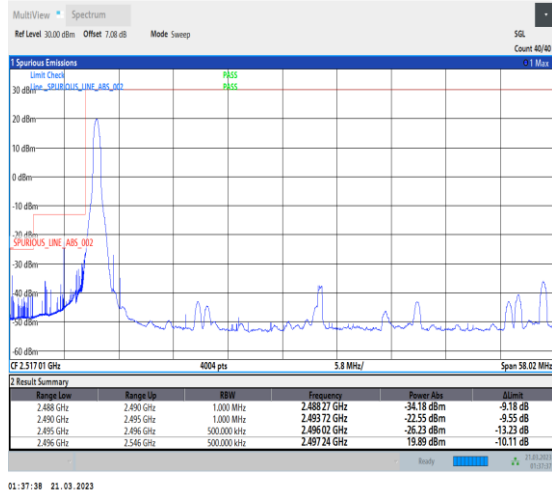
1-N41-30-50-L-1-DFT-PI2BPSK-Edge_1RB_Left-1@0-Ant1-1--PASS-see graph
