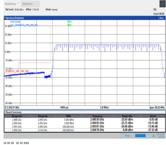
1-N41-30-20-L-6-CP-QPSK-Outer_Full-51@0-Ant1 1-1--PASS-see graph
