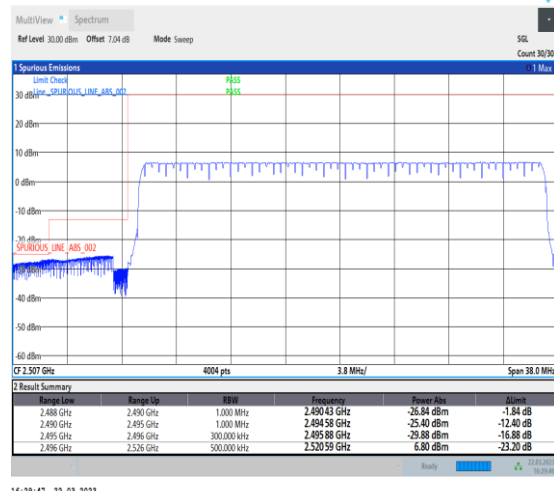
1-N41-30-30-L-6-CP-QPSK-Outer_Full-78@0-Ant1 1-1--PASS-see graph
