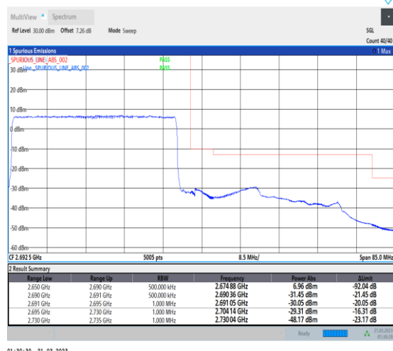
1-N41-30-40-H-3-DFT-PI2BPSK-Outer_Full-100@0-Ant1-1--PASS-see graph
