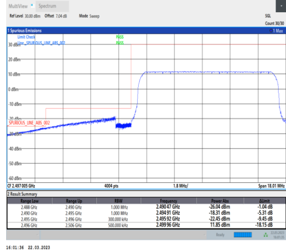
1-N41-30-10-L-6-CP-QPSK-Outer_Full-24@0-Ant1 1-1--PASS-see graph
