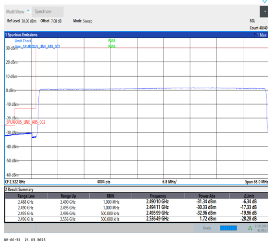
1-N41-30-60-L-6-CP-QPSK-Outer_Full-162@0-Ant1-1--PASS-see graph
