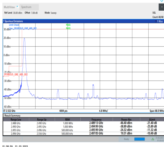
1-N41-30-60-L-4-CP-QPSK-Edge_1RB_Left-1@0-Ant1-1--PASS-see graph
