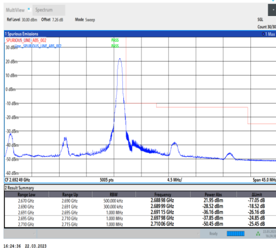
1-N41-30-20-H-5-CP-QPSK-Edge_1RB_Right-1@50-Ant1 1-1--PASS-see graph
