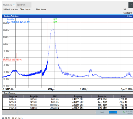
1-N41-30-15-L-4-CP-QPSK-Edge_1RB_Left-1@0-Ant1 -1--PASS-see graph
