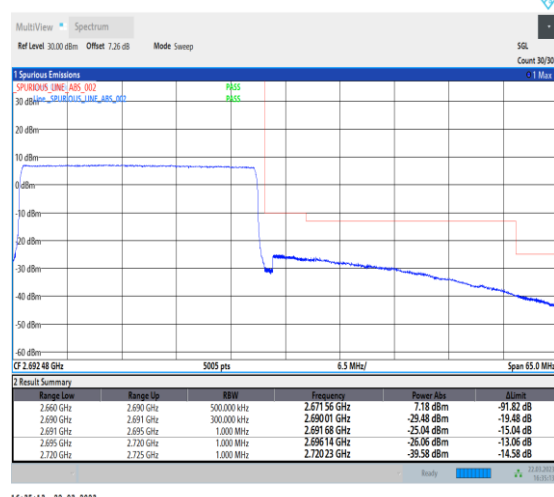
1-N41-30-30-H-6-CP-QPSK-Outer_Full-78@0-Ant1 1-1--PASS-see graph
