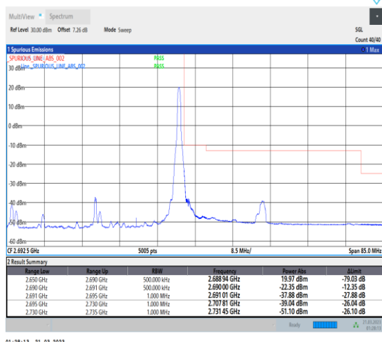
1-N41-30-40-H-2-DFT-PI2BPSK-Edge_1RB_Right-1@105-Ant1-1--PASS-see graph
