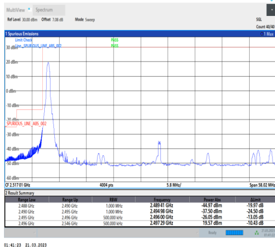
1-N41-30-50-L-4-CP-QPSK-Edge_1RB_Left-1@0-Ant1-1--PASS-see graph
