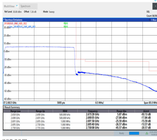
1-N41-30-40-H-6-CP-QPSK-Outer_Full-106@0-Ant1 t1-1--PASS-see graph
