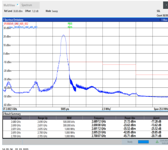
1-N41-30-10-H-5-CP-QPSK-Edge_1RB_Right-1@23-Ant1 nt1-1--PASS-see graph
