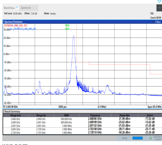
1-N41-30-30-H-5-CP-QPSK-Edge_1RB_Right-1@77-Ant1 nt1-1--PASS-see graph
