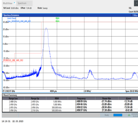
1-N41-30-20-L-4-CP-QPSK-Edge_1RB_Left-1@0-Ant1 -1--PASS-see graph
