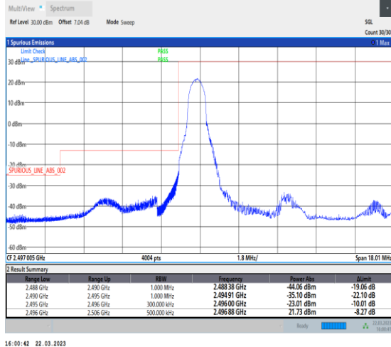
1-N41-30-10-L-4-CP-QPSK-Edge_1RB_Left-1@0-Ant1 -1--PASS-see graph
