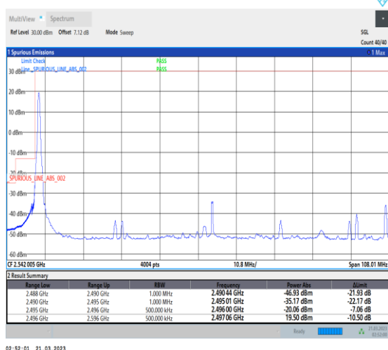
1-N41-30-100-L-4-CP-QPSK-Edge_1RB_Left-1@0-Ant1-1--PASS-see graph
