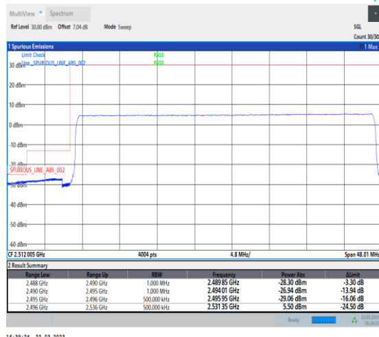
1-N41-30-40-L-6-CP-QPSK-Outer_Full-106@0-Ant1 t1-1--PASS-see graph
