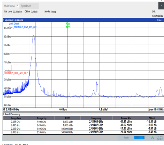
1-N41-30-40-L-4-CP-QPSK-Edge_1RB_Left-1@0-Ant1 -1--PASS-see graph
