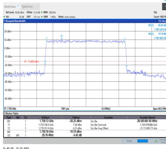
1-N66-PC3-15-30-H-7-CP-16QAM-Outer_Full-160@ 0-Ant1-28.545-29.760-≤30-PASS
