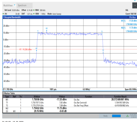
1-N66-PC3-15-30-H-4-DFT-64QAM-Outer_Full-160 @0-Ant1-28.573-29.760-≤30-PASS
