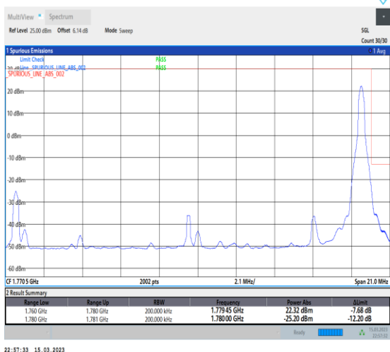
1-N66-PC3-15-20-H-2-DFT-PI2BPSK-Edge_1RB_Right-1@105-Ant1-1-seegraph-PASS-see graph
