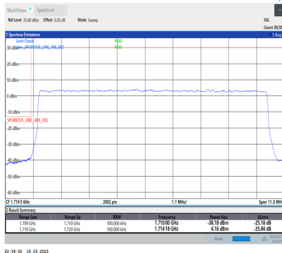
1-N66-PC3-15-10-L-3-DFT-PI2BPSK-Outer_Full-50@0-Ant1-1-seegraph-PASS-see graph
