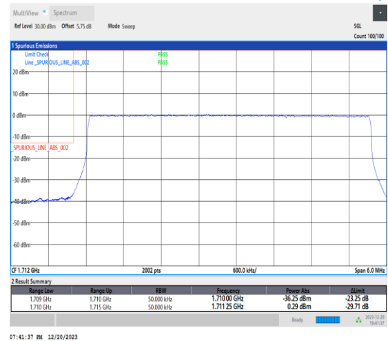
1-N66-15-5-L-6-CP-QPSK-Outer_Full-25@0-Ant1- 1-seegraph-PASS-see graph
