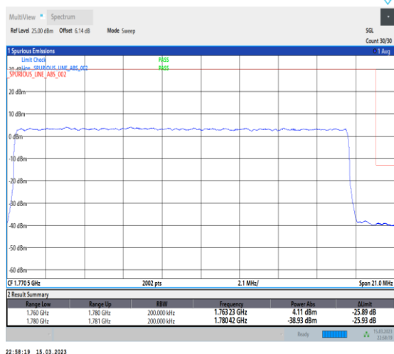
1-N66-PC3-15-20-H-3-DFT-PI2BPSK-Outer_Full-100@0-Ant1-1-seegraph-PASS-see graph
