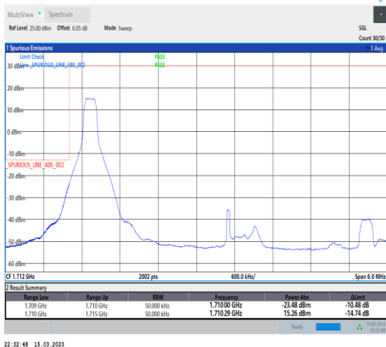
1-N66-PC3-15-5-L-4-CP-QPSK-Edge_1RB_Left-1@0- Ant1-1-seegraph-PASS-see graph
