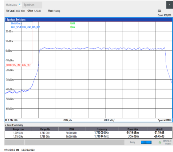
1-N66-15-5-L-3-DFT-PI2BPSK-Outer_Full-25@0- Ant1-1-seegraph-PASS-see graph
