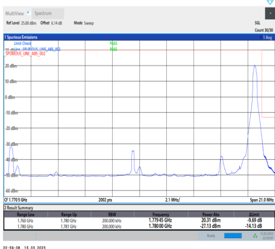
1-N66-PC3-15-20-H-5-CP-QPSK-Edge_1RB_Right-1@105-Ant1-1-seegraph-PASS-see graph
