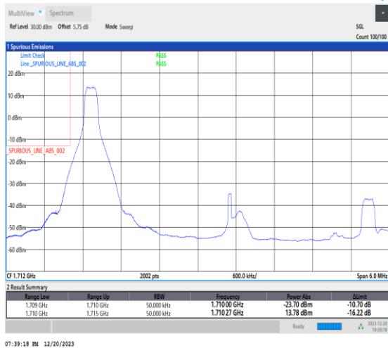
1-N66-15-5-L-4-CP-QPSK-Edge_1RB_Left-1@0-Ant1- 1-seegraph-PASS-see graph
