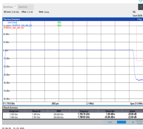
1-N66-PC3-15-20-H-6-CP-QPSK-Outer_Full-106@0-Ant1-1-seegraph-PASS-see graph
