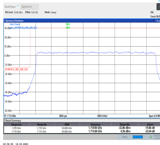
1-N66-PC3-15-5-L-3-DFT-PI2BPSK-Outer_Full-25 @0-Ant1-1-seegraph-PASS-see graph
