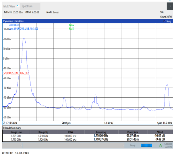
1-N66-PC3-15-10-L-1-DFT-PI2BPSK-Edge_1RB_Left-1@0-Ant1-1-seegraph-PASS-see graph
