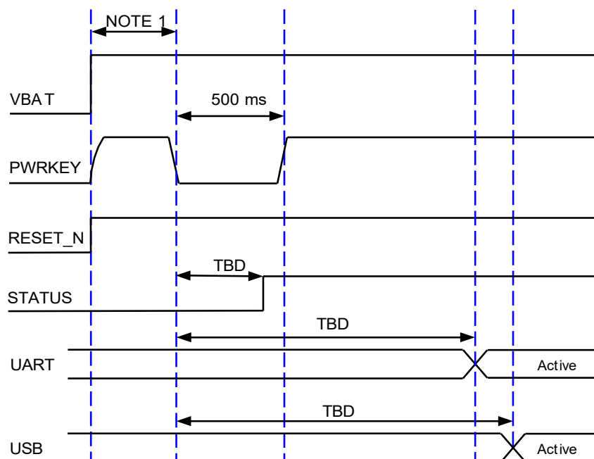
Figure 9: Timing of Turn On with PWRKEY
