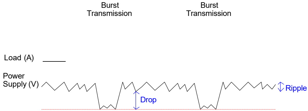
Figure 5: Power Supply Limits During Burst Transmission
