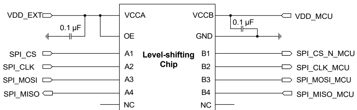
Figure 29: Reference Design of SPI with a Level-Shifting Chip
