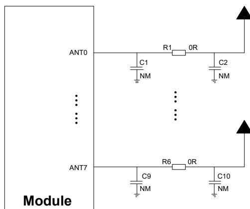
Figure 37: Reference Design of Cellular Antennas
