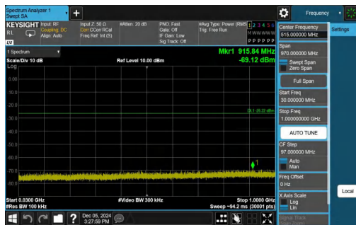
11N40SISO-Ant1-2437-30~1000-PASS
