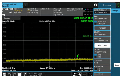
11N20SISO-Ant1-2462-30~1000-PASS
