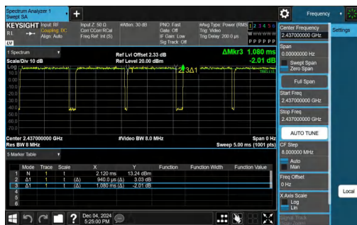
NTNV-11N40SISO-Ant1-2437
